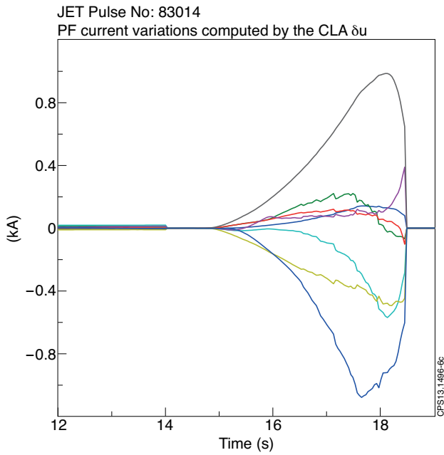
Figure 6: Outputs of the CLA. This plot shows the PF current variations u computed by the CLA and added to the XSC outputs.
