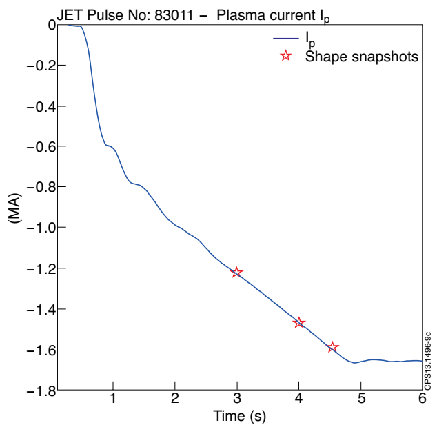
Figure 9: JET Pulse No: 83011, plasma current. The red markers show the time instants where the plasma snapshots shown in Figs. 12 and 13 have been taken.
