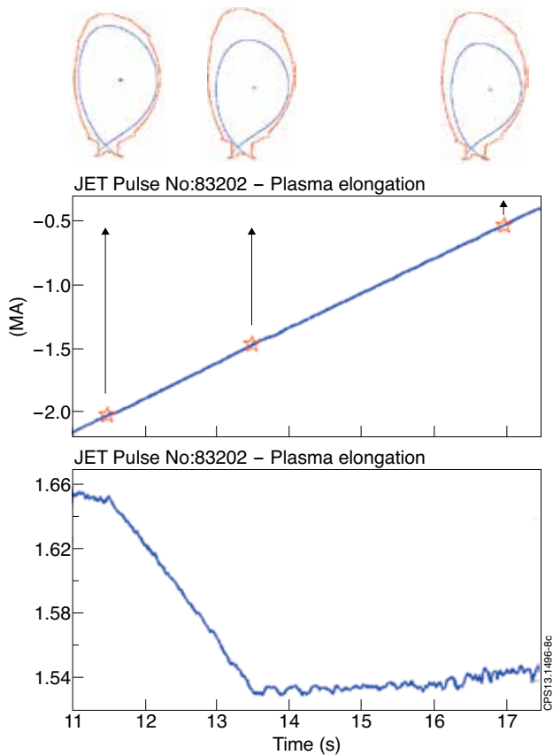
Figure 8: Change of the plasma elongation during the ramp-down (JET Pulse No: 83202). The elongation changes from 11 1:66 to 11 1:54, while the plasma current is ramping down.
