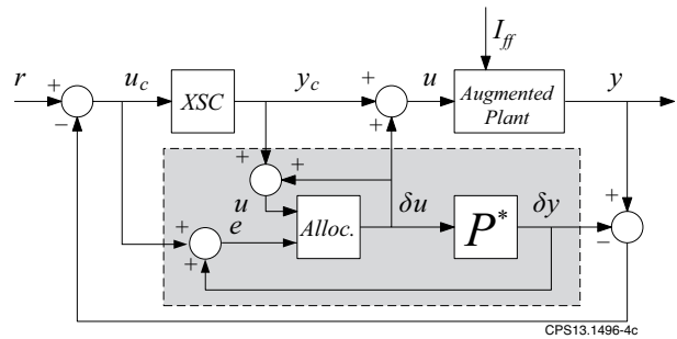
Figure 4: Block diagram of the allocated closed-loop. The Current Limit Avoidance is the grey shaded box, which includes the Allocator dynamical system, and takes both the controller input and output signals as an input.
