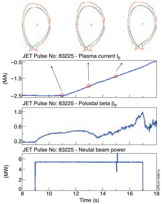
Figure 7: Shape control with the XSC during the the L-H transition at the ramp-down (JET Pulse No: 83225). In this figure the plasma shape is shown at different time instants during the ramp-down (the shape reference is the blue curve, while the green curve is the actual shape). The experimental values of the poloidal beta p and of the neutral beam injected power are also shown.
