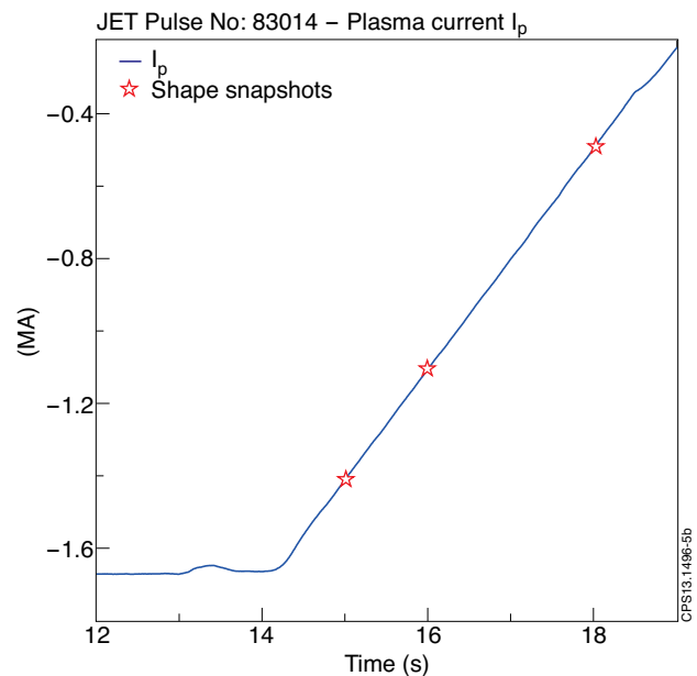
Figure 5: Plasma current during the ramp-down of the JET Pulse No's: 72203 and 83014. The red markers show the time instants where the plasma snapshots shown in Figs. 10 and 11 have been taken.
