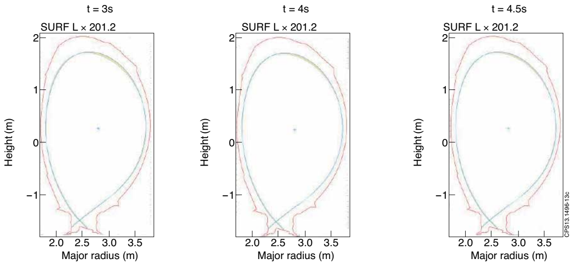
Figure 13: Shape tracking with the JET standard Shape Controller during the plasma current ramp-up (Pulse No: 83014).
