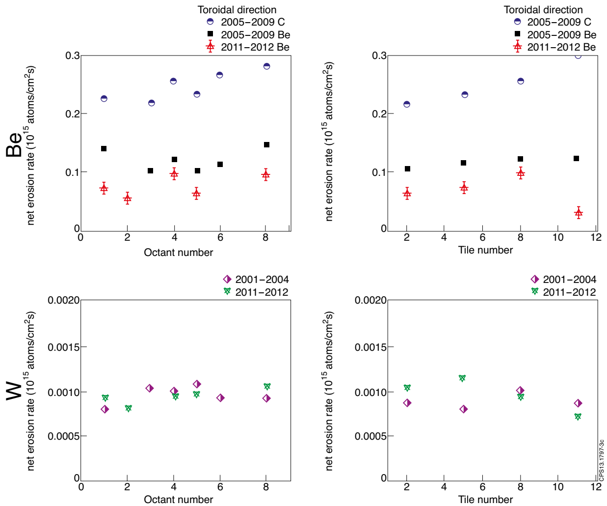
Figure 3: Poloidal and toroidal distributions of the erosion rates of W and Be during the 2011-2012 discharge campaign in comparison to the data for the 2005-2009 and 2001-2004 campaigns, respectively.
