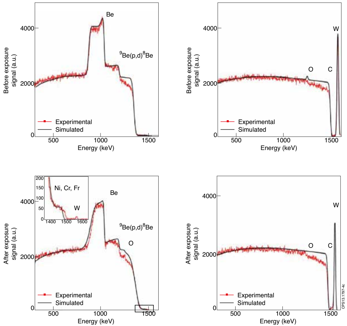
Figure 4: Typical RBS spectra before and after exposure for Be (on the left) and W (on the right) coated LTS. The Be spectrum includes a magnified area marked by the black rectangle on the spectrum.
