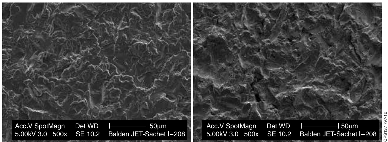
Figure 1: SEM images of Be (on the left) and W (on the right) layers on the LTS surfaces before exposure, 500x magnification.
