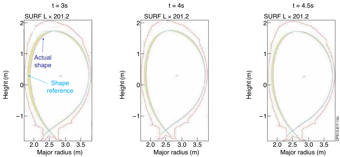
Figure 12: Shape tracking with the JET standard Shape Controller during the plasma current ramp-up (Pulse No: 83011).
