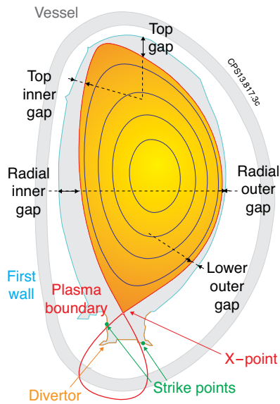
Figure 3: Plasma shape descriptors that can be controlled by the JET standard Shape Controller.
