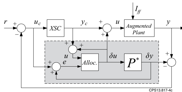
Figure 4: Block diagram of the allocated closed-loop. The Current Limit Avoidance is the grey shaded box, and takes both the controller input and output signals as an input.
