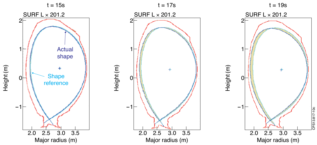
Figure 10: Shape tracking with the JET standard Shape Controller during the plasma current ramp-down (Pulse No: 77203).
