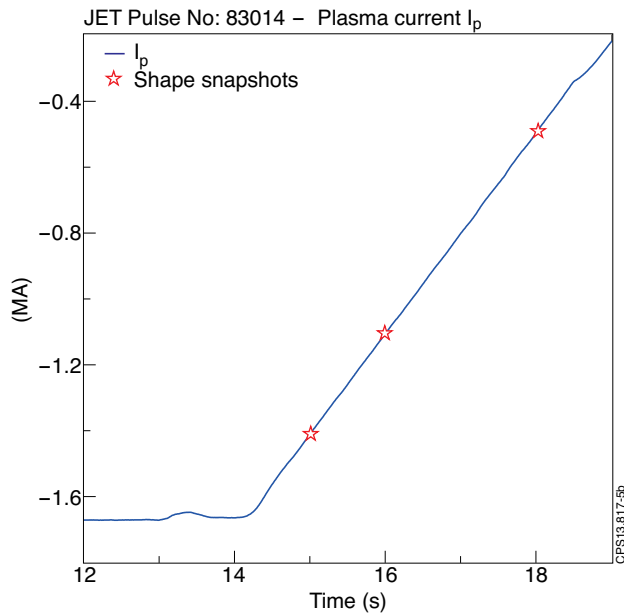
Figure 5: Plasma current during the ramp-down of the JET Pulse No's:72203 and 83014. The red markers show the time instants where the plasma snapshots shown in Figs. 10 and 11 have been taken.
