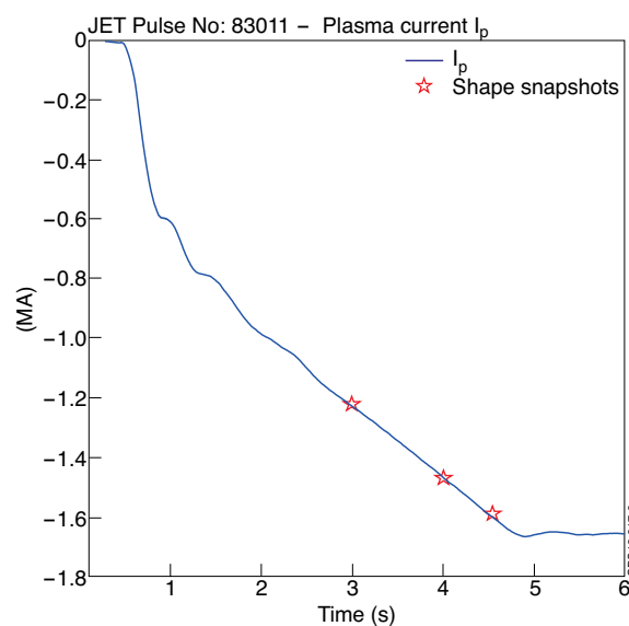
Figure 9: JET Pulse No: 83011, plasma current. The red markers show the time instants where the plasma snapshots shown in Figs.12 and 13 have been taken.
