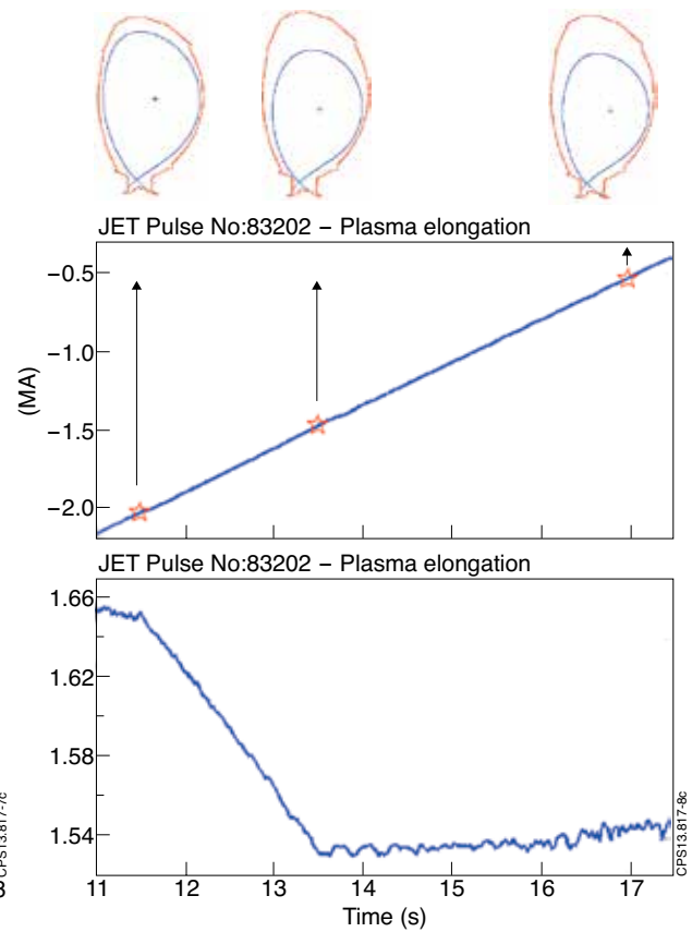
Figure 8: Change of the plasma elongation during the ramp-down (JET Pulse No: 83202). The elongation changes from \sim 1.66 to \sim 1.54 , while the plasma current is ramping down.
