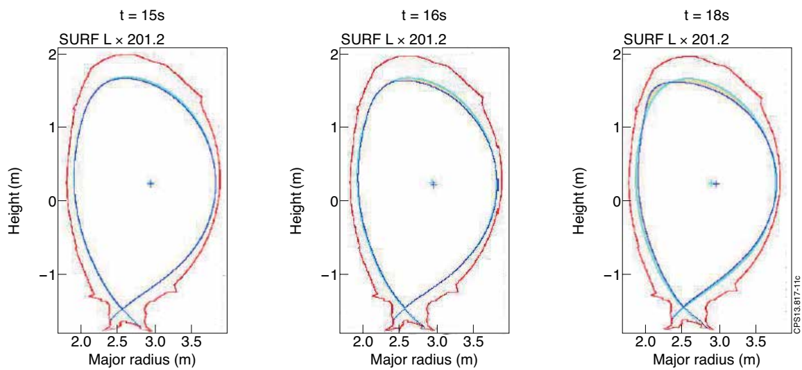
Figure 11: Shape tracking with the eXtreme Shape Controller during the plasma current ramp-down (Pulse No: 83014).
