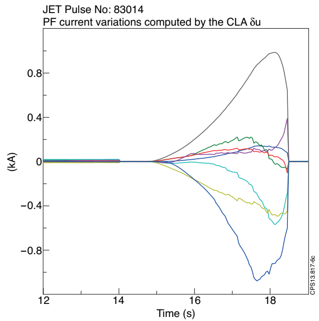
Figure 6: Outputs of the CLA. This plot shows the PF current variations u computed by the CLA and added to the XSC outputs.
