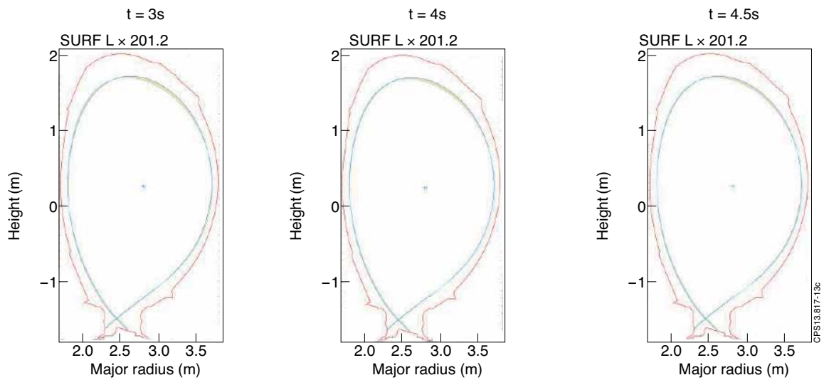
Figure 13: Shape tracking with the eXtreme Shape Controller during the plasma current ramp-up (Pulse No: 83014).
