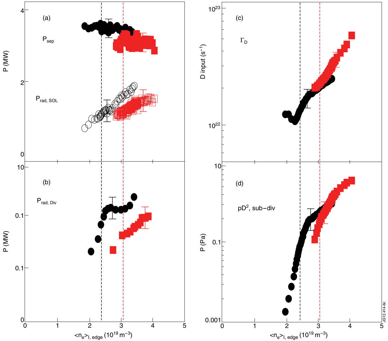
Figure 6: Total power across the separatrix and total radiated power in the main chamber and divertor SOL (a), total radiated power in the divertor region (b), total deuterium atom input (c), and molecular deuterium pressure in the sub-divertor. The data pertain to the high triangularity plasmas; black symbols refer to JET-C, and the red symbols to JET-ILW.
