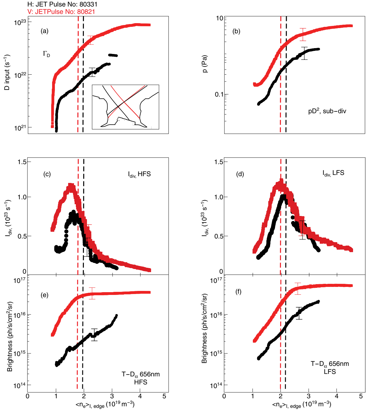
Figure 8: Total deuterium atom input (a), molecular deuterium pressure in the subdivertor (b), total ion currents to the HFS (c) and LFS (d) plates, and divertor leg integrated D_{\alpha} brightness across the HFS (e) and LFS legs (f) as function of line-averaged upstream density. The data were taken in JET-ILW in horizontal (black) and vertical (red) divertor plasma configurations shown in the insert.
