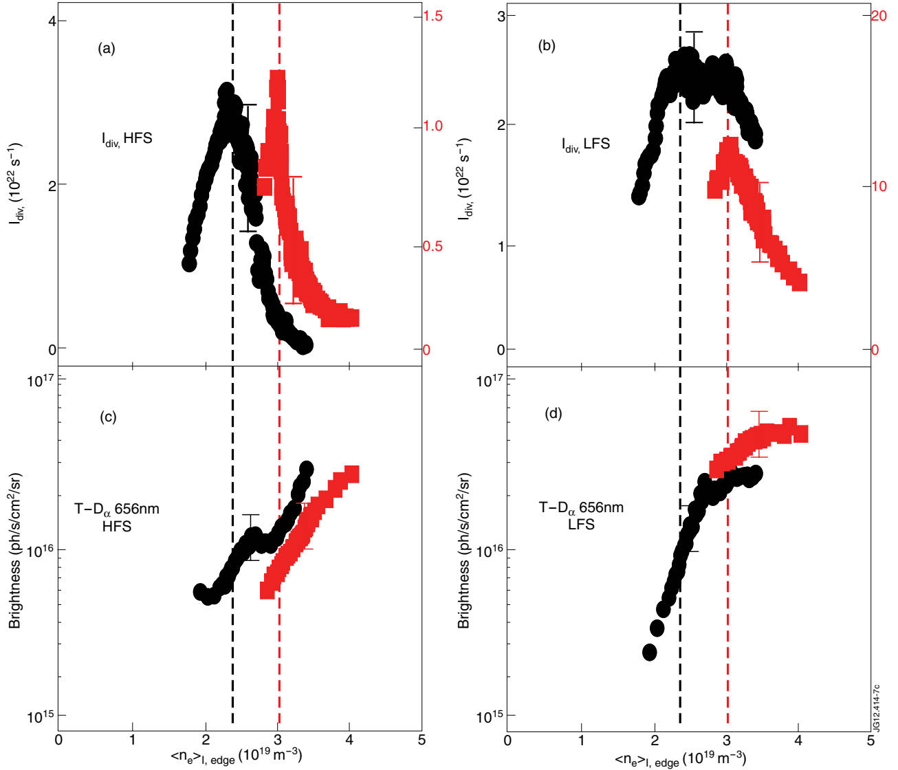
Figure 7: Total ion currents to the HFS (a) and LFS (b) plates, and divertor leg integrated D_\alpha brightness across the HFS (c) and LFS legs (d) as function of line-averaged upstream density. Colours as in Fig.6.
