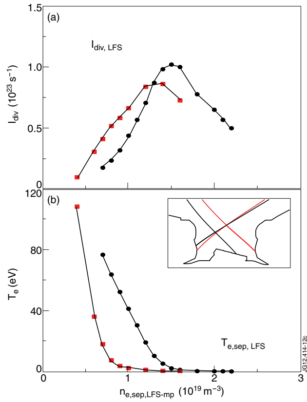
Figure 12: Predicted ion currents to the LFS plate (a) and electron temperature at the LFS plate separatrix (b) as a function of electron density at the LFS midplane separatrix. The black curves represent the horizontal and the red curves a corresponding vertical configuration
