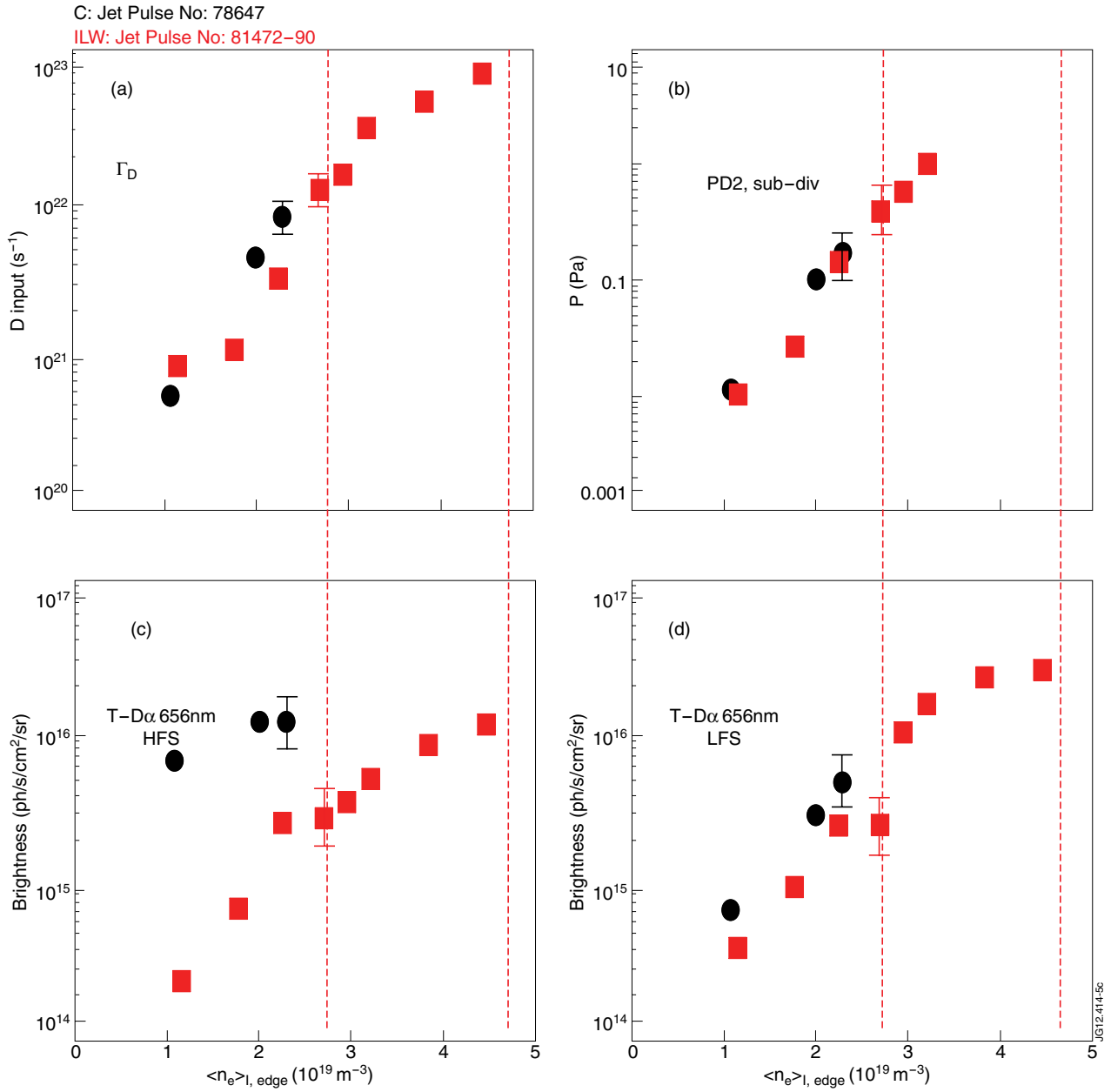
Figure 5: Total deuterium atom input (a), molecular deuterium pressure in the subdivertor near the cryo pump (b), and divertor leg integrated D_\alpha brightness across the HFS (c) and LFS legs (d) as function of line-averaged upstream density. Colours as in Fig.2.
