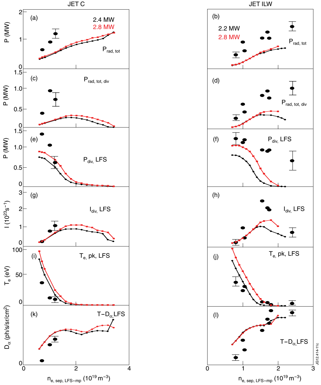
Figure 11: Comparison of the measured (symbols) and predicted (lines) total radiated power in the SOL (a,b), total radiated power in the divertor (c,d), conducted power to the LFS plate (e,f), total ion currents to the LFS plates (g,h), peak electron temperature (i,j), and D_{\alpha} emission integrated over the LFS leg (k,l) for JET-C wall (left column) and JET-ILW (right column) L-mode plasmas in horizontal configuration. The data is plotted as a function of upstream electron density at the separatrix. The simulated curves in black and red indicate the lower and upper bounds of the assumed power across the grid core boundary.
