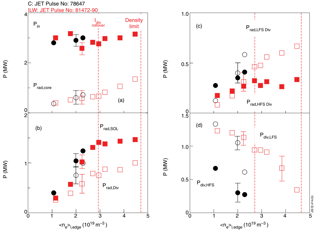
Figure 2: Total input power and radiated power in the core (a), radiated power in the entire SOL and in the divertor (b), total radiated power in the HFS and LFS divertor legs (c), and total conducted power to the HFS and LFS plates (d) as function of line-averaged edge density. Black symbols refer to JET-C, the red symbols to JET-ILW.
