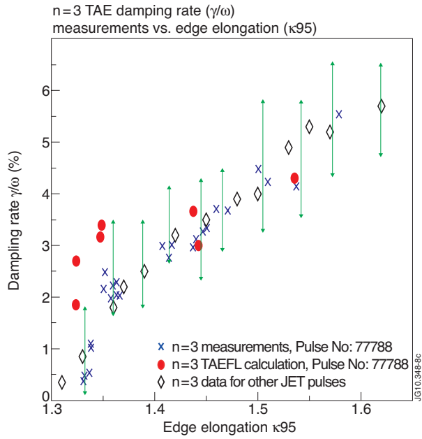
Figure 8. Damping rate data for n=3 TAEs as function of \kappa_{95} , showing an almost linear dependence \gamma/\omega_{MEAS}=f(\kappa_{95}) , compared with the results of the TAEFL simulations. The vertical double-pointed arrows indicate the scatter in the damping rate measurements obtained for these \kappa_{95} points: this scatter includes not only the estimated error on the individual \gamma/\omega_{MEAS} measurements, but also the variation observed for different JET discharges and background plasma parameters (absolute value and profiles) in \gamma/\omega_{MEAS} for n=3 modes at similar frequency within the TAE gap.
