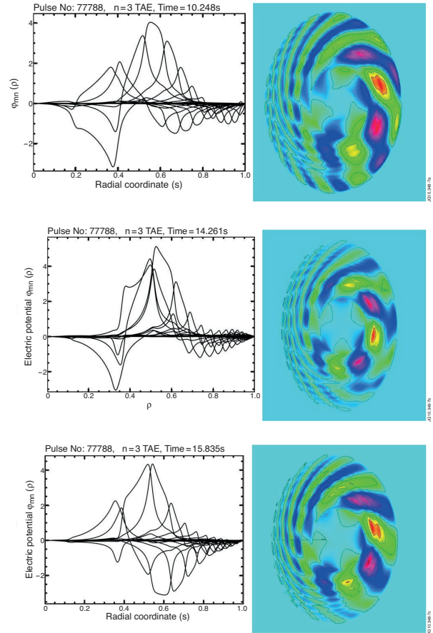
Figure 7. The radial Eigenfunction (left, expressed in terms of the electrostatic potential \Phi_{mn}(s) ) and the 2D contour plot (right) of the n=3 Eigenmode as calculated by the TAEFL code in the JET shot #77788 at t=10.248\text{sec} (top frame), t=14.261\text{sec} (middle frame) and t=15.835\text{sec} (bottom frame). The radial coordinate is s=\sqrt{\psi_N} as in fig4.
