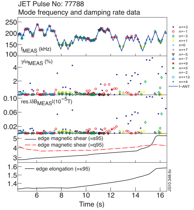
Figure 5. Measurement of the mode frequency ( f_{MEAS} ) and damping rate ( \gamma/\omega_{MEAS} ) for individual toroidal mode numbers for the JET shot #77788 as function of the evolution of the edge magnetic shear ( s_{95} ) and elongation ( \kappa_{95} ). The various n -modes that have been detected are ordered in the plot according to decreasing residue amplitude, as measured using magnetic pick-up coils located on the low-field side. The typical uncertainties on the measured mode frequency and damping rate are below <1\text{kHz} and 15% for the measurements presented here (see [6] for further details). Note that modes with the same toroidal mode number are detected at almost the same time at different frequencies within the TAE gap and with very different damping rate, hence the importance of being able to track in real-time the evolution of one specific single n -mode.
