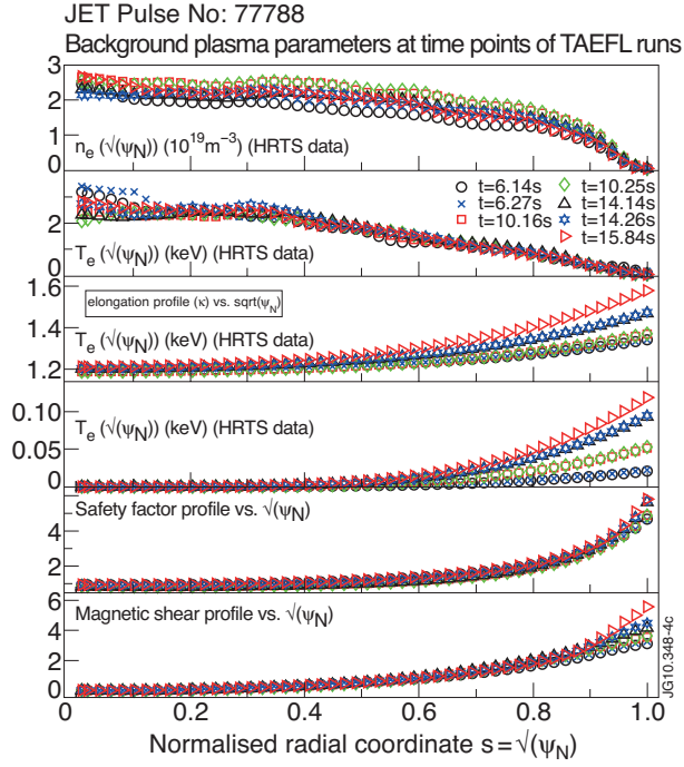
Figure 4. The profiles of the main background plasma parameters at the time points used for the TAEFL simulations (note that T_i \sim T_e ). The equilibrium current and shaping data are computed using the EFIT code, the electron density and temperature are from the HRTS measurements. The error bars on the n_e , T_e , shaping, safety factor and magnetic shear profile are all within 5→10% across the entire poloidal cross-section (not shown to avoid excessive cluttering in the figure).
