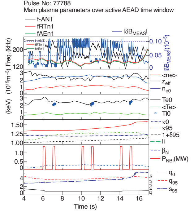
Figure 3. The main background plasma parameters for the JET shot #77788: the toroidal field on the magnetic axis is B_\phi=2.7 T, the plasma current is I_p=2 MA. The labels f-ANT, fRTn1 and fAE n1 indicate, respectively, the antenna driving frequency, the antenna driving frequency, and the central frequency of the n=1 TAE gap at \sqrt{\psi}N=0 calculated in real-time by the AELM (assuming q_{TAE}=(2m+1)/2n=1.5 , R=3 m, and using the line-averaged value of the electron density in the plasma core from the interferometer measurements) and post-pulse using the EFIT (+MSE) measurement of the q -profile in the plasma core and the measurement of the core electron density obtained via the High-Resolution Thomson Scattering diagnostic. Here q is the safety factor and s the magnetic shear, \beta_N is the normalized plasma beta and P_{NBI} is the NBI blip power, \kappa is the elongation, \delta is the averaged up/down triangularity, li is the plasma internal inductance, T_e and T_i are the electron and ion temperatures, n_e is the plasma density, z_{eff} is the effective charge, with the suffixes “0”, “95” and “<>” indicating the core, edge and volume-averaged values, respectively. For illustrative purposes, the signal from one of the synchronously acquired magnetic pick-up coils is also shown in the top frame.
