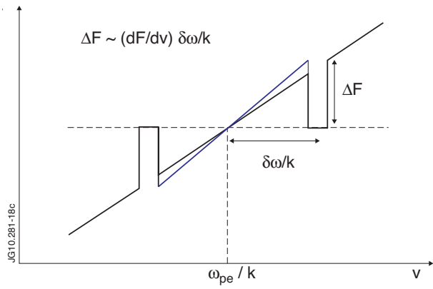
Figure 26: (Color online) Cartoon illustrating the motion of holes and clumps and the wake (dotted line) that acts to steepen to distribution function, creating a favourable environment for instability.
