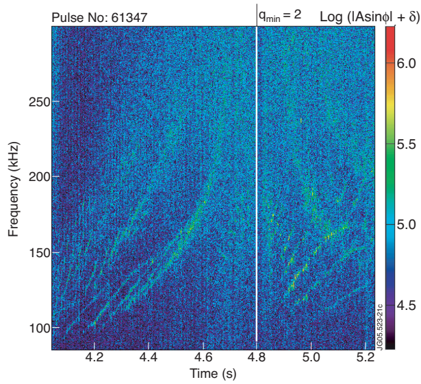
Figure 6: Alfvén cascades detected with O-mode interferometry in JET pulse no: 61347. Due to the Doppler shift n f_{ROT} in this toroidally rotating plasmas the discrete spectrum observed spreads over a broad frequency range. A grand cascade is seen at t = 4.8s .
