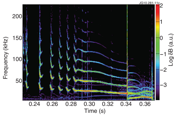
Figure 20: Magnetic spectrogram showing fishbone oscillations that initiate a long-lived n = 1 kink mode (at frequency 30 kHz) in MAST pulse no: 16038. The long-lived mode degrades the plasma performance and causes internal reconnection event at t = 0.34s .
