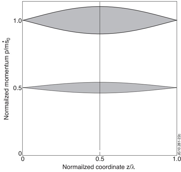
Figure 16: Evolution of the phase-space bucket during sweeping event. The plot shows the initial separatrix (upper shaded area) and the shrunk separatrix at half of the initial mode phase velocity (lower shaded area).
