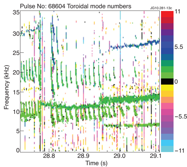
Figure 22: Magnetic spectrogram showing toroidal mode numbers of the perturbations in figure 21.
