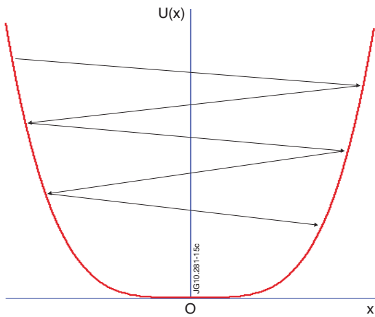
Figure 24: Damped oscillations in a quartic potential well illustrate nonlinear frequency downshift during fishbone pulse decay.
