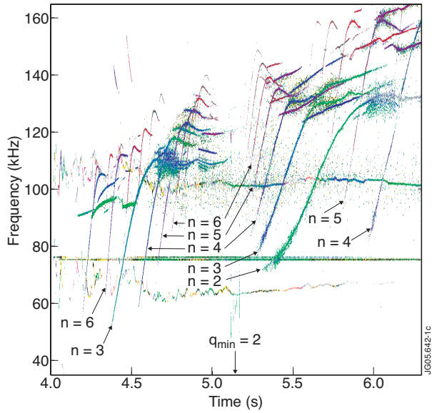
Figure 1: Magnetic spectrogram (Fourier decomposition of Mirnov coil signal) showing an example of ICRH-driven ACs with different toroidal mode numbers in a JET reversed shear plasma.
