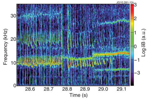
Figure 21: Magnetic spectrogram showing typical JET hybrid scenario with n = 1 NBI-driven fishbones. Long-lived NTM at frequency around 12-15 kHz (lab reference frame) is initiated in the absence of sawteeth or ELMs at t = 28.77s and after some time it eventually degrades thermal plasma confinement.
