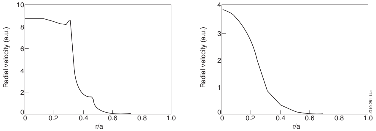
Figure 23: The radial velocity profiles in the linear (left) and nonlinear (right) regimes.
