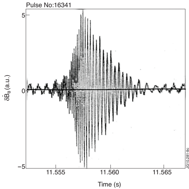
Figure 18: Oscillations of the perturbed magnetic field time derivative during fishbone burst (JET pulse no: 16341).
