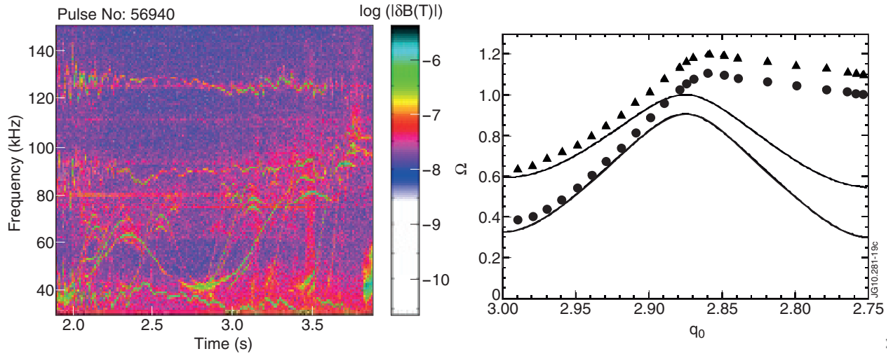
Figure 8: Left: Magnetic spectrogram showing Alfvén cascades in JET pulse no:56940. Alfvén cascades with different toroidal mode numbers reach the same lowest frequency. Right: Alfvén spectral line behavior computed from theory [34], showing the effect of pressure on the mode frequency as a function of safety factor q_0 . The solid curve represents the MHD continuum, and the triangular and the circular points are for \beta = 0.005 and \beta = 0.0015 , respectively.
