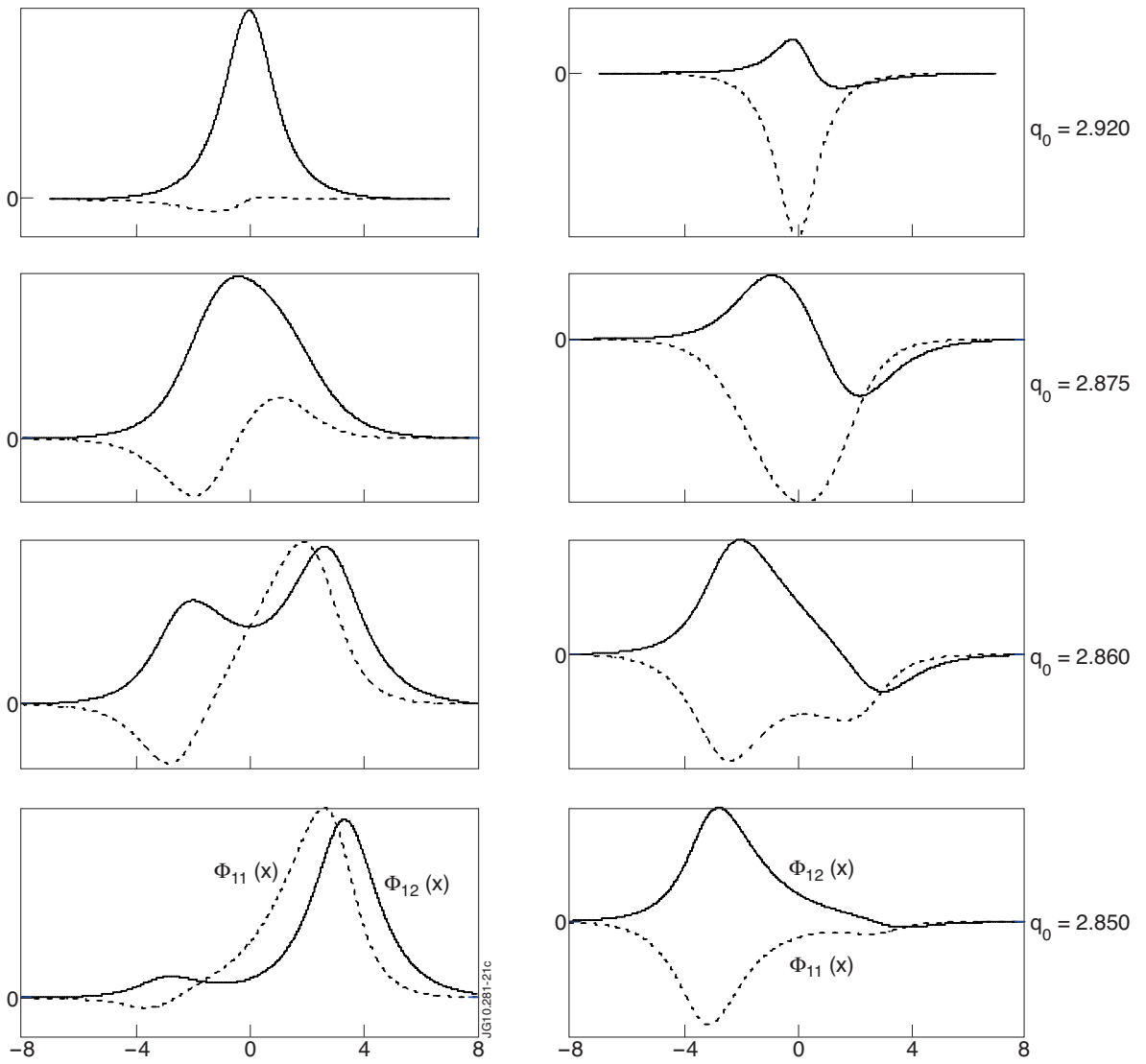
Figure 2: Snapshots of the mode structure for n = 4 and m = (12; 11) during the transition from AC to TAE. Left column shows the radial profiles of the poloidal components for the even parity TAE; right column presents the odd parity mode.
