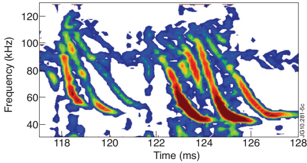
Figure 14: NBI-driven chirping modes on MAST
