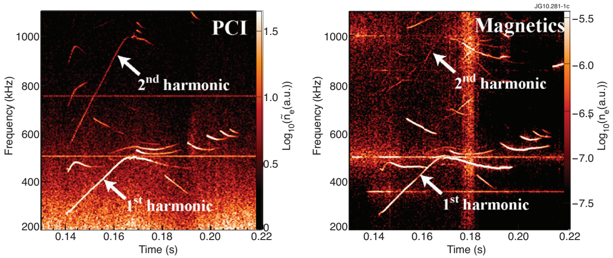
Figure 10: Second harmonic of Alfvén cascade and TAE is observed in Alcator C-Mod [14] on the PCI diagnostic (left) and hardly seen on the magnetic pick-up coils (right).
