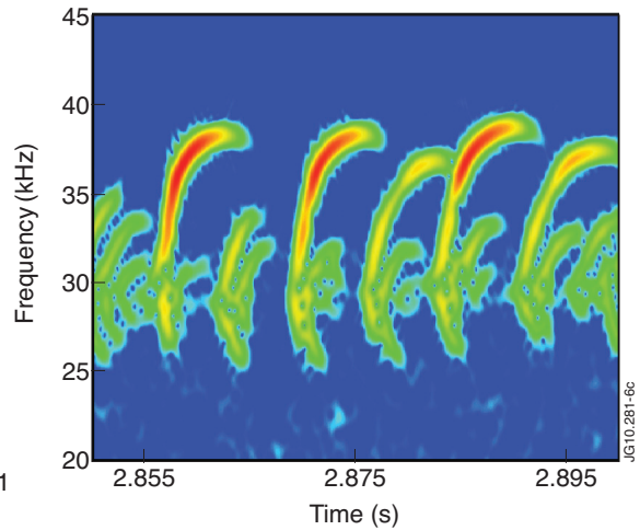
Figure 15: Left: phase magnetic spectrogram showing modes with various toroidal mode numbers excited by ICRH in JET pulse no:54895. The n = 0 mode is seen at around 30 kHz and marked in black color. ACs are seen in the range of 40-110 kHz. Right: the n = 0 mode in JET pulse No: 54895 (zoom).
