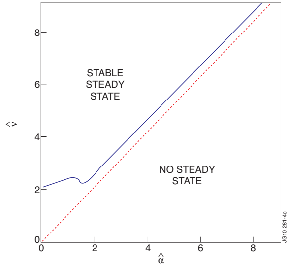
Figure 13: Displays the boundaries in parameter space that give stable, unstable and no steady state solutions to (10). The unstable solution lies in between the solid and dashed lines.
