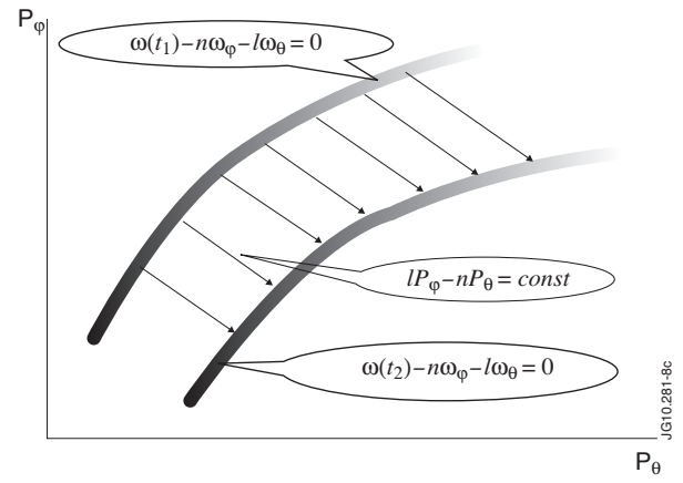
Figure 17: Transport of resonant particles during frequency sweeping. The shaded areas are snapshots of the moving resonant region in the momentum space. The shades of gray mark different values of the particle distribution function. The trapped resonant particles form a locally flat distribution across the resonance and preserve the value of their distribution function when the resonance carries them along the dashed lines.
