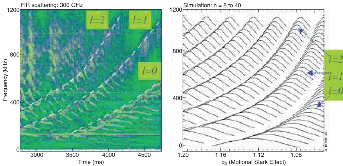
Figure 7: Left: Evolution of far infrared scattering spectrum showing Alfvén cascades in DIII-D discharge. Right: model analysis of frequency evolution of Alfvén continuum at q_0 indicating toroidal mode numbers in the range from 8 to 40 (from [40]).
