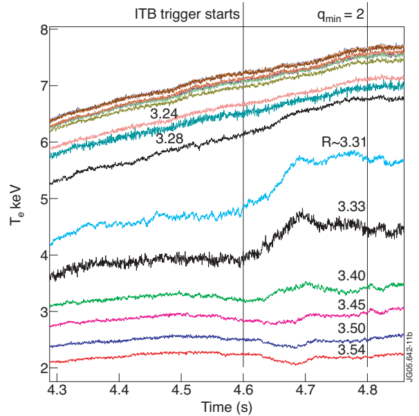
Figure 5: Electron temperature traces measured with multi-channel ECE in JET pulse no: 61347. An ITB triggering event is seen at t = 4.6 \text{ s} .
