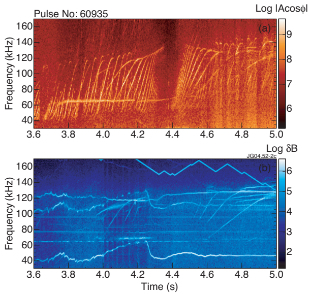
Figure 4: Alfvén cascades detected in the same (JET pulse no: 60935) with O-mode interferometry (top) and with Mirnov coils (bottom). Microwave beam frequency 45.2GHz was just above the cut-off frequency of the O-mode.
