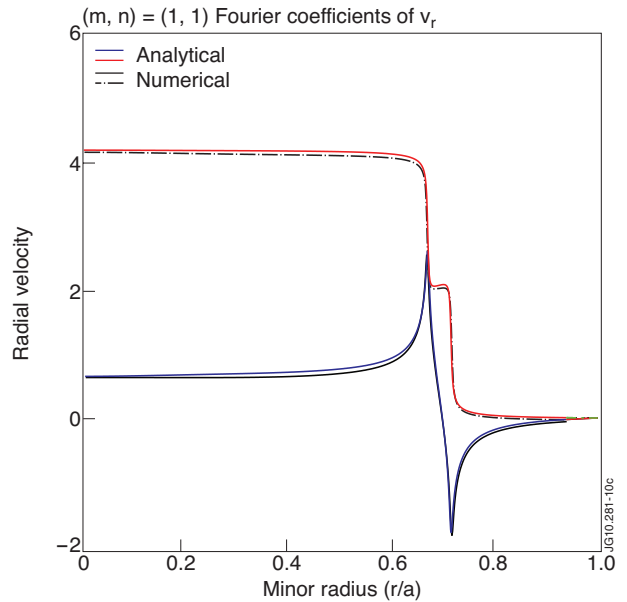
Figure 19: Spatial structure of the fishbone perturbation in the near-threshold regime. The real (red) and imaginary (blue) parts of the radial velocity profile show two well-separated resonant sub-layers near the surface. The width of each sub-layer is proportional to the mode growth rate. The distance between the sub-layers is proportional to the mode frequency.
