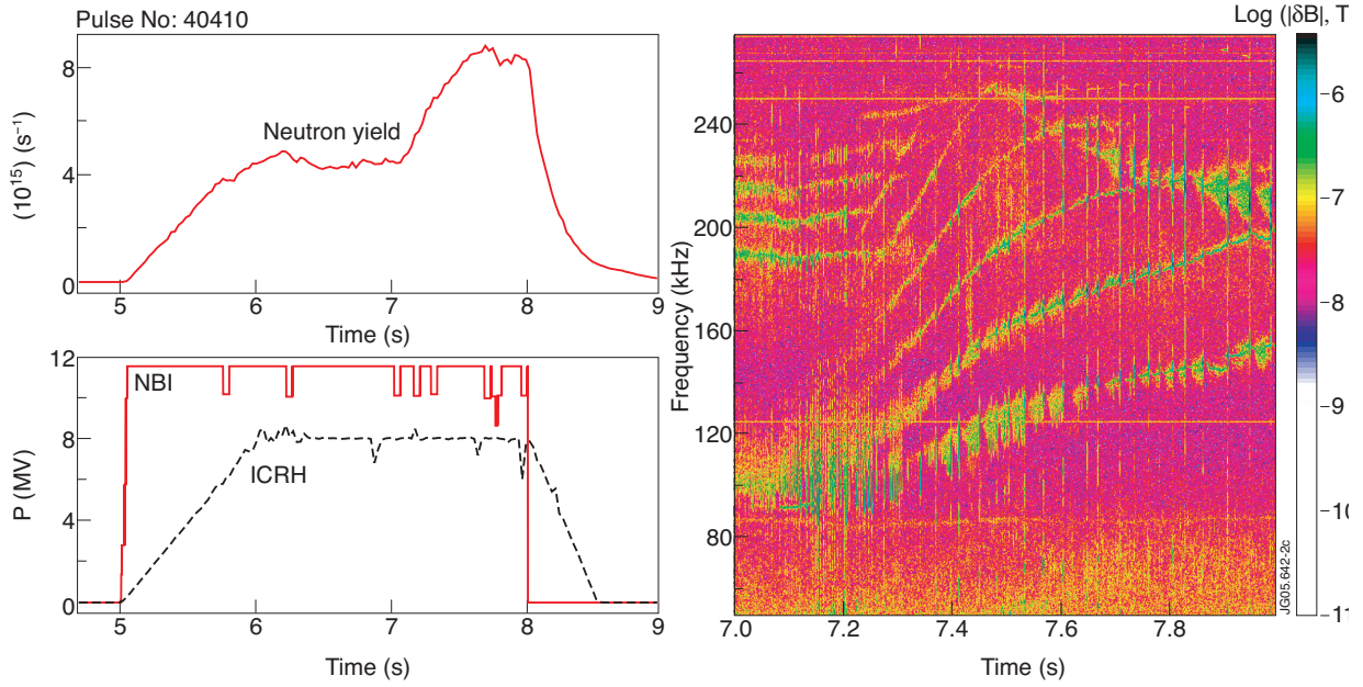
Figure 3: Left: Neutron yield, NBI and ICRH power in JET pulse no: 40410 with toroidal magnetic field B_r = 3.4 \text{ T} and plasma current I_p = 3 \text{ MA} . Right: grand cascade observed at the time of the neutron rate and T_e increase.
