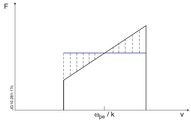
Figure 27: (Color online) Cartoon illustrating how holes and clumps might form a global plateau in a distribution function with a finite extent in velocity space. The dashed lines mark the boundaries of the 'stacked up' holes and clumps.
