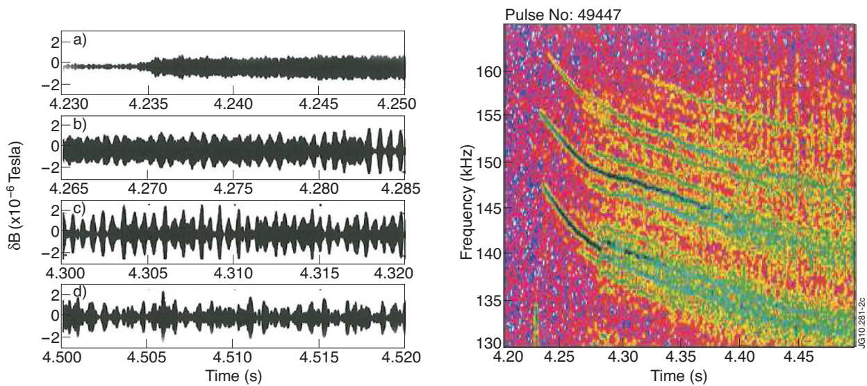
Figure 11: At gradually increasing ICRH power, TAEs exhibit steady state, periodically modulated, and chaotic regimes. Left panel shows the magnetic probe signals. Right panel shows magnetic spectrograms obtained via Fourier decomposition of the signals.
