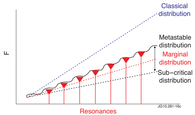
Figure 25: (Color online) Cartoon illustrating intermittent quasilinear relaxation due to resonance overlap in the multi-mode regime. The resonances broaden and eventually overlap as the modes grow above the instability threshold. The energetic particle population drops to subcritical values and then is replenished by the source to a metastable level that exceeds the linear threshold level due to separation of neighboring linear resonances.
