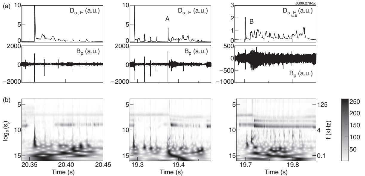
Figure 5: JET Pulse No: 59423 (a) time trace of D_{\alpha,E} measured in the divertor region, and of \dot{B}_p measured on the outboard plane, in the case of spontaneous compound ELMs (left), pellet A (center) and pellet B (right). (b) Wavelet scalogram computed in the same time windows. The sawtooth precursors with n = 1,2 and the NTM are visible in the wavelet scalogram.
