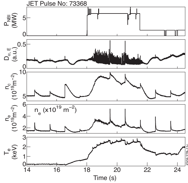
Figure 11: JET Pulse No: 73368. B_T = 2.5T , I_P = 2.0MA , P_{RF} = 3MW . Time traces of the NB injected power (a), of the D_\alpha emission measured in the inner divertor (b), of the line integrated electron density measured at the plasma axis n_c (c) and at the edge n_e (d), and of the electron temperature T_e measured at 3.4m.
