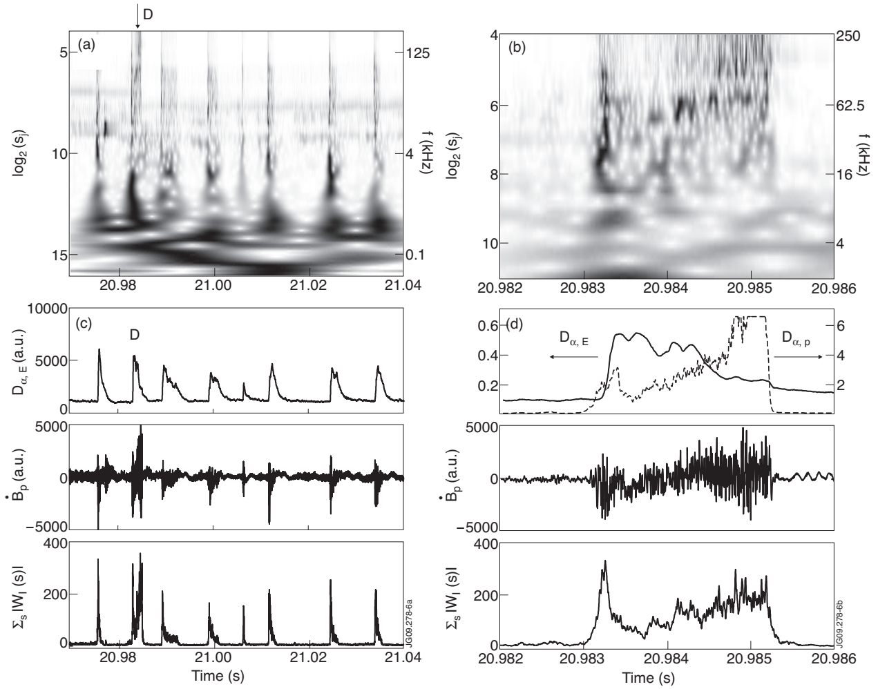
Figure 6: JET Pulse No: 59423. (a) Wavelet coefficients measured during injection from the inboard track. (b) Extended view in a time window centred on the pellet-triggered event D. (c)-(d) time trace of the D_{\alpha,E} , D_{\alpha,P} , of the absolute value of wavelet coefficients, integrated over frequencies larger than 15kHz, \Sigma_s |W_l(s)| , in the same time window as (a) and (b).
