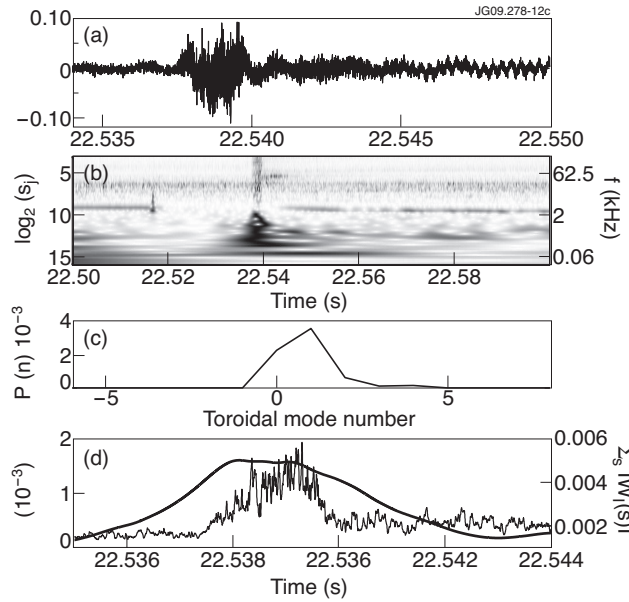
Figure 12: JET Pulse No: 73368, L-mode phase. (a) magnetic perturbations in a time window centred on the triggered event. (b) Power spectral density of magnetic perturbations (arbitrary units) in a window centred on the ELM triggered by pellet C. For graphical purposes data are plotted with the reduced time resolution of 20s. (c) Toroidal mode number spectrum at low frequencies \log_2(s_i) = [9.5, 12] , computed during t = [22.5385, 22.5395] . (d) Amplitude of magnetic perturbations (arbitrary units), integrated over frequencies higher than 4kHz (thin line, left axis) and over frequencies below 4kHz (thick line, right axis).
