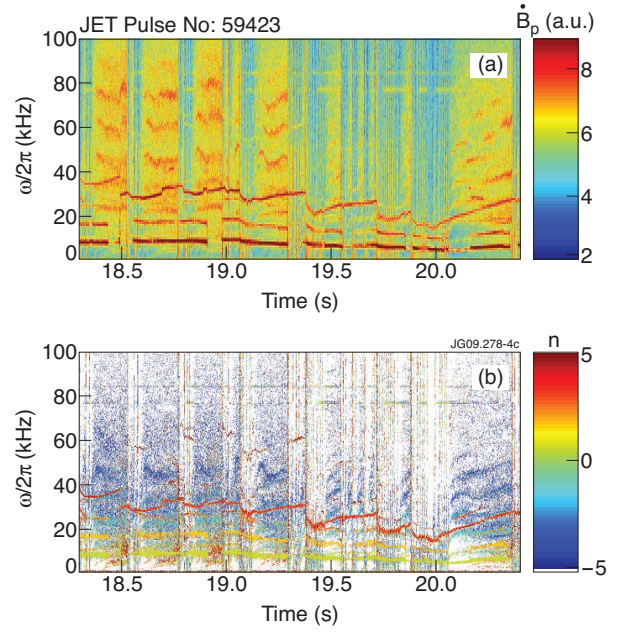
Figure 4: JET Pulse No: 59423. (a) Windowed Fourier spectrum, calculated over overlapping time windows of length 2ms. (b) toroidal mode numbers, extracted from the phase shift between Mirnov pickup coils toroidally separated by 10.17 degrees.
