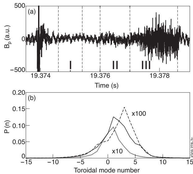
Figure 7: JET Pulse No: 59423. (a) Magnetic perturbations \dot{B}_p measured by the outer edge Mirnov coil H302 in a time window centred on the pellet-triggered event A (see Fig.2). (b) Toroidal mode number spectrum associated with spectral components at frequencies higher than 15kHz, computed during time window I (dashed line), time window II (thin line) and during time window III (thick line).
