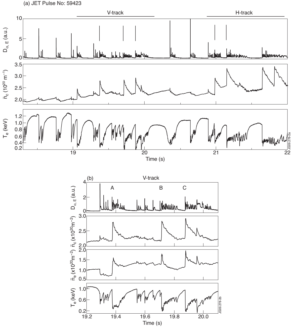
Figure 2: JET Pulse No: 59423: B_T = 2.4 \text{ T} , I_P = 2.5 \text{ MA} , P_{\text{NBI}} = 15 \text{ MW} , P_{\text{RF}} = 3 \text{ MW} . (a) Time traces of the D_{\alpha} emission measured in the inner divertor, of the line integrated electron density measured through a line sight intersecting the plasma axis \bar{n}_{ec} and of the electron temperature T_e measured inside the edge transport barrier, in the pedestal region. Vertical lines in the top plot indicate pellets that are not fragmented. (b) extended view over the time window where pellets are injected from the top (vertical track). (c) extended view over the time window where pellets are injected from the high field side (inboard track). The line integrated density measured at the edge, n_e , is shown in (b) and (c) for comparison. A-E indicate pellet-triggered events, F indicate a spontaneous ELM almost synchronous with the injection of a pellet.
