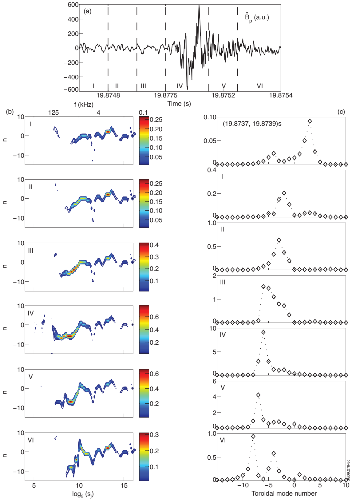
Figure 8: JET Pulse No: 59423, pellet C. (a) time trace of magnetic perturbations \dot{B}_p of the pELM triggered by event C. (b) Scale dependent toroidal mode number spectrum P(n, s) , computed over the time windows I-VI, as indicated in (a). (c) Toroidal mode number spectrum, P(n) , obtained integrating P(n, s) over scales \log_2(s_j) = [4, 10] . For comparison it is also shown P(n) computed 1ms before the pELM crash (top frame).
