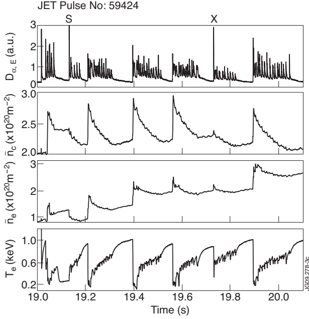
Figure 3: JET Pulse No: 59424: B_T = 2.4T , I_p = 2.5MA , P_{NB} = 15MW , P_{RF} = 3MW . Extended view of the time window where pellets are injected from the vertical track. Time traces of the D_{\alpha} emission measured in the inner divertor, of the line integrated electron density close to the plasma axis \bar{n}_{e,c} , at the edge n_e and of the electron temperature T_e measured inside the edge transport barrier, in the pedestal region. ‘S’ denotes a spontaneous ELM, ‘X’ a fragmented pellet.
