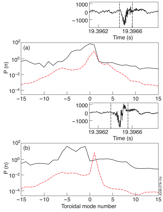
Figure 10: Toroidal mode number spectrum of spontaneous (JET Pulse No: 59423) (a) and triggered ELM (JET Pulse No: 59424) (b), measured 1ms before (thin line), and during the ELM (thick line). The insets show the time trace of magnetic perturbations, with vertical dashed lines indicating the time window where the power spectrum is measured.
