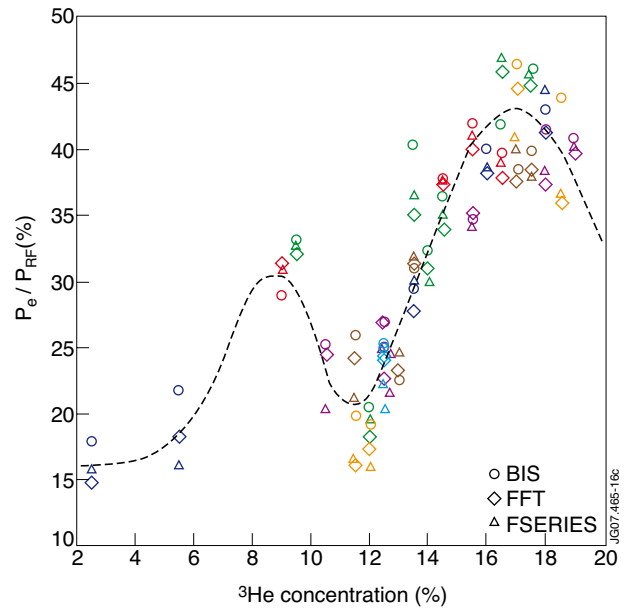
Figure 13: Power fraction directly or indirectly absorbed by the electrons for shots 66413-66437 as a function of X[{}^3\text{He}] . Various analysis techniques were adopted. Circles, diamonds and triangles denote results obtained using Break-in-Slope, Fast Fourier Transform and truncated Fourier series analysis, respectively. Optimal electron heating occurs at X[{}^3\text{He}] 17–19%, a secondary maximum is found at X[{}^3\text{He}] 8–9% while the absorption is poorest at X[{}^3\text{He}] 11–13% and at low concentration.
