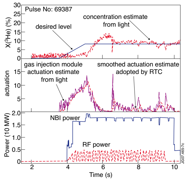
Figure 7: Example of real time control of the ^3\text{He} concentration (based on the photon fluxes - e.g. the intensity of the D_\alpha line - emitted by various ion species) for discharge 69387: desired concentration and actual concentration as estimated using the simplified formula adopted by the real time controller (top), raw gas injection module valve actuation required to ensure the desired concentration is maintained (inferred from the simple formula) as well as smoothed actuation actually used (middle), and NBI and RF power level (bottom). Note that it takes some time for the real time controller to match the desired concentration: when the auxiliary power is switched on the whole plasma is undergoing a slow evolution towards a steady state regime and freezing the concentration is nontrivial.
