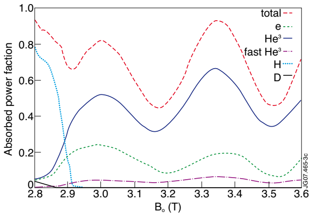
Figure 3: Fraction of the launched wave power absorbed in a double pass over the plasma as a function of the toroidal magnetic field strength; X[{}^3\text{He}] = 10\% and other parameters as for the thermal plasma.
