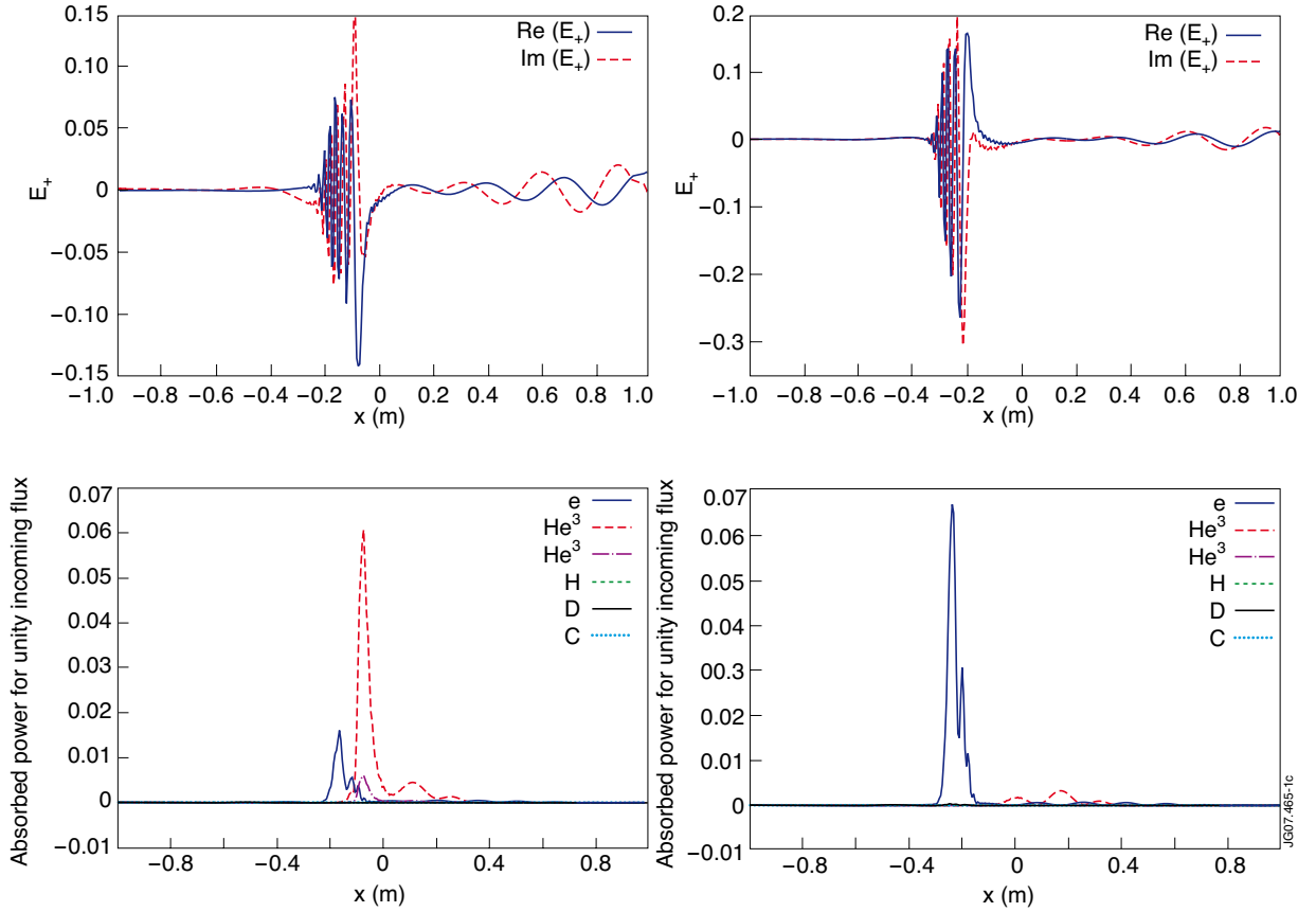
Figure 1: Electric field structure of the field component rotating with the ions (top) and power deposition profile (bottom) for predominant minority (10% ^3\text{He} ; left) and mode conversion (20% ^3\text{He} ; right) heating. The quantities are plotted as a function of x , the distance from the geometric centre: x = R - R_o . An analytical D-shaped equilibrium [4] has been adopted. Note that the dominant absorption shifts position as the efficiency of the competing absorption mechanisms changes due to the fact that the local wave polarization's dependence on the minority concentration.
