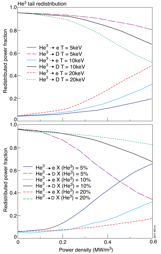
Figure 4: Collisional redistribution of the power absorbed by the {}^3\text{He} minority to the electrons and bulk D ions as a function of the minority RF power density: (top) temperature scan, (bottom) {}^3\text{He} concentration scan; other parameters as for the thermal plasma TOMCAT runs.
