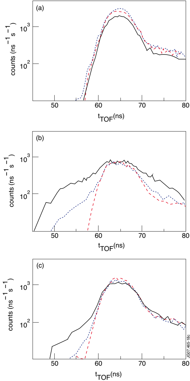
Figure 15: Neutron time of flight spectra (number of counts as function of flight-time - t_{\text{TOF}} ) from the TOFOR neutron spectrometer. The top panel (a) shows data for pulse 69388 ( X[{}^3\text{He}] = 10\text{-}12\% : minority heating regime), the middle (b) and bottom (c) panels correspond to pulses 69392 and 69393 ( X[{}^3\text{He}] = 18\% : mode conversion regime). Each panel displays spectra for three different contiguous time slices during the magnetic field flat top: short dashes for t = 5\text{-}6\text{s} , long dashes for t = 6\text{-}7\text{s} , solid lines for t = 7\text{-}8\text{s} . The statistical uncertainties follow Poisson statistics, i.e. 100 counts give a 10% and 1000 counts a 3.2% accuracy.
