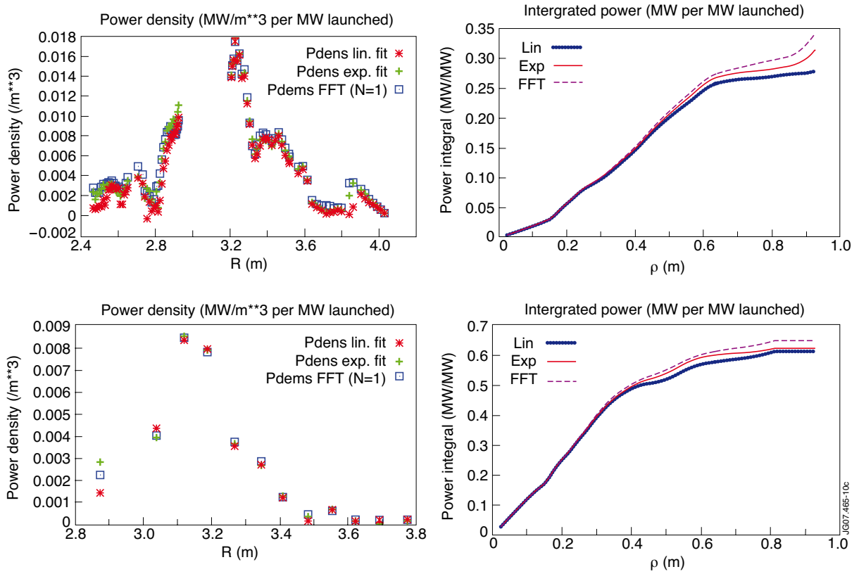
Figure 10: Power density as a function of major radius: On-axis RF heating (shot 69387) with main parameters B_o = 3.35T, f = 33MHz (dipole phasing), T_{o,e} = 7 - 8keV, T_{o,i} = 14keV, N_{o,e} = 4 \cdot 10^{19} m^{-3} : (top left) electron power density, (top right) integrated electron power absorption, (bottom left) ion power density, (bottom right) integrated ion power absorption
