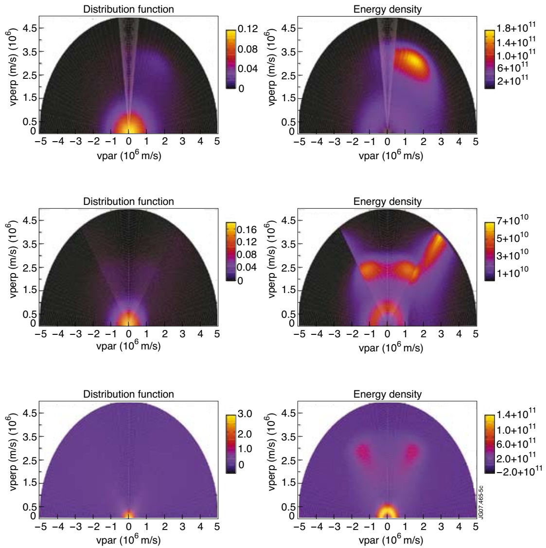
Figure 5: RF heated D beam distribution (left) and corresponding energy density (right) in a (v_{\perp}, v_{\parallel}) diagram - the parameters chosen qualitatively represent those of the combined 80+130keV & normal and tangential JET beams: (top) \rho = 0:02m , (centre) \rho = 0:50m , (bottom) \rho = 0:90m ; r is the magnetic surface labeling parameter.
