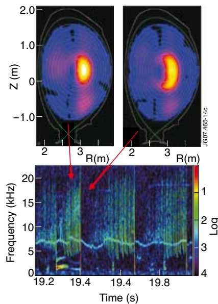
Figure 11: Tomographical reconstruction of the gamma ray emissivity for gamma's with energies exceeding 2.2MeV. The top plots represent the emissivity averaged over 150ms just prior to (left) and just after (right) a sawtooth crash. The bottom plot is the frequency spectrum of the plasma's magnetic activity as a function of time, showing the presence of fishbone activity prior to sawtooth crashes.
