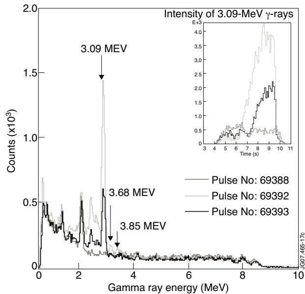
Figure 14: Gamma ray spectra recorded from 7.5s to 9.5s in discharges 69388, 69392 and 69393. The temporal evolution of the rate of the 3.09MeV gamma-line resulting from reaction {}^{12}\text{C}(\text{D}; p\gamma){}^{13}\text{C} marked in the spectra is shown in the inset; the same grey coding is used in both figures.
