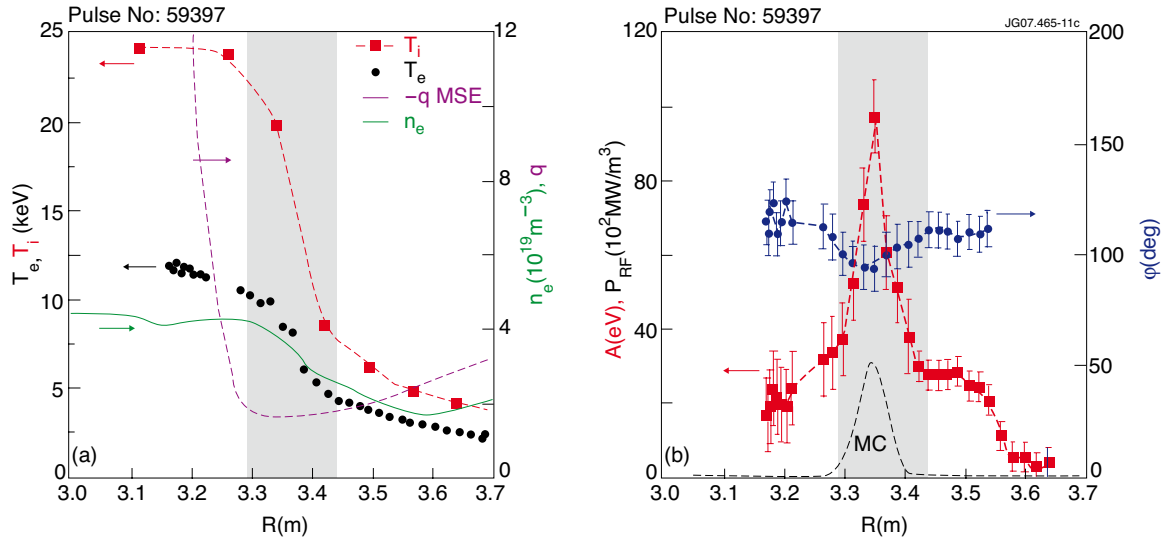
Figure 18: Transport analysis of ITB shot 59397 (reproduced from [14]) showing various quantities as a function of the major radius: (a) deeply reversed q -profile, density, ion and electron temperature profiles, (b) amplitude and phase of the fundamental Fourier component as well as the power deposition profiles adopted in the simulation. Reprinted figure with permission from P. Mantica et al., Phys. Rev. Letters 96 0950020 (2006). Copyright (2006) by the American Physical Society.
