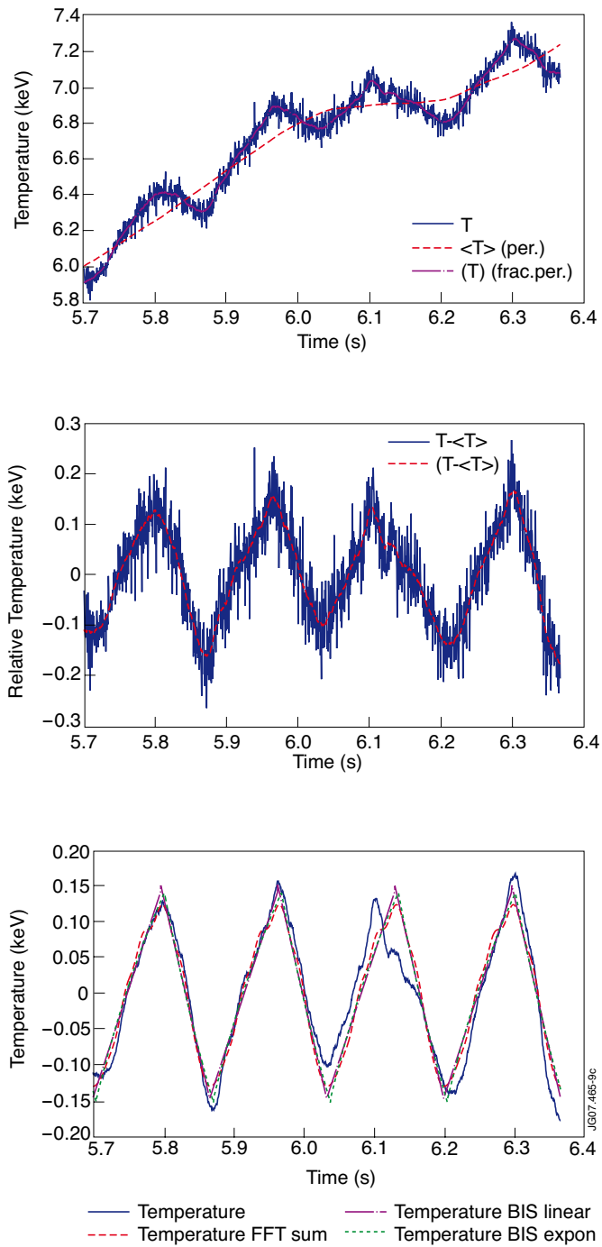
Figure 9: Electron temperature response at R \sim 3.2m to RF power modulation for shot 69387 during the ITB shown as a function of time: (top) raw ECE data T_e as well as data smoothed over a full modulation period \langle T_e \rangle to remove slow time variation and [T_e] over a fraction (typically 20% of the period) to remove the most rapid variation but retaining modulation-related trends, (middle) T_e - \langle T_e \rangle and [T_e - \langle T_e \rangle] (input for further data analysis), (bottom) FFT fit, linear fit and exponential fit of [T_e - \langle T_e \rangle] .
