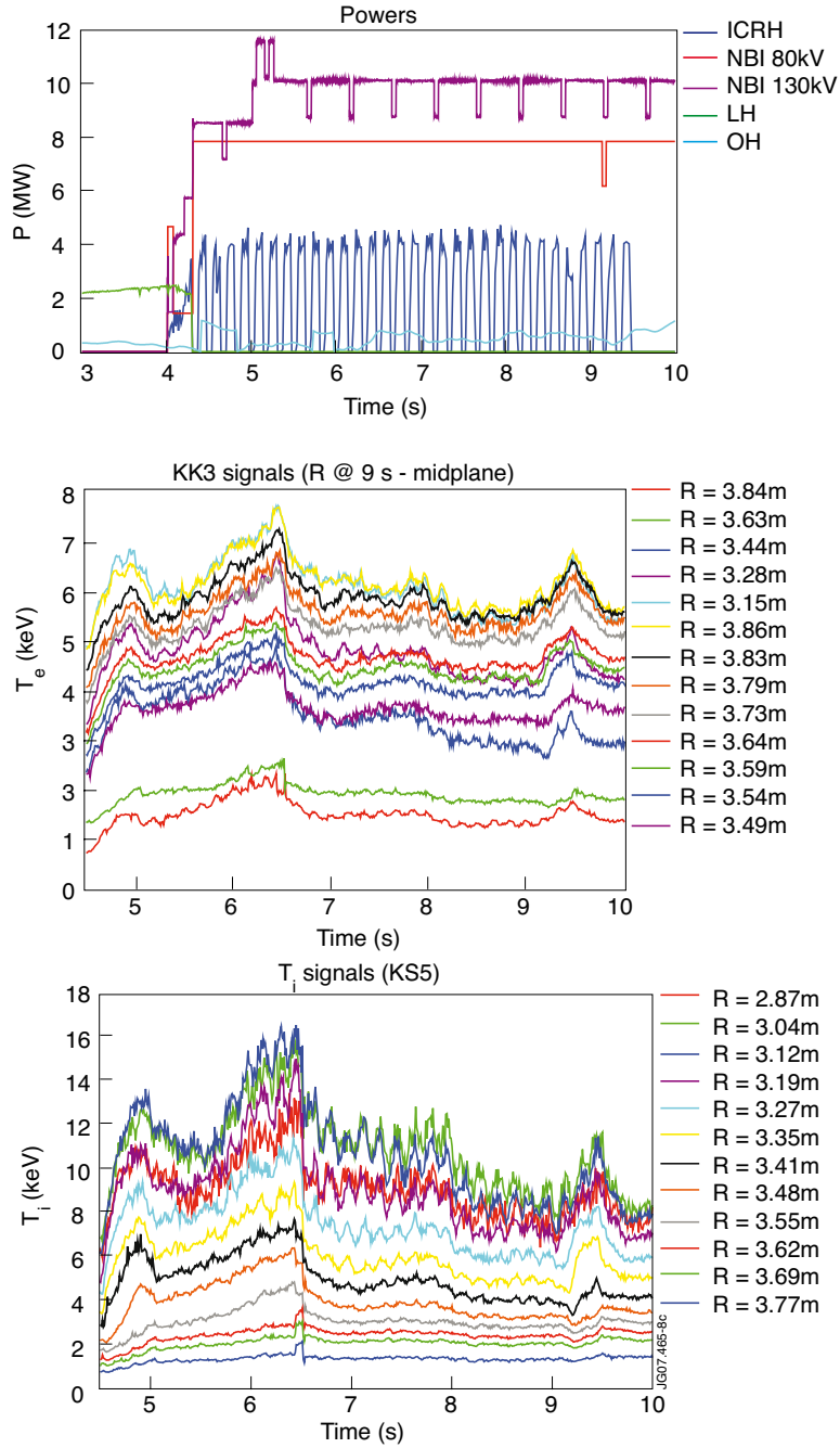
Figure 8: On-axis RF heating (shot 69387) shown as a function of time: (top) various power levels, including the RF power PICRH modulated at a frequency of 6Hz, (middle) electron temperature T_e and (bottom) ion temperature T_i as a function of time. The charge exchange periscope from which T_i was inferred was tuned to ^3\text{He} .
