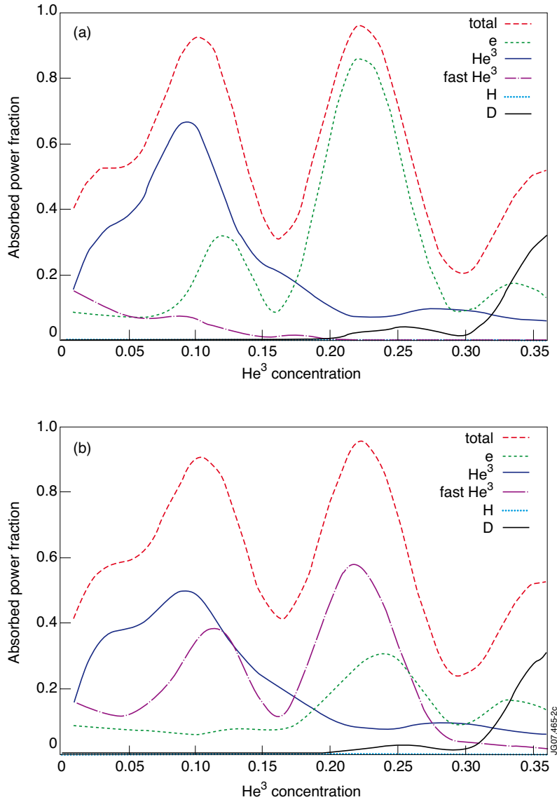
Figure 2: Fraction of the launched wave power absorbed in a double pass over the plasma as a function of the 3 He concentration when: (a) all ion species are thermal, sharing the same core temperature of T_o = 10\text{keV} , (b) thermal ions are considered but 1% of the 3 He ions has T_o = 100\text{keV} .
