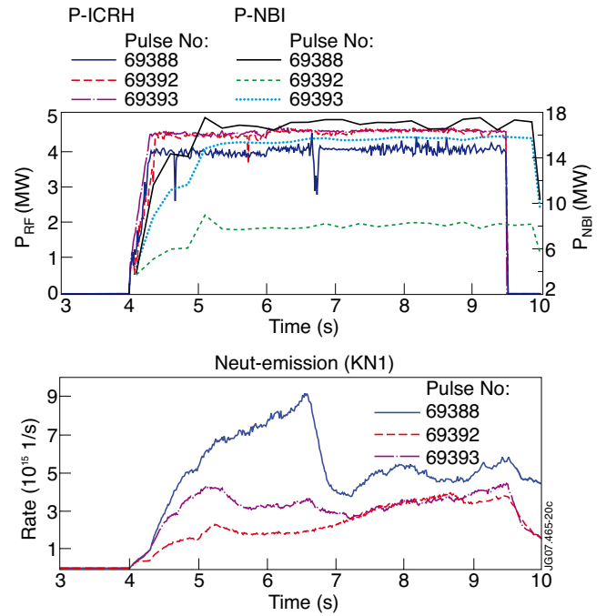
Figure 16: ICRH and NBI power (top) as well as neutron yield (bottom) as a function of time for shots 69388 (minority heating regime), 69392 & 69393 (mode conversion regime) .
