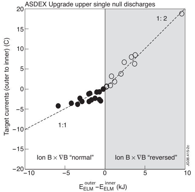
Figure 2: Correlation between the measured difference of ELM deposited energies towards inner and outer divertor target, E_{outer} - E_{inner} , with the ELM related charge difference C_{ELM} . Note that both values, E_{outer} - E_{inner} and C_{ELM} strictly change sign with field direction. Open symbols are 'reversed' field data and closed symbols 'normal field'.
