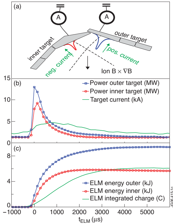
Figure 1: (a) Sketch of inner/outer ELM power load asymmetry and corresponding target current direction for ASDEX Upgrade Upper Single Null discharges with 'reversed' ion B \times \nabla B drift direction pointing away from the active (upper) X-point. (b) Power load for inner (red) and outer (blue) target plates and target current evolution during type-I ELM in ASDEX for coherently averaged data of about 20 ELMs. (c) Time integrals of the values in (b) over ELM duration in same colours.
