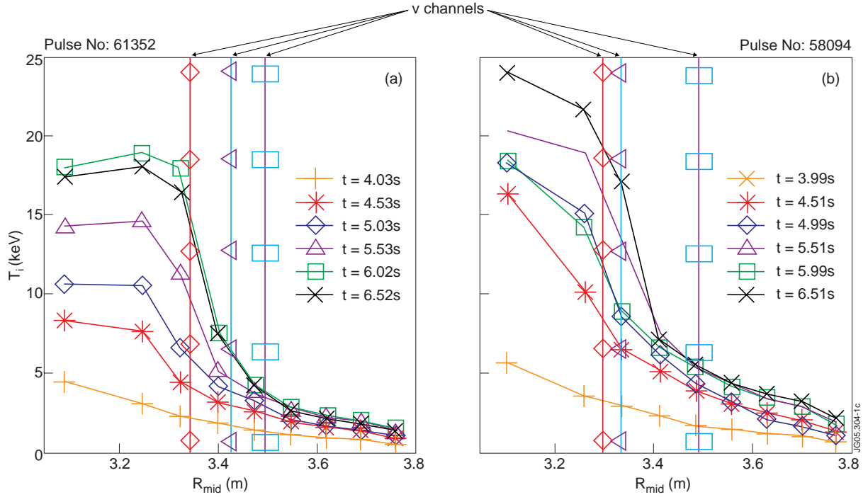
Figure 1: Radial T_i profiles during the evolution of the ITB for (a) Pulse No's: 61352 and (b) 58094. The vertical lines show the locations of the CXRS channels for v_\theta measurements.
