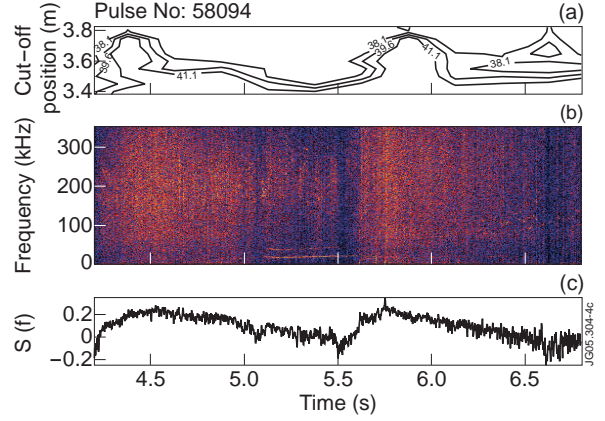
Figure 4: Reflectometry measurements of (a) radial position of the cut-off layer for three frequencies, (b) sliding FFT spectrogram of the reflected signal and (c) integrated spectrogram.
