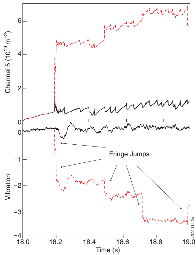
Figure 2: Comparison between uncorrected (red) and corrected (blue) density and vibration.
