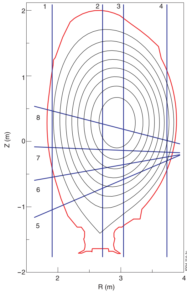
Figure 1: Lines of sight of the interferometric/polarimetric diagnostic at JET.
