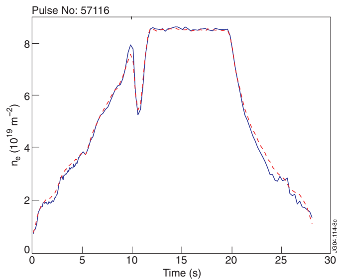
Figure 7: Density for channel 3 (red) compared with Cotton-Mouton measure (blue).
