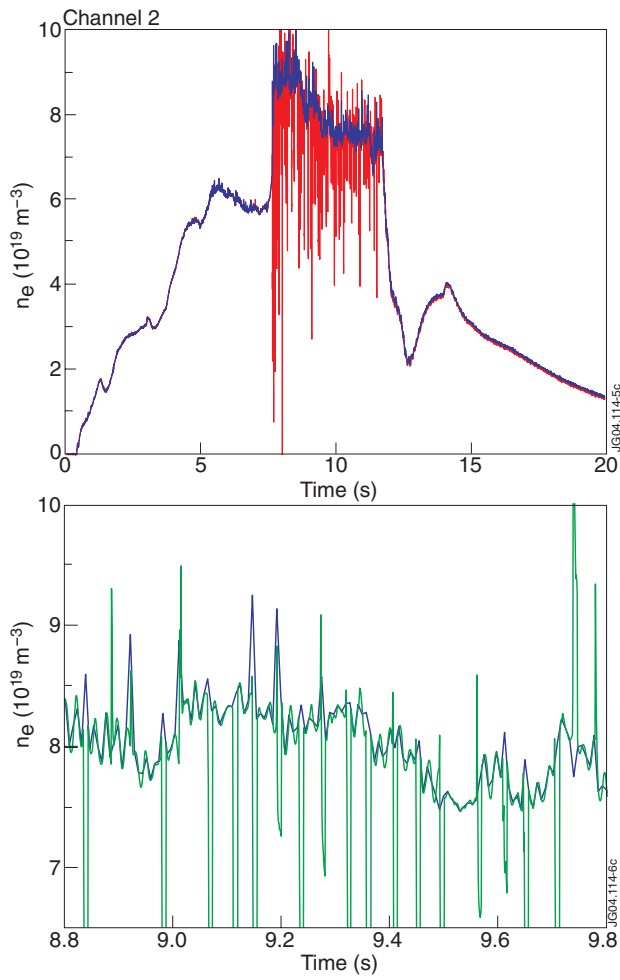
Figure 5: Corrected density for channel 2 (green line) compare to the offline density (blue line). Whole time evolution and one second detail.
