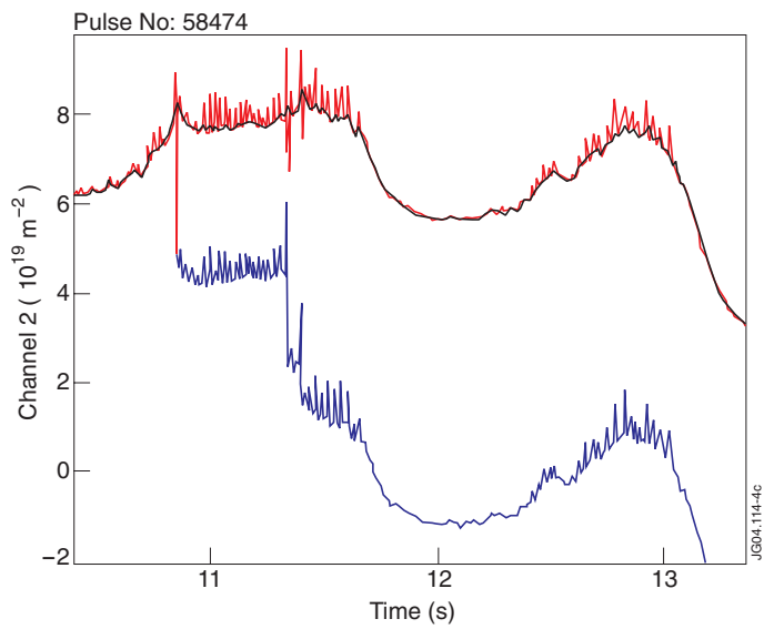
Figure 4: Plotting of the uncorrected (blue), reconstructed (red) and corrected (black) densities.
