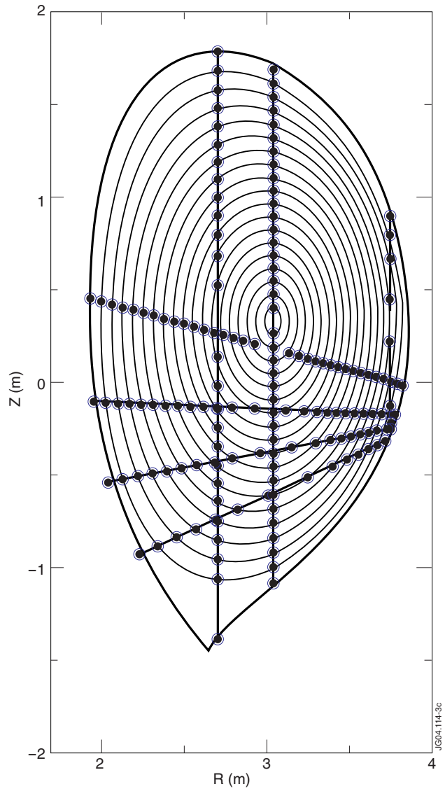
Figure 3: Iso-flux structure for the inversion of the interferometric data.
