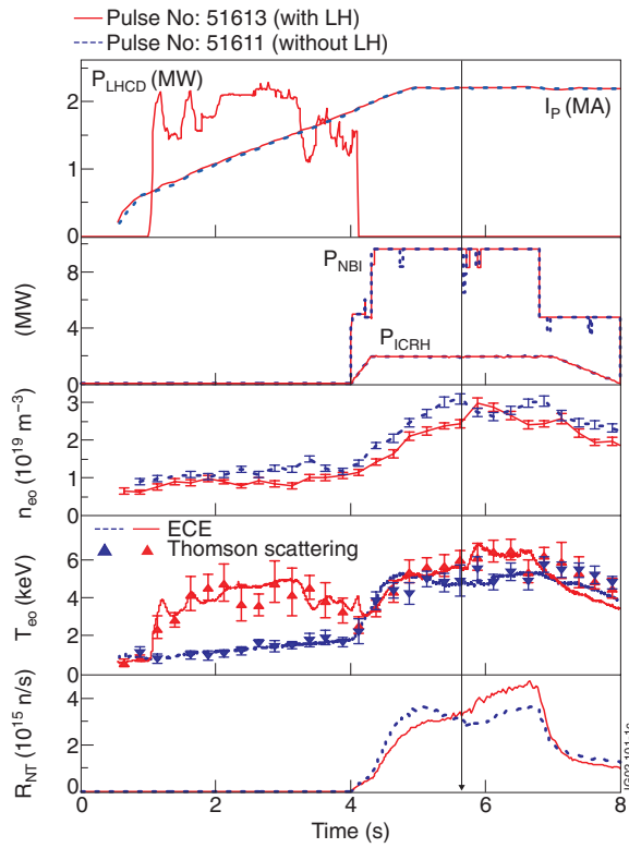
Figure 1: Overview of two JET discharges: Pulse No: 51611 without LH (---), and #51613 with LH (—). Plasma current and LH power (a); NBI and ICRF power (b); electron density (c); electron temperature (d); neutron rate (e).
