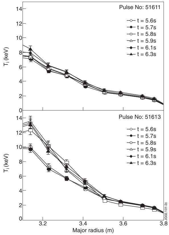
Figure 2: Ion temperature versus major radius at various times.
