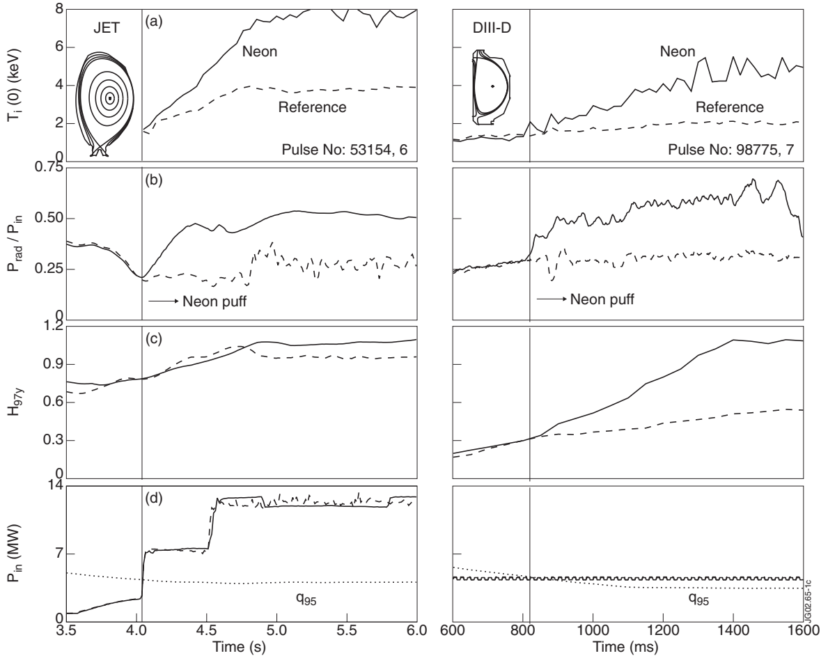
Figure 1: Temporal evolution of JET (left panels) and DIII-D (right panels) neon seeded discharges (Pulse No: 53154 and Pulse No:98775). Reference discharges are also shown (dashed lines, Pulse No: 53156 and Pulse No: 98777). Plotted are: (a) T_i(0) , (b) radiated power fraction, (c) H_{97y} confinement enhancement factor and (d) input power. Safety factor, q_{95} , is also shown in (d) as dotted lines. Ordinate scales are the same for both DIII-D and JET to allow a direct comparison. Discharge parameters are: (JET) I_p = 1.7\text{MA} , B_t = 2.2\text{T} , q_{95} = 4.1 , and (DIII-D) I_p = 1.2\text{MA} , B_t = 1.6\text{T} , q_{95} = 3.7 .
