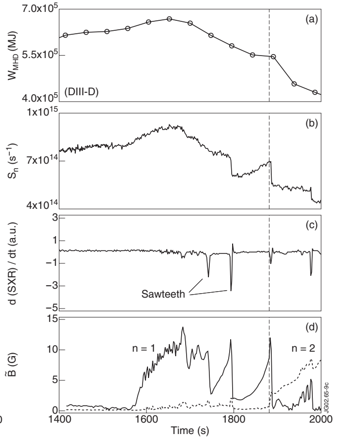
Figure 9: Stored energy (a) and the neutron rate (b) both decrease after the onset of sawteeth (c) and n=1 MHD activity (d) and further decrease after the onset of an m/n = 3/2 neoclassical tearing mode (dashed line) for a DIII-D neon seeded discharge (Pulse No: 98775).
