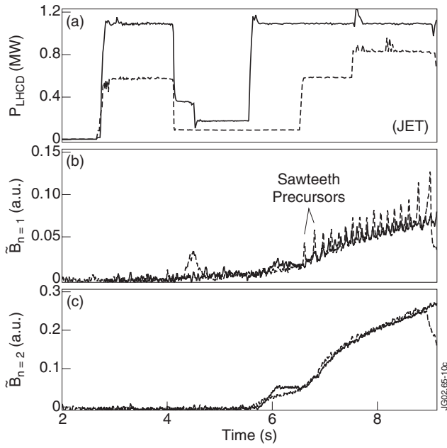
Figure 10: Plotted are: (a) LHCD power, (b) n=1 MHD amplitude and (c) n=2 MHD amplitude. The excursions in B_{n=1} are sawteeth precursors. Both neon seeded discharges (Pulse No: 52180, 52183) have similar parameters.
