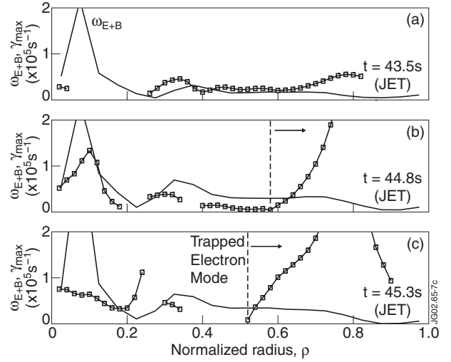
Figure 7: Maximum growth rate and calculated 'ExB' shearing rate for JET Pulse No: 53154 with neon seeding at three times: (a) 3.5s, (b) 4.8s, and (c) 5.3s. Vertical dashed lines in (b) and (c) indicated radius where the maximum growth rate is in the electron diamagnetic drift direction and higher k , indicating that electron effects are dominant.
