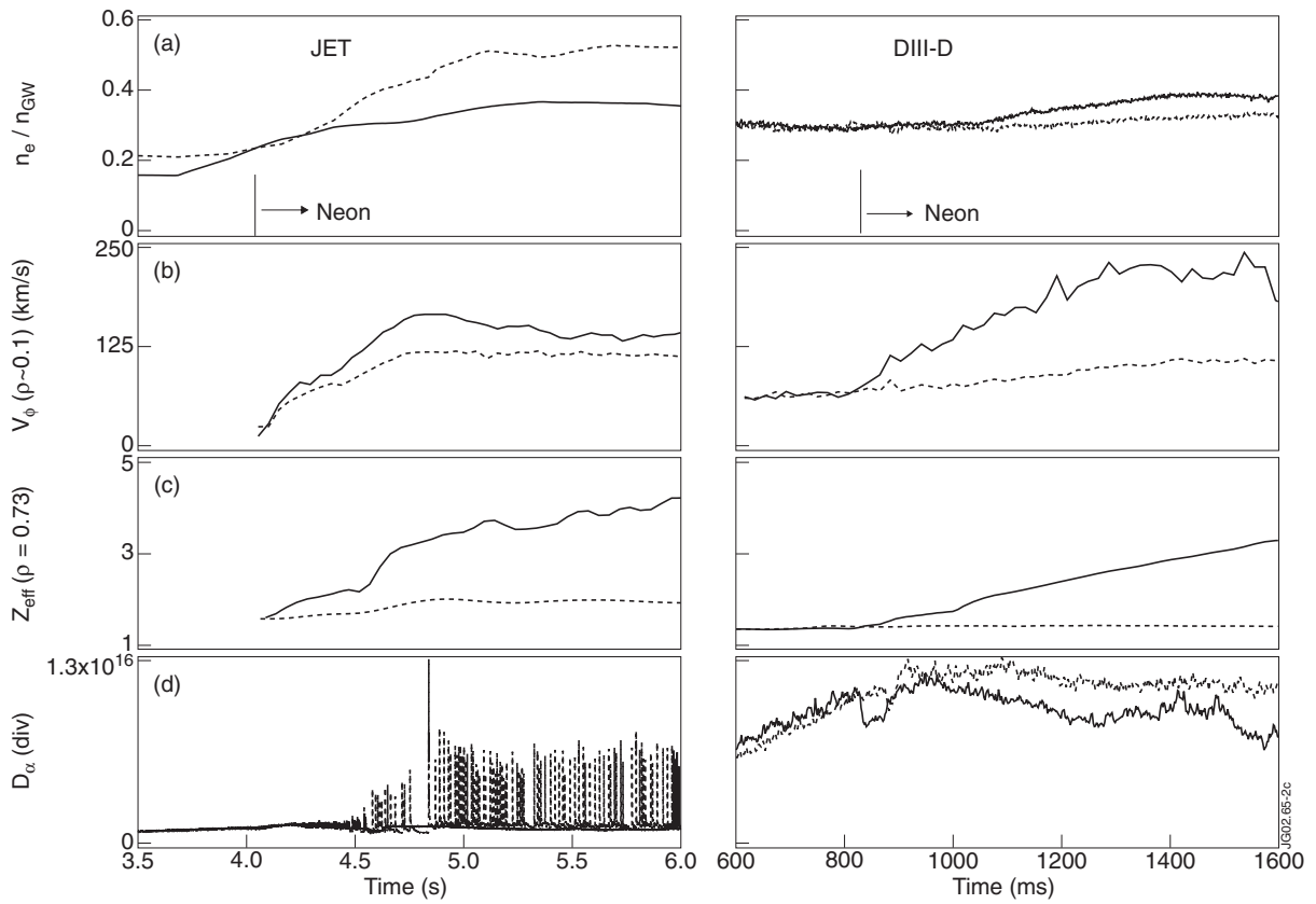
Figure 2: Plotted is (a) normalized density, (b) core toroidal rotation, (c) mantle Z_{\text{eff}} and (d) divertor deuterium line intensity ( D_{\alpha} ) for the same discharges as in Fig.1. Left panels are JET discharges and right DIII-D. Reference (no neon) discharges are shown as dashed lines.
