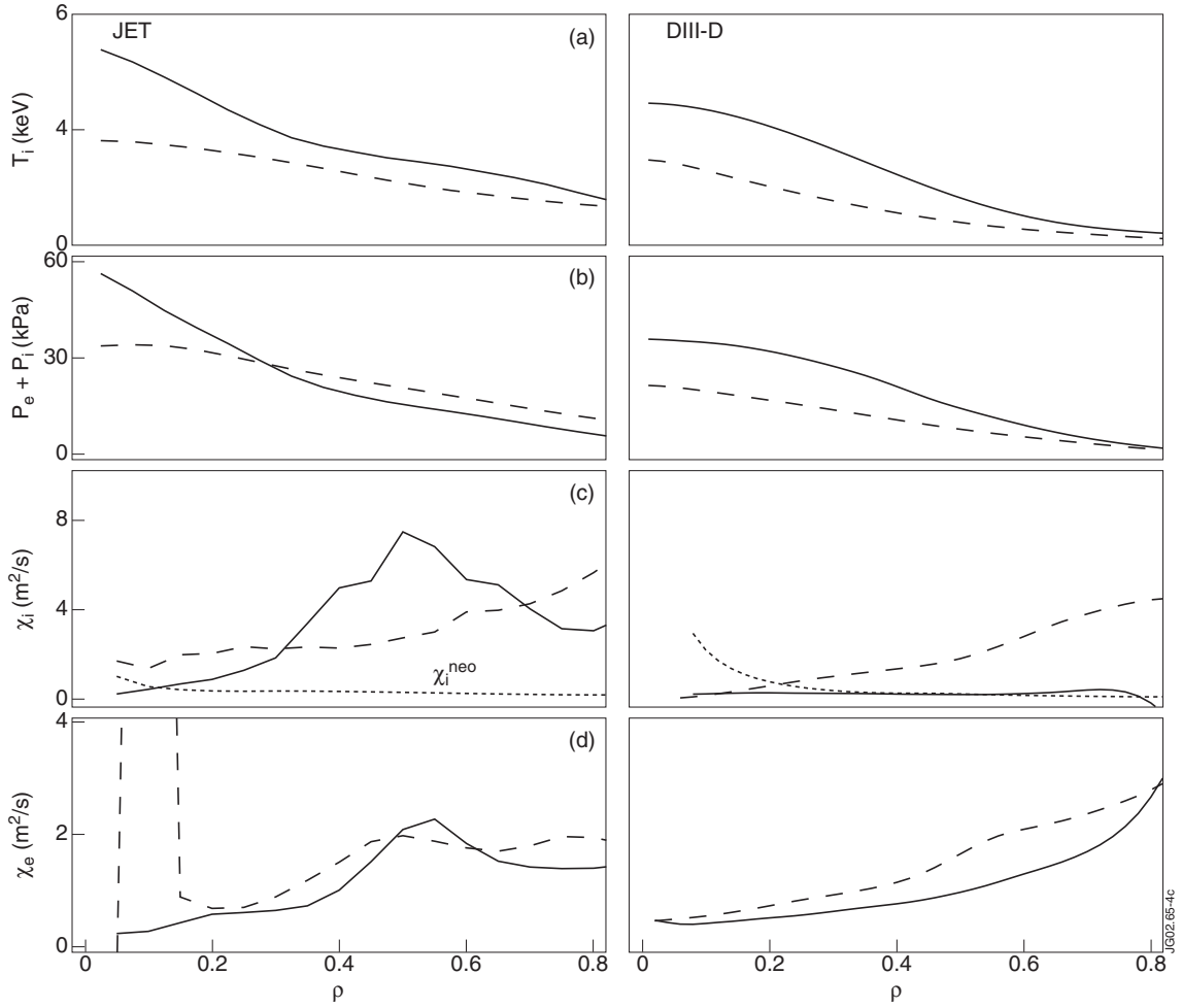
Figure 4: Profiles of (a) T_i , (b) plasma thermal pressure, (c) \chi_i , and (d) \chi_e for both JET (left panels) and DIII-D (right panels) at 4.8s (JET) and 1.16s (DIII-D). Ion neoclassical diffusivity is shown as a dotted line (c). Reference discharges (no neon) are shown as dashed lines. Discharges are the same in figure 1.
