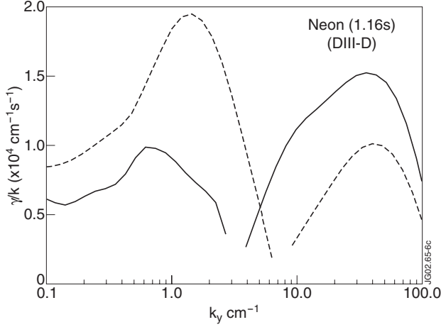
Figure 6: GKS calculated growth rates normalized to k as a function of wavenumber for a DIII-D seeded discharge (Pulse No: 98775, solid line) and a reference discharge (Pulse No: 98777, dashed line) at t = 1.16 s and \rho = 0.64
