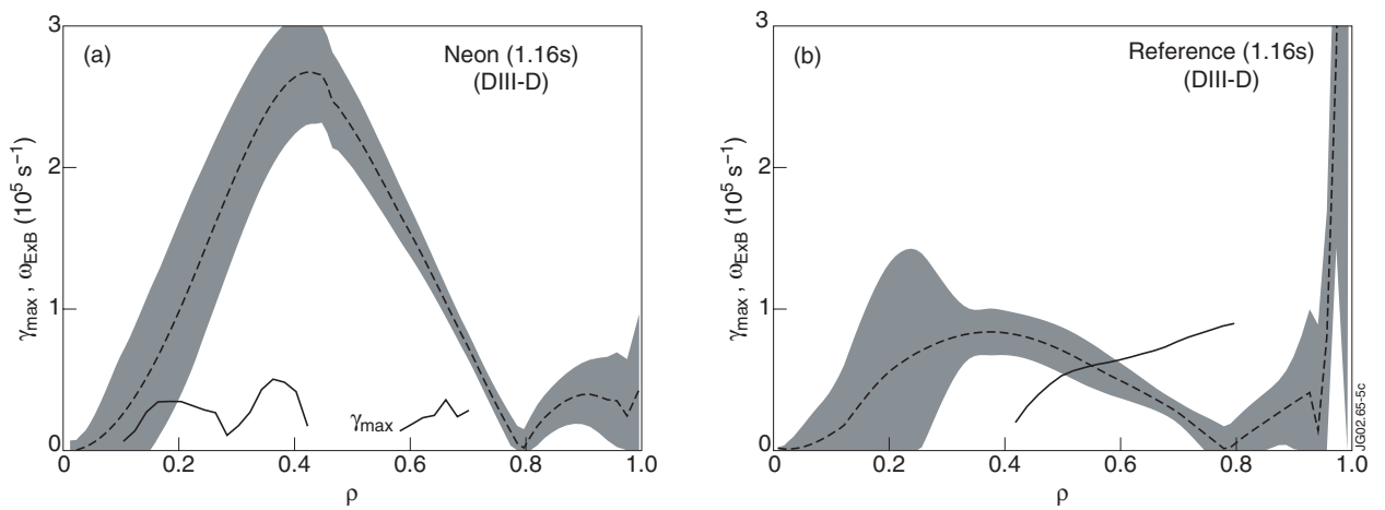
Figure 5: Maximum growth rates and E×B shearing rates for DIII-D discharges with (a) and without (b) neon seeding at 1.16s. DIII-D discharges are the same as in figures 1 and 2.
