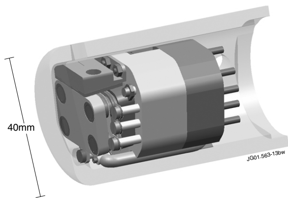
Figure 4: Engineering and assembly of the PIMS probe head.
