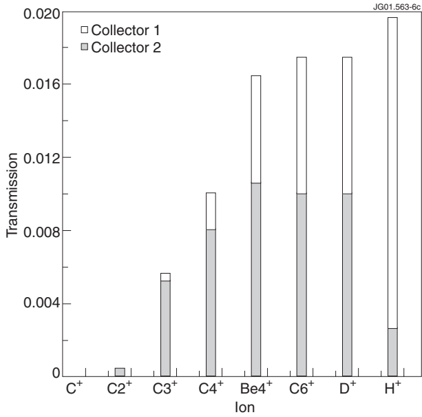
Figure 8: Peak transmission for different charge states of carbon for the base case.
