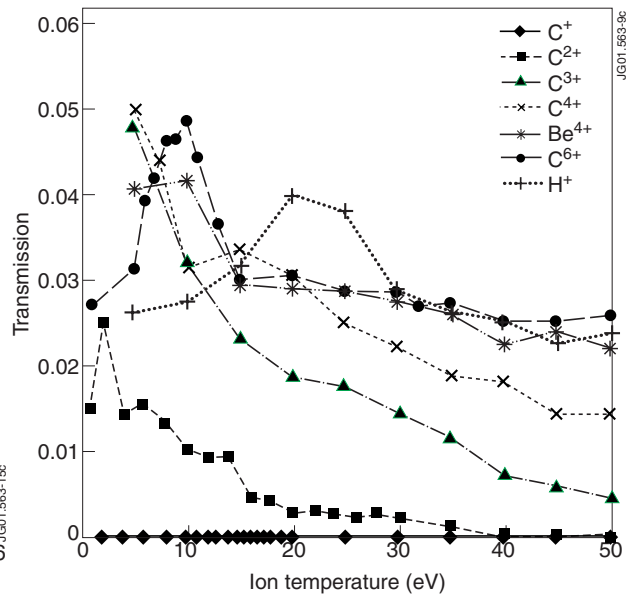
Figure 11. Variation of total transmission with ion temperature for a fixed sheath voltage of 100V.
