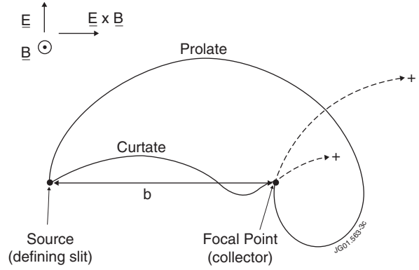
Figure 2: In perpendicular electric and magnetic fields ion orbits are cycloidal and the focussing properties are perfect [5].
