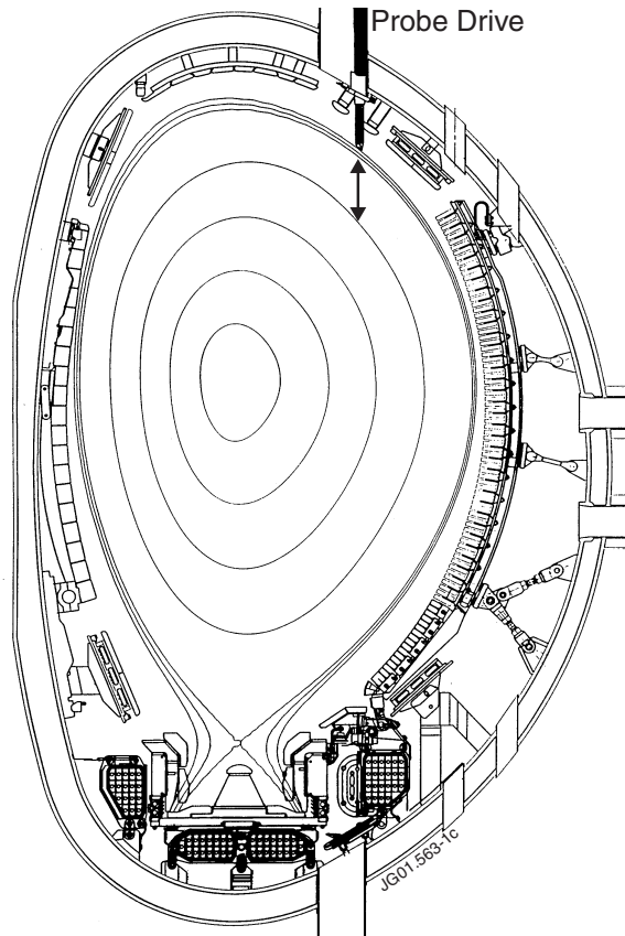
Figure 3: Cross-section of the JET torus and plasma showing the location of the reciprocating probe head.
