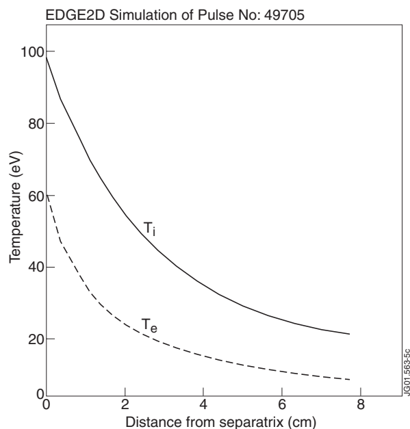
Figure 6: Ion temperature and electron temperature as predicted by EDGE2D-U/NIMBUS for pulse 49705 which is an L-mode plasma with 2.5MA of plasma current, 2.5T toroidal field and 2MW of neutral beam heating.
