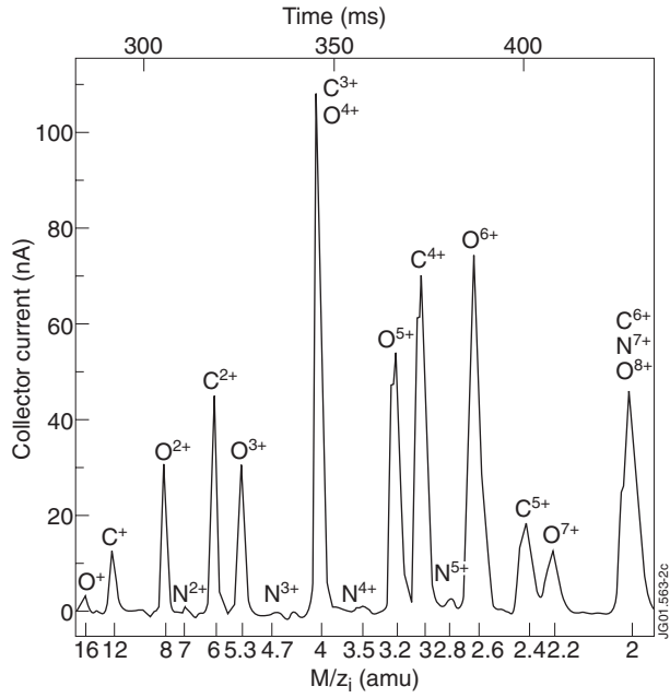
Figure 1: Mass-spectrum from a plasma ion mass-spectrometer (PIMS) in the edge plasma of the DITE tokamak [2]. M is the atomic mass of the ion and z_i its charge state. The electric field in the PIMS ramped up linearly with time, top axis, to sweep the various ion species across the collector during steady state phase of the plasma discharge.
