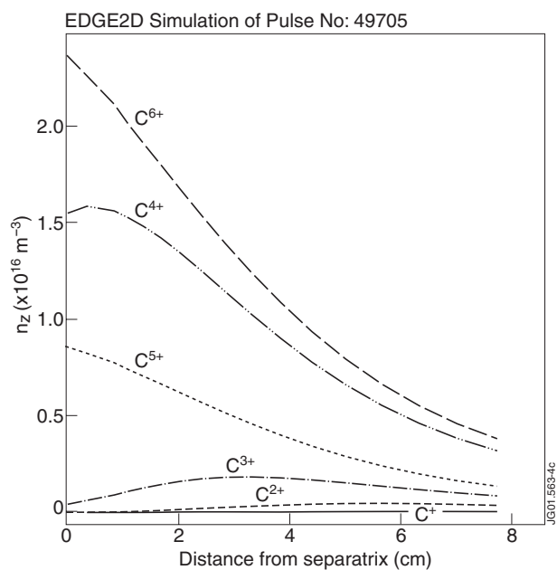
Figure 7: Charge state distribution predicted by EDGE2D-U/NIMBUS for JET pulse 49705.
