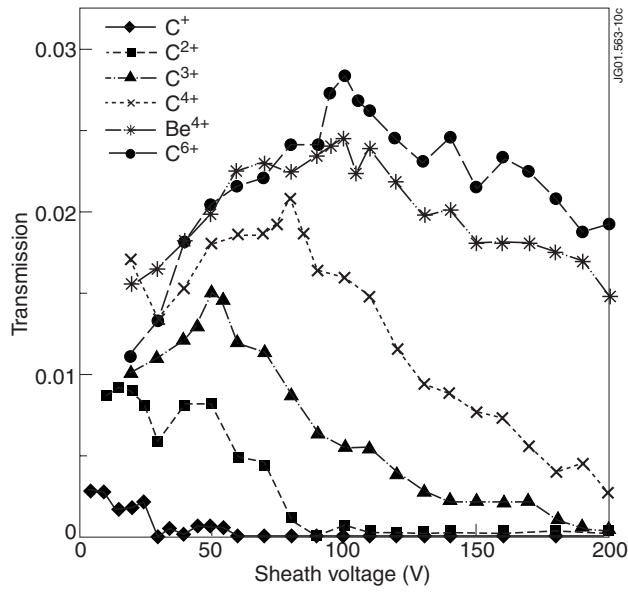
Figure 12. - Variation of total transmission with sheath voltage for an ion temperature of 50eV.
