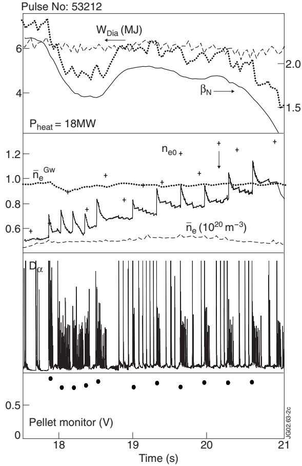
Figure 2: Optimised pellet refueling for high performance high density operation. \bar{n}_e > \bar{n}_e^{GW} is achieved at the energy content of an unfueled reference discharge (dashed lines) as energy recovers after the initial pellet sequence. Diamagnetic plasma energy and normalised pressure: first box; line averaged and Greenwald density (lines) as well as central density (crosses): second box; D_\alpha radiation signal from the outer divertor region monitoring ELMs: third box; microwave pellet mass detector signal: fourth box.
