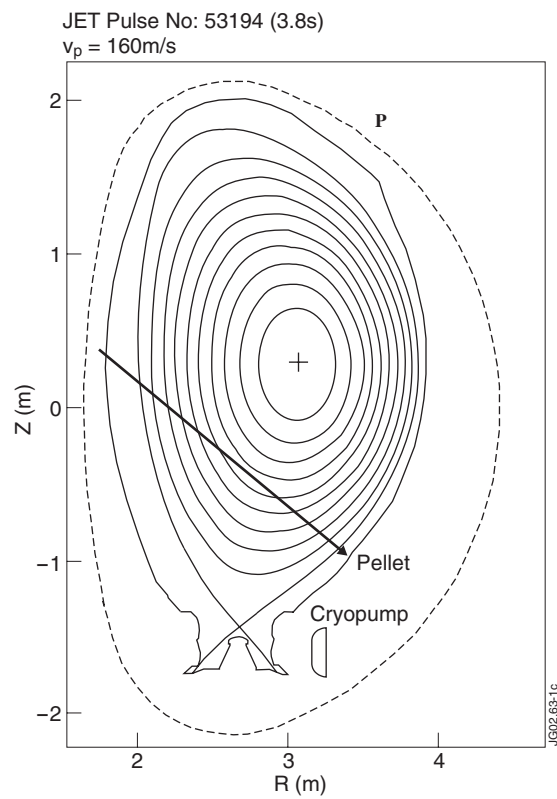
Figure 1: Poloidal cross section of JET with Mark II gas box divertor and central septum; magnetic structure of used lower single null plasma configuration with I_p = 2.5\text{MA} , B_t = 2.4\text{T} , q_{95} = 3.2 ; \langle \delta \rangle \approx 0.34 and strike zone deep in divertor throat for efficient pumping. Used designated pellet injection path from the HFS (max. launch speed v_p = 160\text{ms} )
