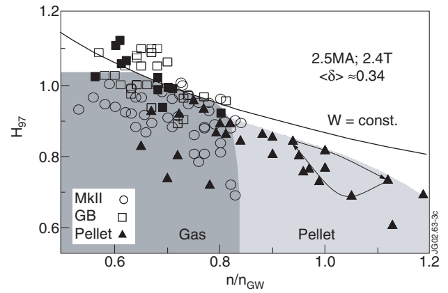
Figure 3: Extension of accessible operational area for 2.5MA/2.4T HT plasma configuration by pellet refueling visualized in a f^{GW} - H_{97} plot. Values from JET data base for MkII (open circles) and current gas box (open squares) as well as from reference shots (filled squares) included. Pellet refueling (filled triangles) allows high density operation at elevated confinement level.
