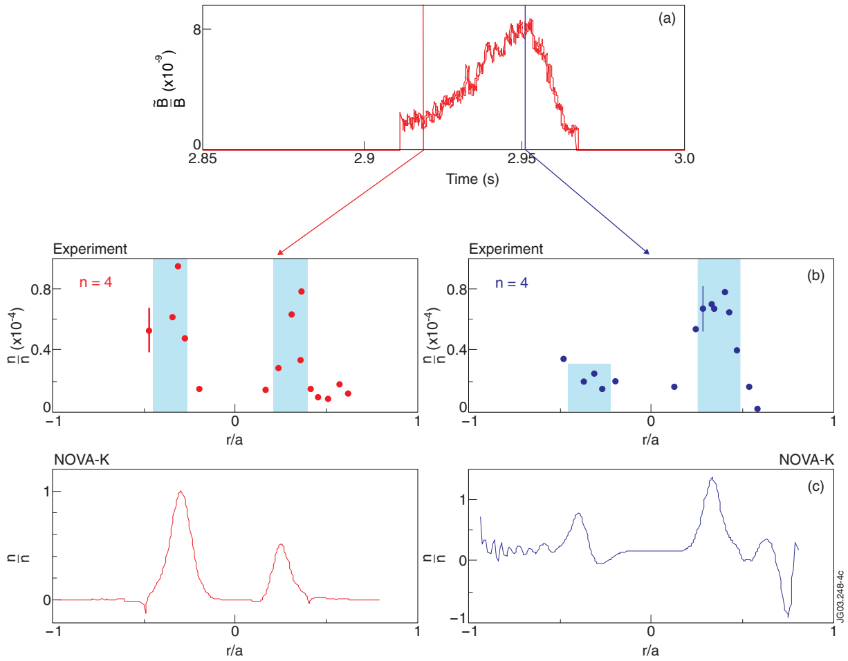
Figure 4: Time evolution of edge magnetic fluctuations for the n=4 mode in Figure 2 (a). The radial density fluctuation profile using the reflectometer diagnostic is shown in (b) early (left) and later (right) in time, and radial density eigenmode expected for the n=4 Cascade mode (left) and TAE (right) in (c).
