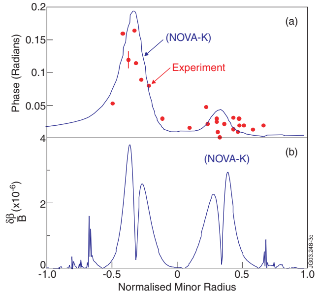
Figure 3: Measured radial structure of density fluctuations (a) for the n=2 mode in Figure 2 compared to the theoretically expected radial mode structure for the n=2 Cascade mode according to the NOVA-K code. In (b) the magnetic fluctuation level |\delta B|/B from NOVA-K is also shown, indicating the cylindrical nature of the mode from the near equal amplitude on the high and low field side of the magnetic axis.
