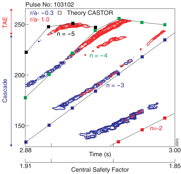
Figure 2: Contour plot of edge magnetic measurements (red) and core density fluctuations using an X-mode reflectometer (blue) for the discharge in Figure 1. The reflectometer measurements are located at a normalized minor radius of -0.3 . Also indicated is the range of expected mode frequencies for TAEs and the range of mode frequency expected for Cascade modes. Rectangles indicate CASTOR code calculations of the mode frequency expected for Cascade modes using the measured plasma equilibrium and evolving the central safety factor over a narrow range near q=2 .
