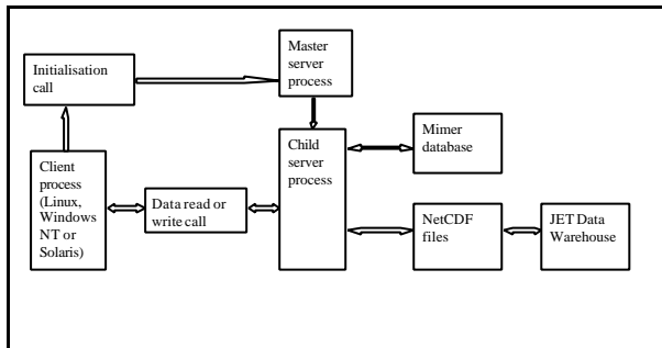
Figure 1: Interaction between components of the PPF system
