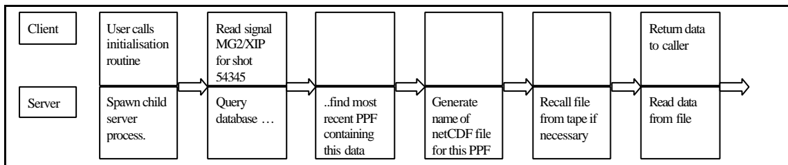
Figure 2: Typical read transaction
