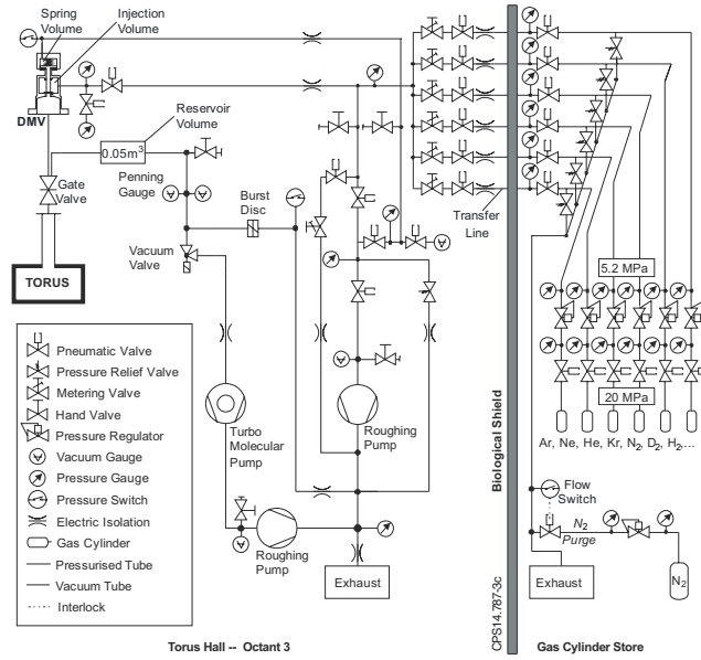
Figure 3: Schematic of the new DMS Gas Handling System.
