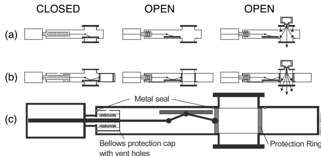
Figure 2: Illustration of the all metal gate valve compatible with high pressure injections. (a) Normal gate valve and (b) special gate valve in closed-open state and in the case of a gas injection through the open gate valve. (c) Special gate valve key design features.
