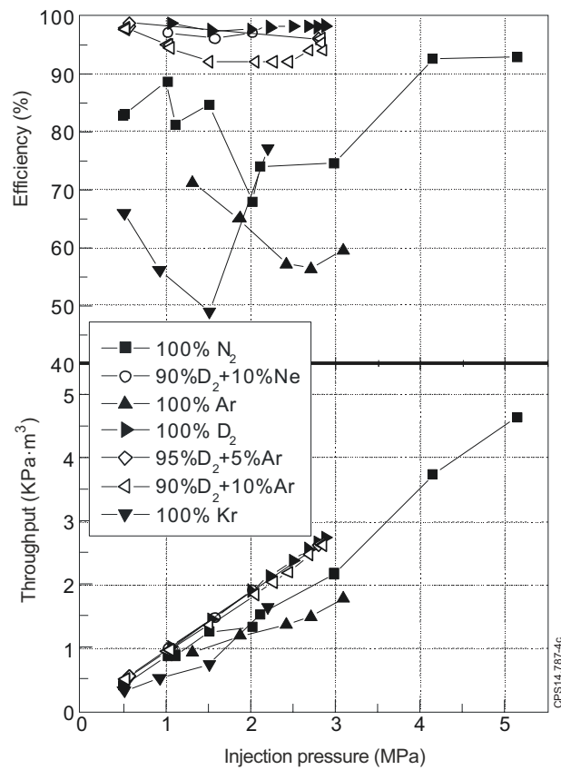
Figure 4: Valve throughput and efficiency (Pressure drop/charging pressure) for DMV2 at various injection volume pressures.
