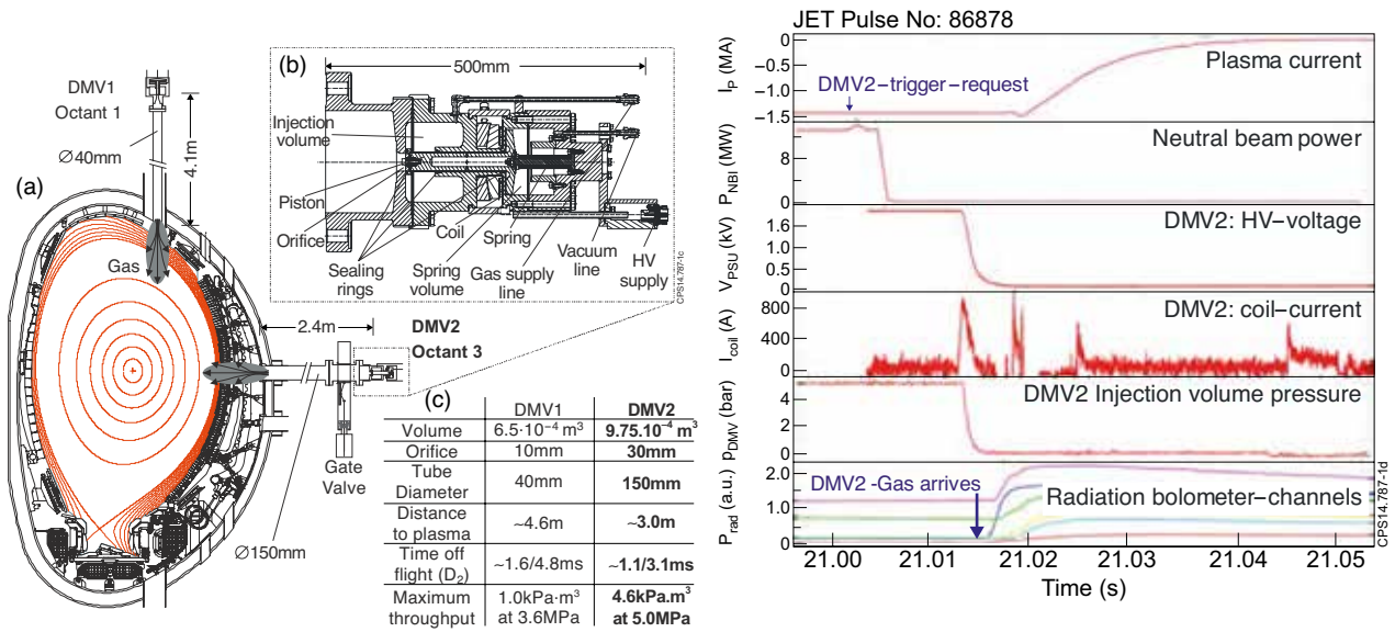
Figure 1: (a) Poloidal cut of JET presenting the JET DMS. The two Disruption Mitigation Valves (DMV) are projected into the same poloidal plane. Their physical positions are on top of the machine in octant 1 (DMV1) and at a horizontal position in octant 3 (DMV2). Both systems are located 90^\circ toroidally apart. (b) Technical drawing of the new DMV (DMV2). (c) Characteristic properties of the two DMS. (d) Typical DMV2 sequence (JET Pulse Number: 86878, B_t = 1.5 \text{ T} , I_p = 1.5\text{MA} , Auxiliary heating: 14MW NBI, DMV request time: 21.0s, Total injected gas: 0.5\text{-kPa m}^3 of 10% argon and 90% deuterium mixture, Time of flight: \sim 1.5\text{ms} , Total radiated energy fraction is about 92% (not considering radiation asymmetry effects)).
