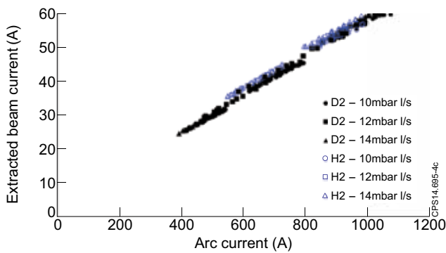
Figure 4: (Colour online). Extracted positive ion current for PINI 5E2T in hydrogen and deuterium at different source gas flow rates with a neutraliser gas flow rate of 20mbar l/s.
