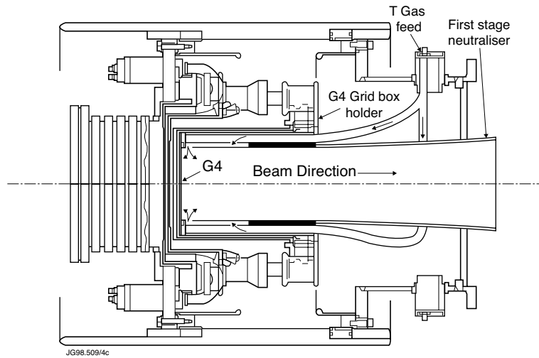
Figure 2: Horizontal section of a JET PINI showing the grid gas introduction at the earth grid (G4 in this case).
