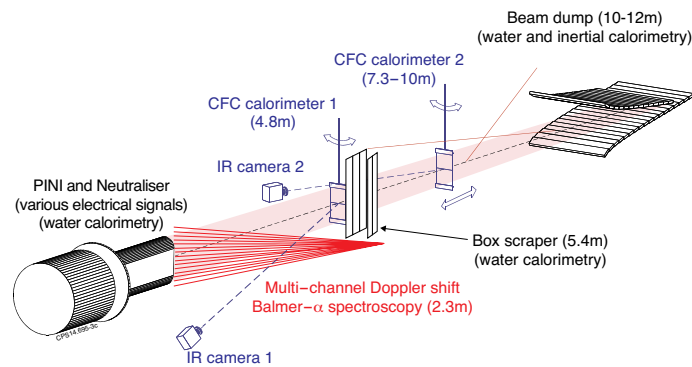
Figure 3: (Colour online). The JET Neutral Beam Test Bed
