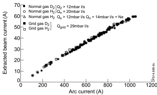
Figure 6: Extracted positive ion current for three PINIs in both normal and grid gas operation for various source gas, Q_s , neutraliser gas, Q_n and grid gas Q_{grid} flow rates.
