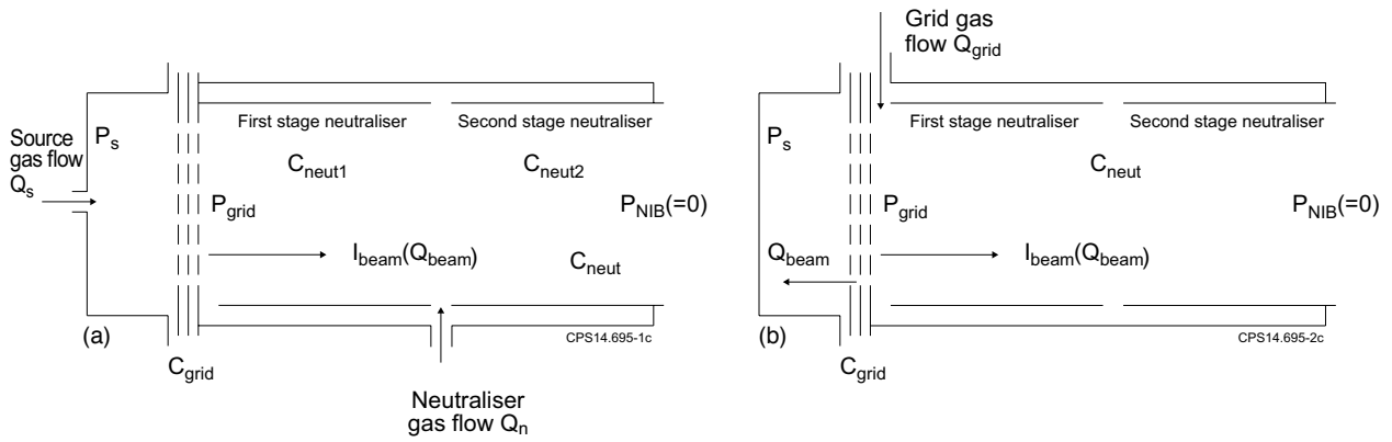
Figure 1: Schematic of the gas flows and pressures in (a) normal gas operation (b) grid gas operation.
