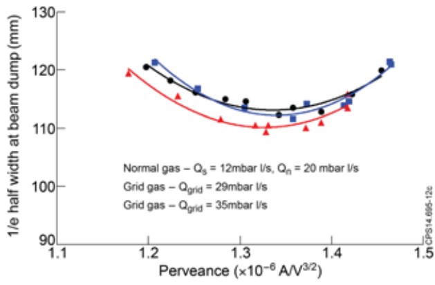
Figure 8: (Colour online). Perveance curves for deuterium operation in normal and grid gas modes.
