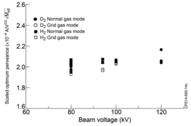
Figure 9: Optimum perveance for hydrogen and deuterium operation in normal and grid gas modes.
