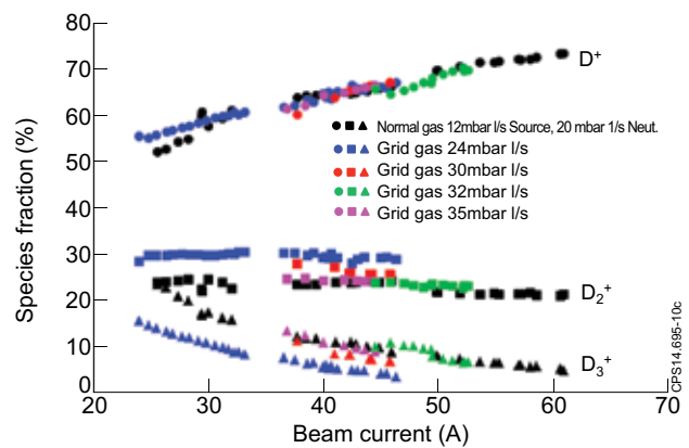
Figure 7: (Colour online). Species flux fractions in deuterium normal gas and grid gas operation.
