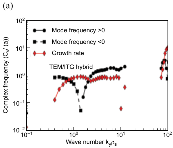
Figure 3: (a) Microturbulence modeling for L-mode phase before injection of neutral beam power ( t = 3.2s ) made by the GENE code. Pulse No: 72595. ETG is absent.
