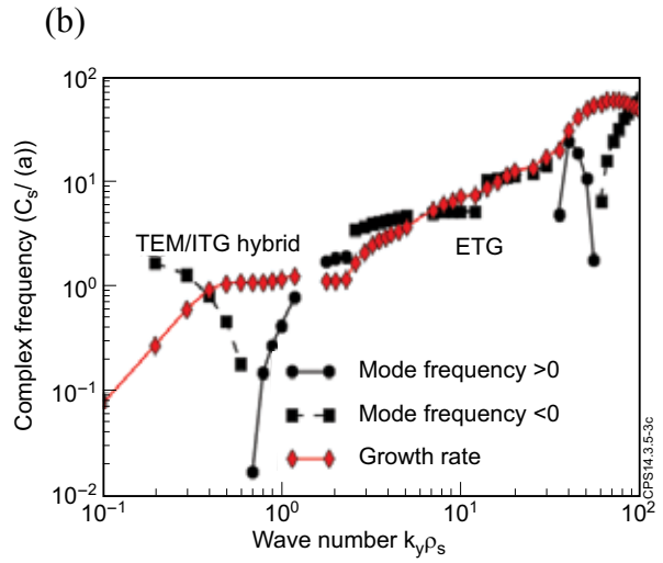
Figure 3: (b) Simulations as in Fig.3a but considering plasma parameters of Pulse No: 70068. In this case ETG takes over at higher wavenumber.
