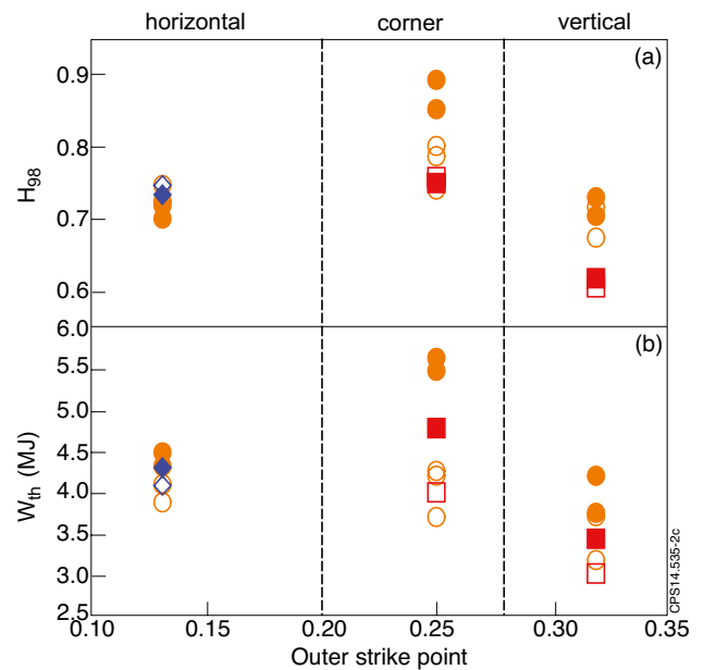
Figure 2. H_{98} (a) and thermal energy (b) versus outer strike position. Red symbols: high \Gamma_{D2} ( \approx 3.5 \cdot 10^{22} e/s). Orange symbols: medium \Gamma_{D2} ( \approx 2 \cdot 10^{22} e/s). Blue symbols: low \Gamma_{D2} ( \approx 1.4 \cdot 10^{22} e/s). Open symbols: low power phase. Full symbols: high power phase.
