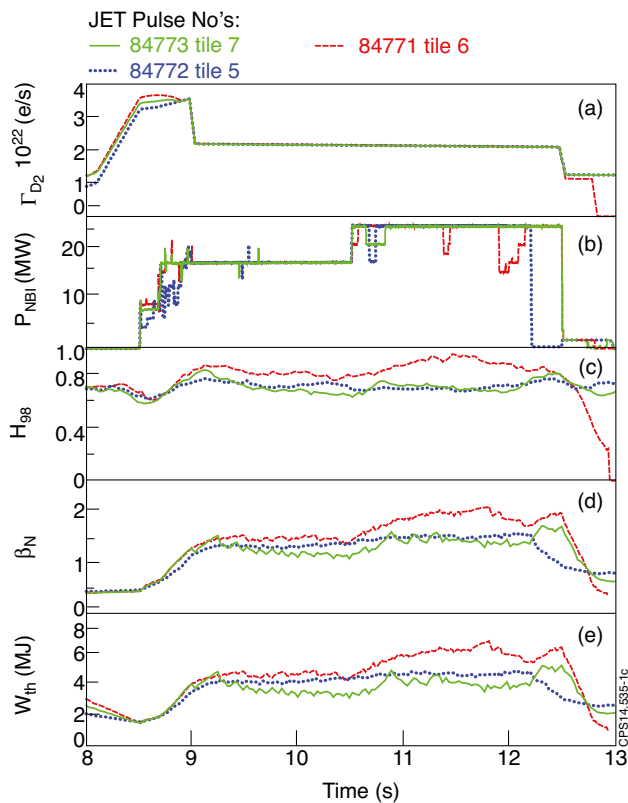
Figure 1. Time traces of gas fuelling (a), NBI power (b), H_{98} (c), \beta_N (d) and thermal stored energy (e) for three shots with different outer strike point position.
