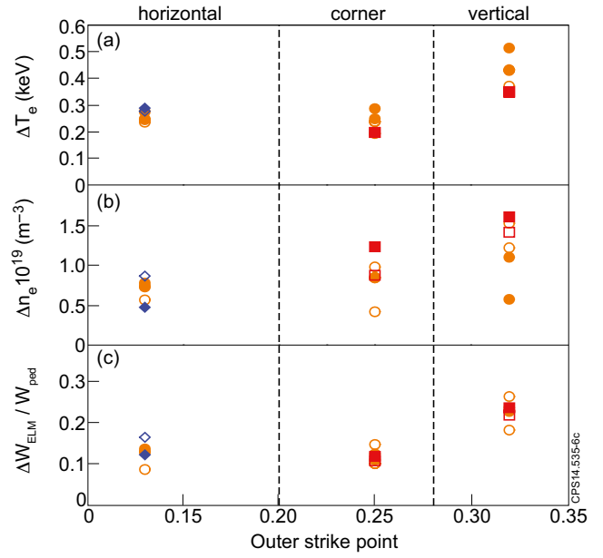
Figure 6. ELM temperature drops (a), density drops (b) and relative ELM energy losses (c).
