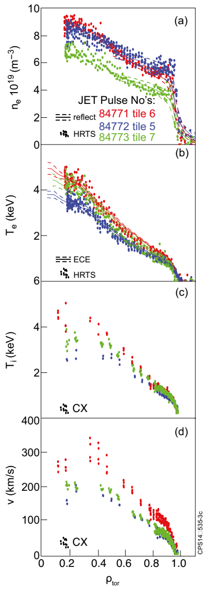
Figure 3. Profiles of electron density (a) electron temperature (b) ion temperature (c) and toroidal velocity (d) in the pre-ELM phase.
