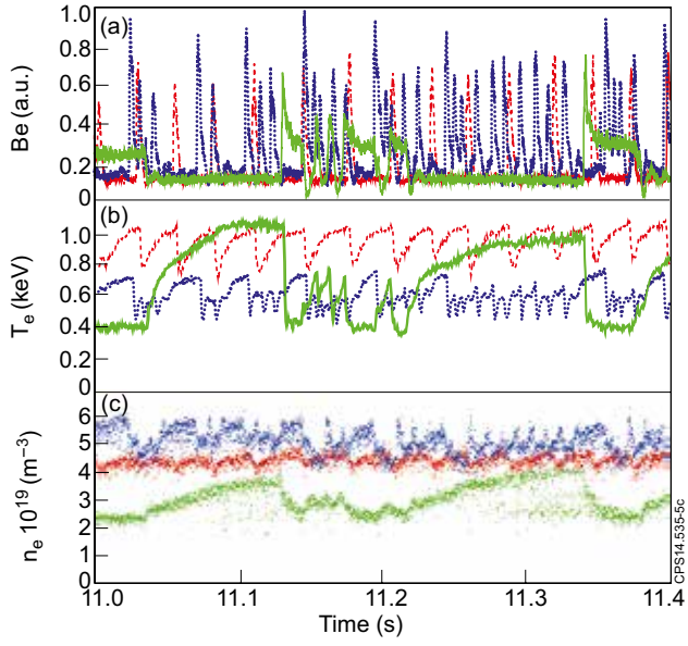
Figure 5. Time traces of Be signal from the outer divertor (a), electron temperature (b) and density (c) for the shots of figure 1 in a 0.4s time interval during the high power phase.
