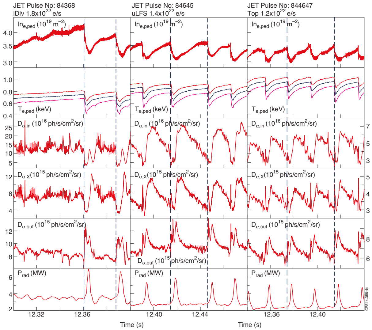
Figure 3b) time zoom to show negative ELMs.
