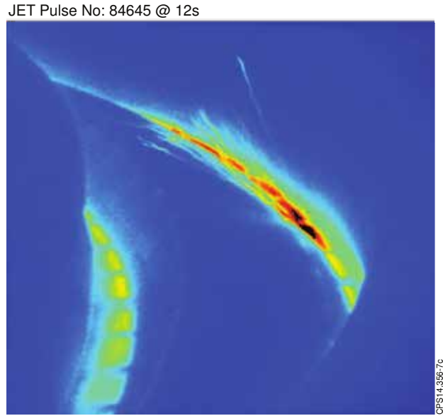
Figure 5: shower of W sparks originating near the outer strike point, following a combined sawtooth and ELM event, responsible for triggering radiation increase and T_{e,ped} drop at 12s in Pulse No: 84645, shown in Figure 4.
