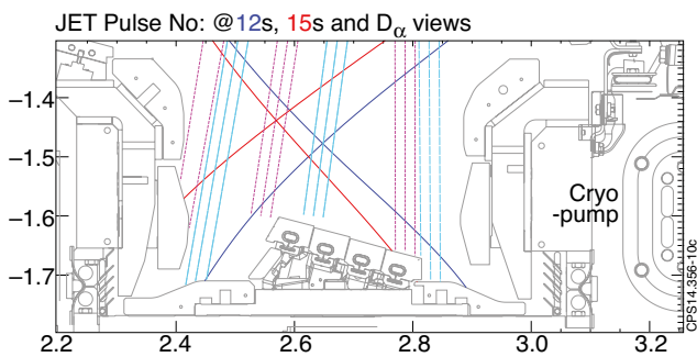
Figure 1.: Blue and Red plasma shapes studied and D_\alpha lines viewing inner strike, X-point and outer strike.
