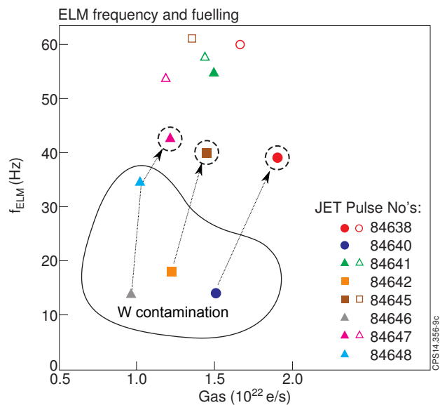
Figure 2: ELM frequency achieved for different fuelling levels and locations. Solid symbol for blue shape, open for red.
