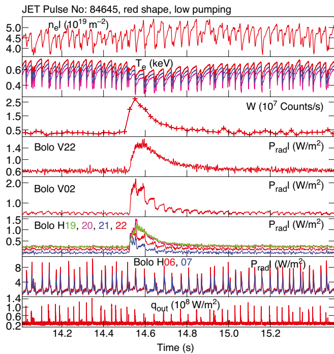
Figure 6: effect of W influx on pedestal.
