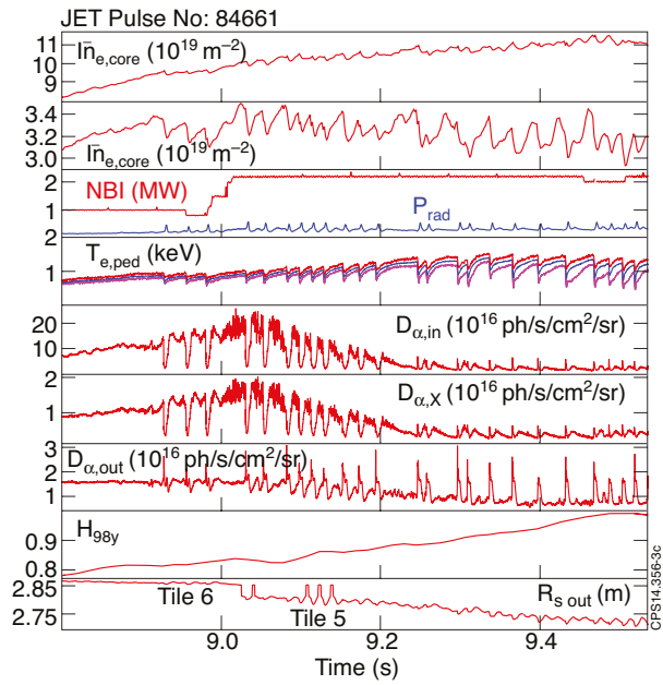
Figure 4: evolution of D_{\alpha} from negative to positive ELMs, together with change in T_{e,ped} .
