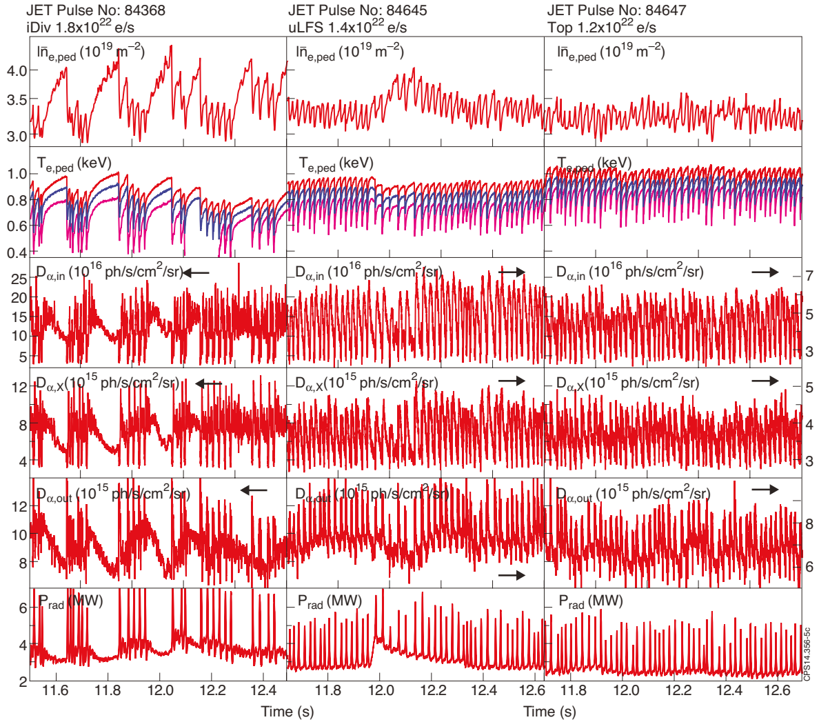
Figure 3a) for blue shape and divertor, upper LFS and top fuelling: pedestal density, temperature, D_{\alpha} from inner strike, X-point and outer strike views, total radiation.
