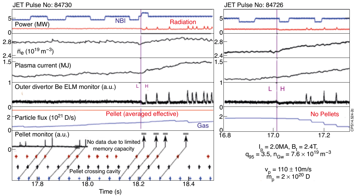
Figure 2: Demonstration of ELM control at JET by pellet pacing while the plasma undergoes the L \rightarrow H transition. The reference discharge (JET Pulse Number: 84726, right) with pure gas fuelling shows a delay of about 110ms between entering the H-mode and the first ELM. Applying partial pellet fuelling (Pulse Number: 84730, left) results in a slightly higher density in the L - Mode phase due to better fuelling efficiency. In the H-mode phase a similar fuelling efficiency as in the gas reference is found but now every pellet triggers an ELM and the ELM free phases is avoided. The first ELM is triggered in a still almost L - Mode like pedestal. Due to the higher density in the pellet case, the L \rightarrow H transition occurs later and the pre-set timed pellet monitor run out of data memory. Pellet arrival in the plasma is estimated (uncertainty represented by the grey bars) from a time-of-flight analysis of the pellets passing through several cavities installed along the flight tubes, as shown in the lower box. Note the speed scatter resulting in a distorted pellet train frequency and the gap due to a pellet obviously destroyed in flight.
