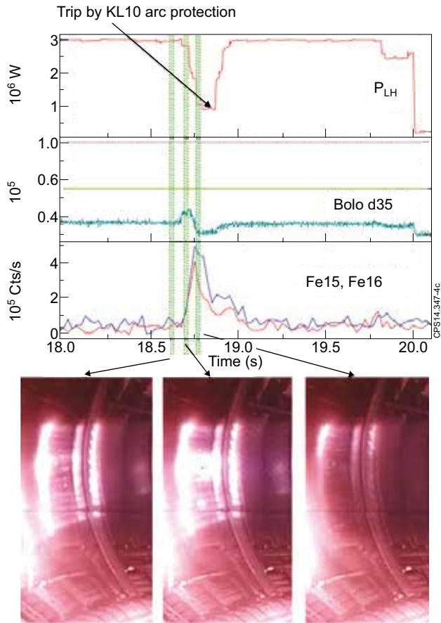
Figure 4: LH antenna as viewed by wide angle visible camera. Consecutive frames show arc imaging protection system in operation. The detection of an arc precursor on the second frame leads to a local reduction in the power and avoidance of arc event.
