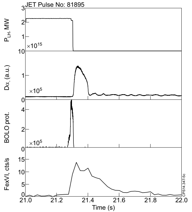
Figure 5: Evolution of an arc event as seen from a visible camera in consecutive frames, acquired at 20ms rate, showing how it develops into a flare. On the right, the time traces of the LH power, D_{\alpha} signal, bolometer protection and FeXVI line are shown.
