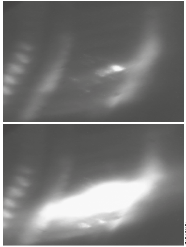
Figure 2: Two consecutive frames (20ms acquisition rate) of LH antenna protection camera show evolution of uncontrolled arc event. On the first frame an arc precursor is visible which develops into a flare on the second frame. In order for the protection system to act locally a grid of 24 ROIs was defined (Fig.3). Each ROI covers one klystron.
