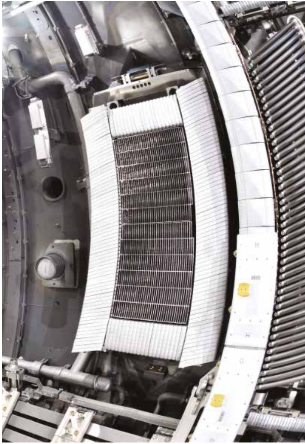
Figure 1: JET LH Antenna as imaged by visible camera. Low field side limiter is seen to the side of the antenna.
