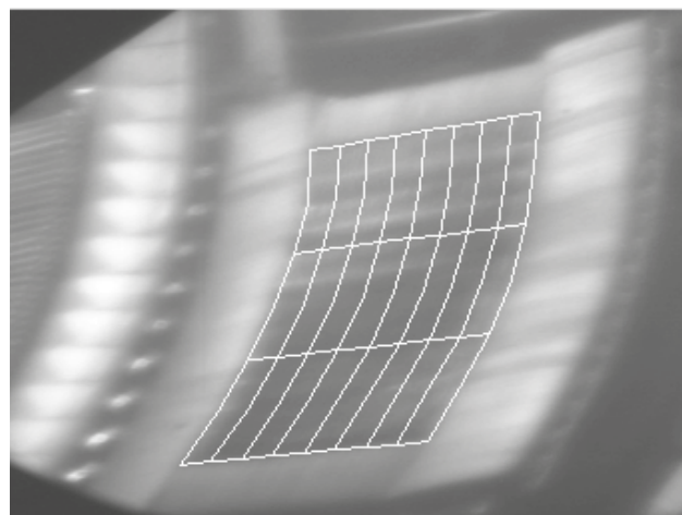
Figure 3: JET LH Antenna showing overlaid schematic representation of ROIs.
