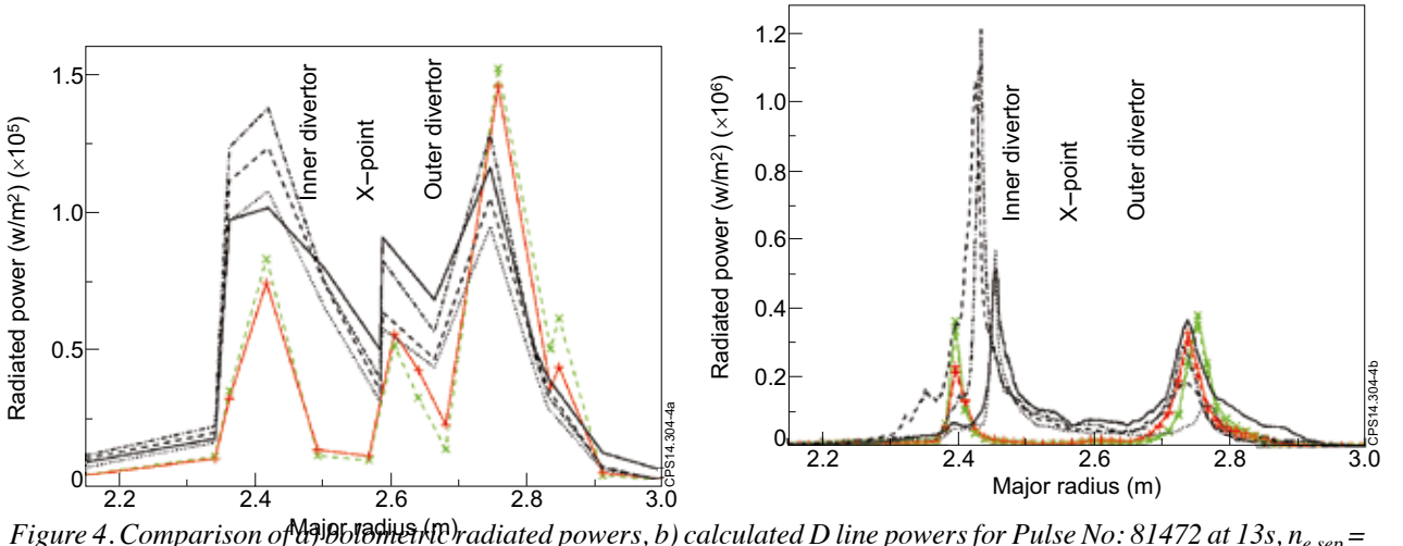
Figure 4. Comparison of a) bolometric radiated powers, b) calculated D line powers for Pulse No: 81472 at 13s, n_{e,sep} = 1.5 \times 10^{19} m^{-3} . Measured data (4 curves) without symbols (bolometric powers 1.3 \times 10^4 W/m^2 core emission subtracted). Simulated data + no drifts 2.2MW power to SOL, \times no drifts 2.8MW power to SOL. Simulated D line powers — total, ---- without D radiative recombination and ..... also without D molecular component.
