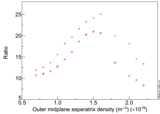
Figure 1. Ratio of simulated Ly_\alpha to Ly_\beta emission integrated along the spectrometer line-of-sight with the profile averaged over the inner divertor ( R = 2.31\text{--}2.53\text{m} , +) and outer divertor ( R = 2.53\text{--}2.94\text{m} x). Power to SOL in the simulations is 2.2MW.
