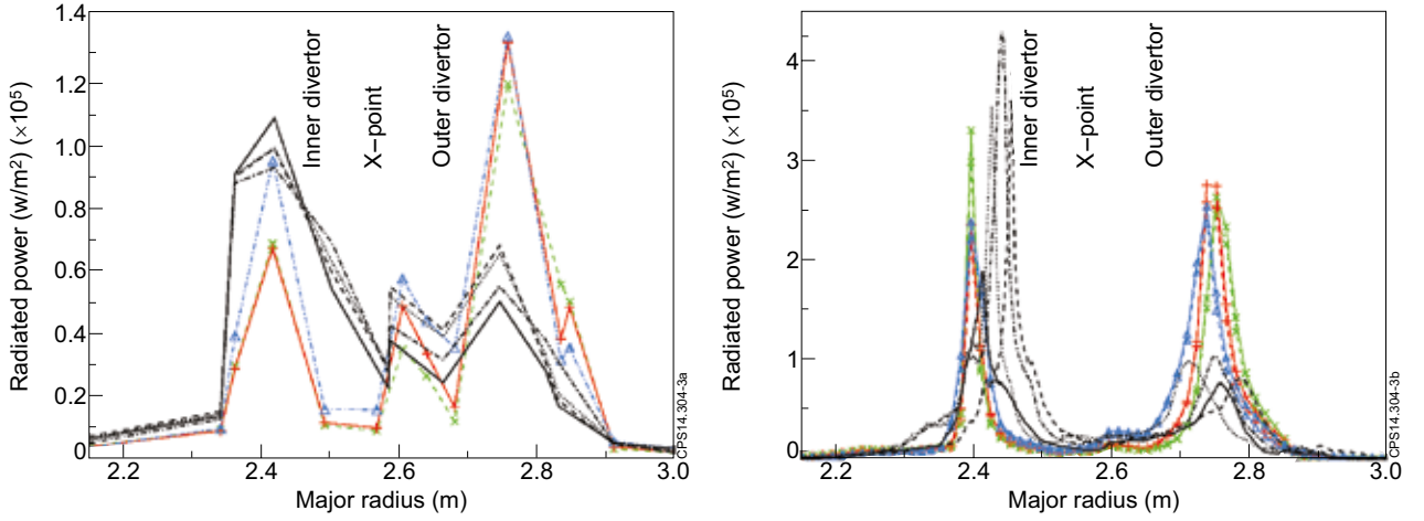
Figure 3. Comparison of a) bolometric radiated powers, b) calculated D line powers for Pulse No: 81480 at 17s, n_{e,sep} = 1.4 \times 10^{19} m^{-3} . Measured data (4 curves) without symbols (bolometric powers 1.3 \times 10^4 W/m^2 core emission subtracted). Simulated data + no drifts, \Delta with drifts 2.2MW power to SOL, \times no drifts 2.8MW power to SOL. Simulated D line powers — total, ---- without D molecular component.
