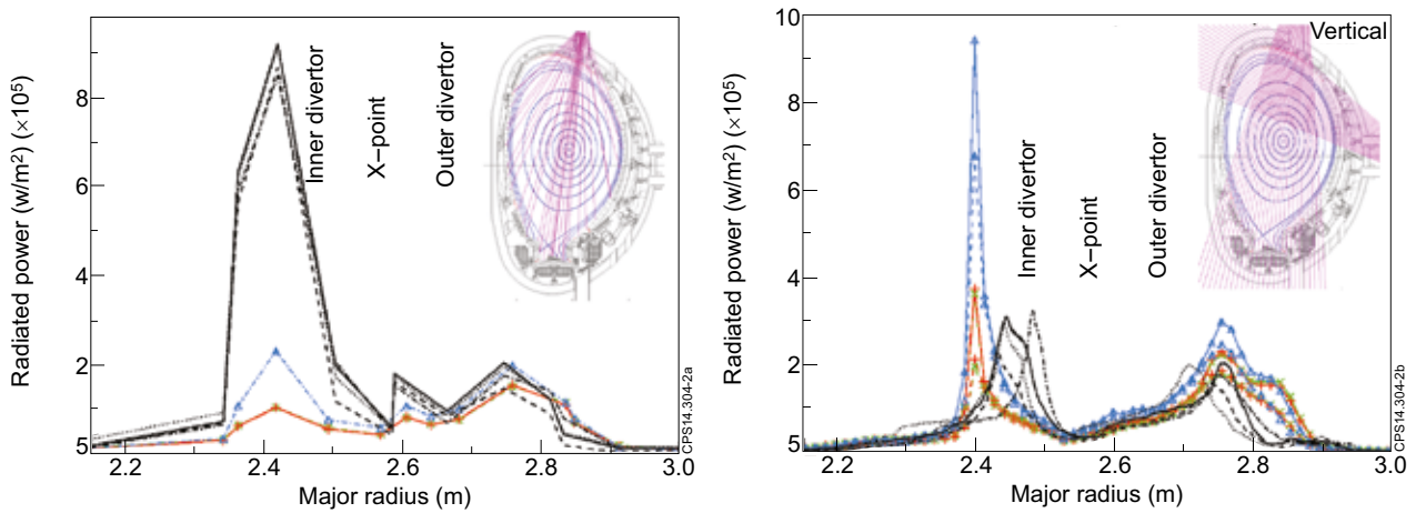
Figure 2. Comparison of a) bolometric radiated powers, b) calculated D line powers for Pulse No: 81472 at 10s, n_{e,sep} = 8.3 \times 10^{18} \text{ m}^{-3} . Measured data (4 curves) without symbols (bolometric powers 1.3 \times 10^4 \text{ W/m}^2 core emission subtracted). Simulated data + no drifts, \Delta with drifts 2.2MW power to SOL, x no drifts 2.8MW power to SOL. Simulated D line powers — total, ---- without D molecular component.
