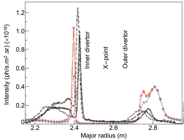
Figure 5. Simulated 527nm, Be II line intensity profiles (— \times 0.1 reduction, ---- \times 0.05 reduction in divertor sputtering yield), 2.2MW power to SOL, n_{e,sep} = 8.0 \times 10^{18} m^{-3} . Other (3) lines are observed emission profiles for Pulse No: 81472 \sim 10s .
