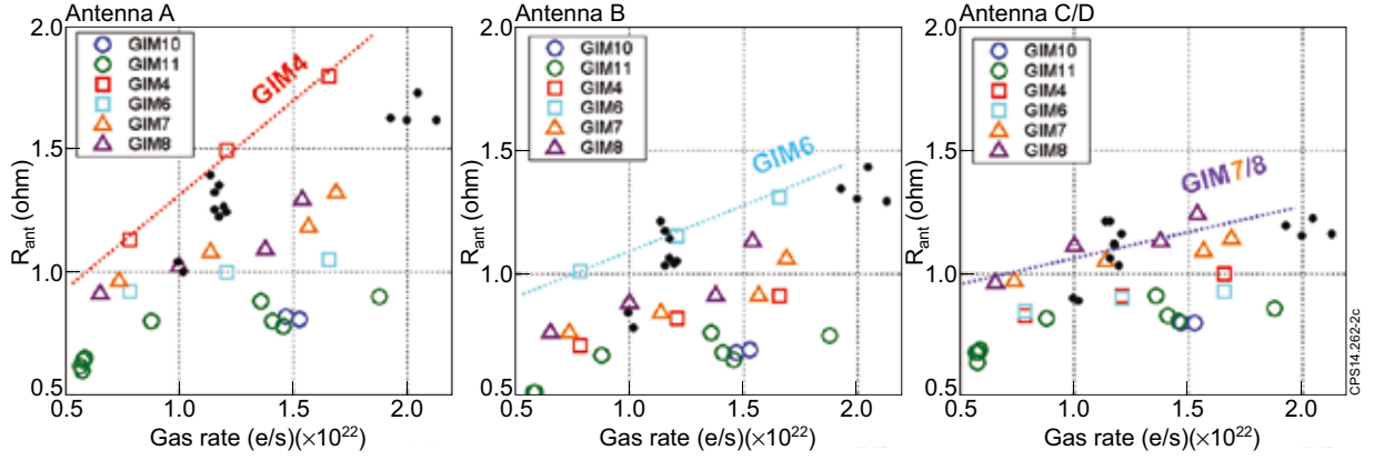
Figure 2: Coupling resistances of the various antenna arrays as function of the total gas injection rate for different fuelling locations: Divertor injection (circles: GIM 10 and 11), mid-plane injection (squares: GIM 4 and 6), top injection (triangles: GIM 7 and 8). The data correspond to 1s averages of the ELM-filtered RF signals at constant gas rate. The black dots represent the results with the best gas injection mix found to simultaneously improve the coupling of all antennas (GIMs 4+6+8).
