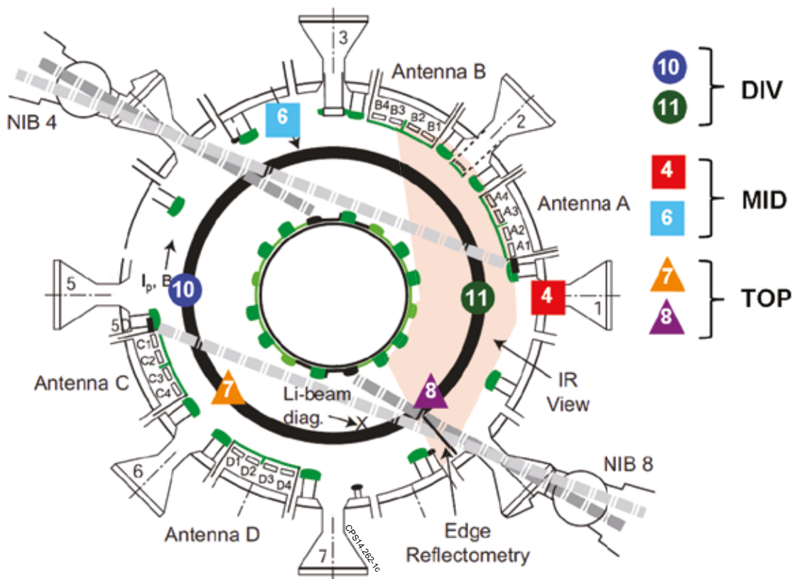
Figure 1: Top view of JET illustrating the toroidal positions of the 4 ICRF antenna arrays and the location of several gas injection modules: GIMs 10/11 (outer and inner divertor rings), GIMs 4/6 (mid-plane valves) and GIMs 7/8 (top valves). The SOL density diagnostics (Li-beam and reflectometry) are also indicated.
