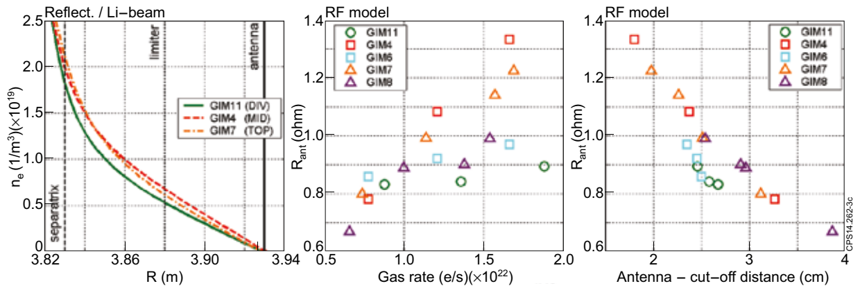
Figure 3: (left) Density profiles reconstructed from reflectometry / Li-beam measurements for 3 gas injection cases: divertor (solid: GIM11, 1.85e22 e/s), mid-plane (dashed: GIM4, 1.65e22 e/s) and top (dash-dotted: GIM7, 1.6e22 e/s); (middle) Coupling resistances calculated by a 1D slab RF coupling code using as input the experimental density profiles reconstructed from reflectometry for the various gas injection cases; (right) Calculated coupling resistances as function of the fast wave evanescence width for f=42\text{MHz} and dipole phasing.
