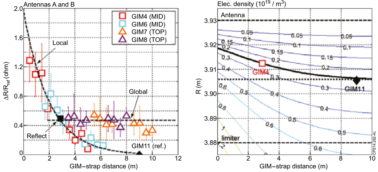
Figure 4: (left) Relative coupling resistance increase of the individual antenna straps with respect to a divertor fuelled discharge (GIM11, 1.85e22 e/s) for two mid-plane (GIM4 and GIM6, 1.65e22 e/s) and two top gas injection pulses (GIM7 and GIM8, 1.6e22 e/s) as function of the toroidal GIM-strap distance; (right) 2D density profile reconstructed from RF coupling modelling by finding analytical density profiles (parameterized to the reflectometry data) that best fit the experimental coupling measurements in each toroidal position for mid-plane gas injection. The thick solid curve represents the cut-off density for the mid-plane gas injection case while the dotted line indicates the cut-off position if divertor fuelling would be used (toroidally homogeneous far-SOL density).
