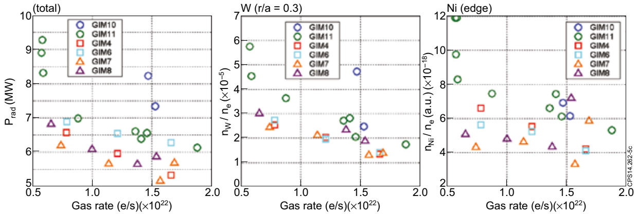
Figure 5: (left) Total radiation, (middle) W concentration at mid-radius and (right) edge Ni concentration (in a.u.) as function of the gas rate for the various fuelling cases studied.
