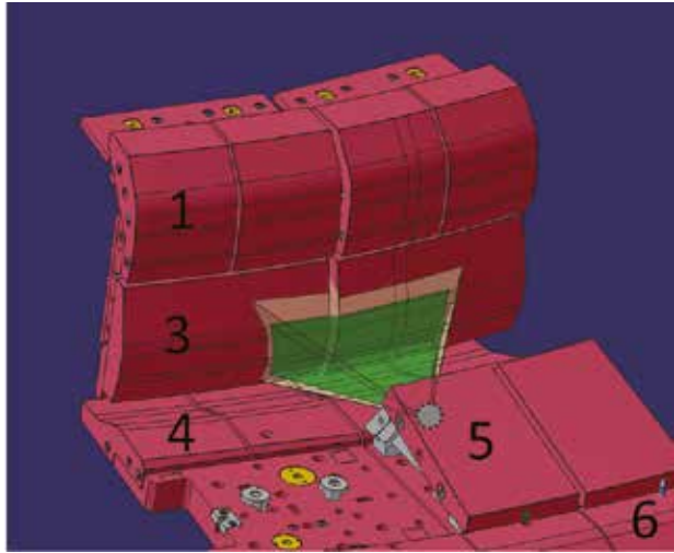
Figure 1: View of the MkIIHD (carbon) inner divertor, with tile numbers labelled. The rotating collector is located under central tile 5 and views tile 3. The projections depict the 'umbra' and 'penumbra' of the view from the collector.
