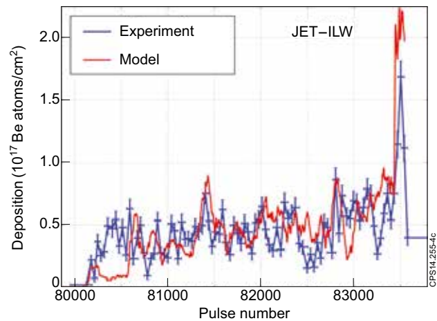
Figure 4: Beryllium deposition on the collector for 2010–12 ILW operation found by NRA (blue), and model scaled by 0.64 attenuation factor (red). The large horizontal error bars at \sim 83,600 indicate that the collector ended its rotation \sim 200 pulses before the end of the campaign, resulting in high aggregate deposition. The modelled deposition for the remaining \sim 200 pulses has been allocated to this stopping point accordingly.
