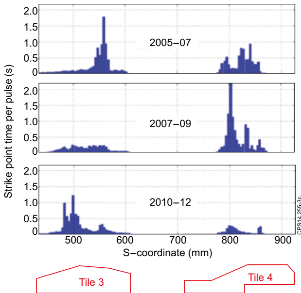
Figure 3: Campaign-averaged inner strike point distributions. The s -coordinate system follows the divertor surface poloidally. For 2010–12 operation there were also a significant number of strike points on tile 1, part of which has an acute line of sight to the collector for the ILW geometry.
