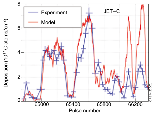
Figure 2: Carbon deposition on the rotating collector for the 2005–07 carbon campaign found by NRA (blue), and model scaled by 0.12 attenuation factor (red). The NRA measurement process is Poissonian, giving n^{-1/2} errors on the deposition. The pulse number error bars show the bounds of the moving sum of deposition imposed by the finite slit width.
