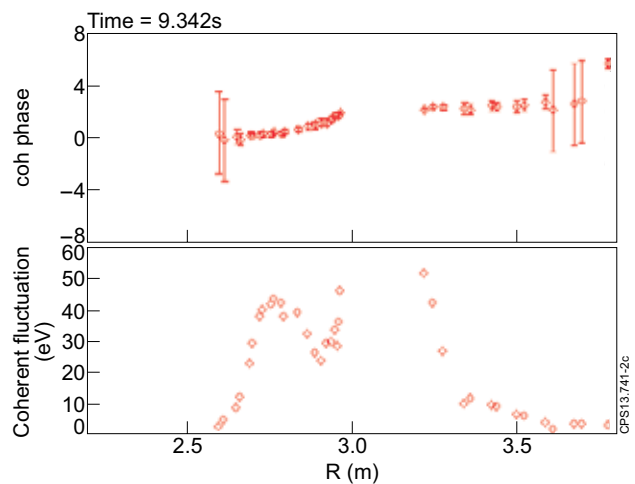
Figure 2: Coherence phase and temperature fluctuation amplitude radial profiles for Pulse No: 74634 (C-Wall).
