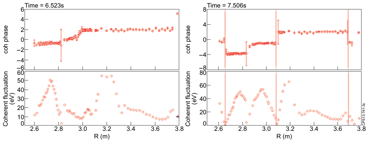
Figure 3: ECE fluctuation phase and amplitude radial profiles for ILW Pulse No: 83525 at 6.52s on the left and at 7.50s on the right.
