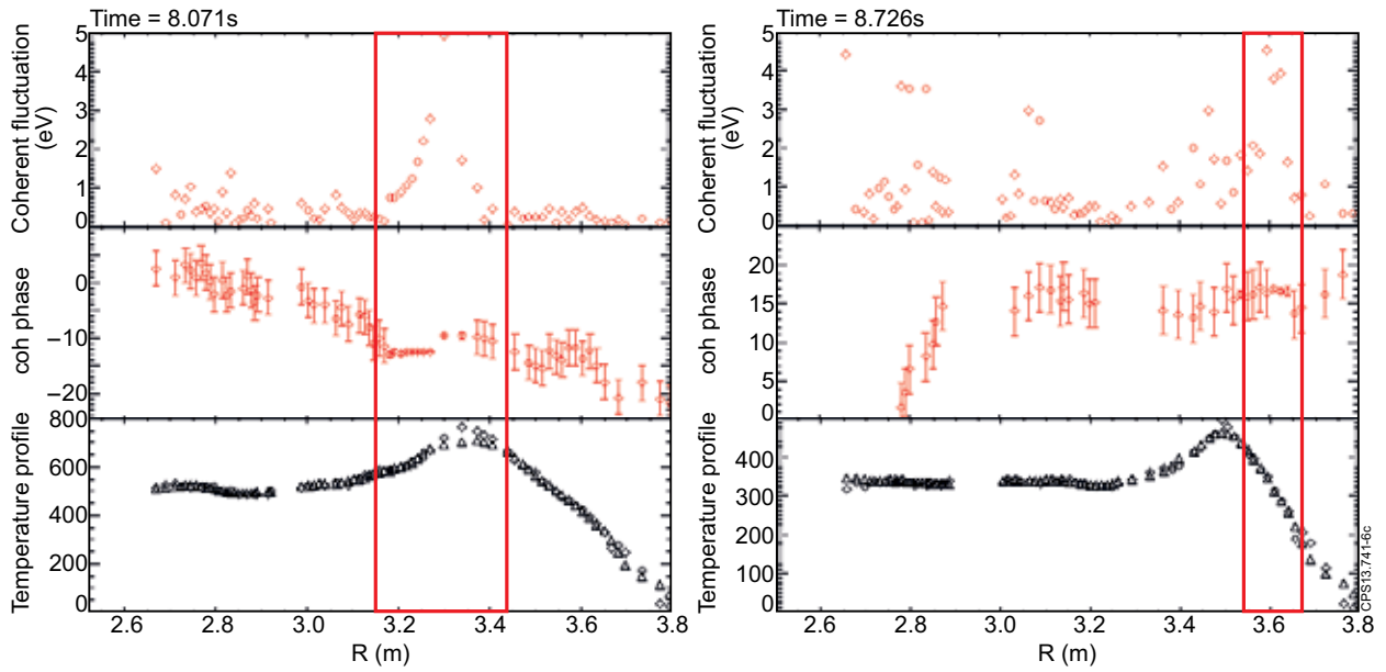
Figure 6: Coherence phase, temperature fluctuation amplitude and temperature radial profiles for Pulse No: 82800 at different times.
