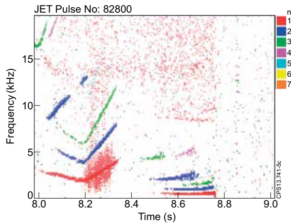
Figure 5: Magnetic spectrogram with mode n number highlighted.
