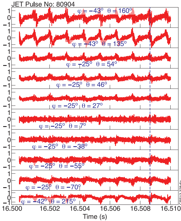
Figure 3: Mirnov signals from poloidal array, showing mode is m = 1 , \sin(\theta) . Toroidal array identifies n = 0 (not shown).
