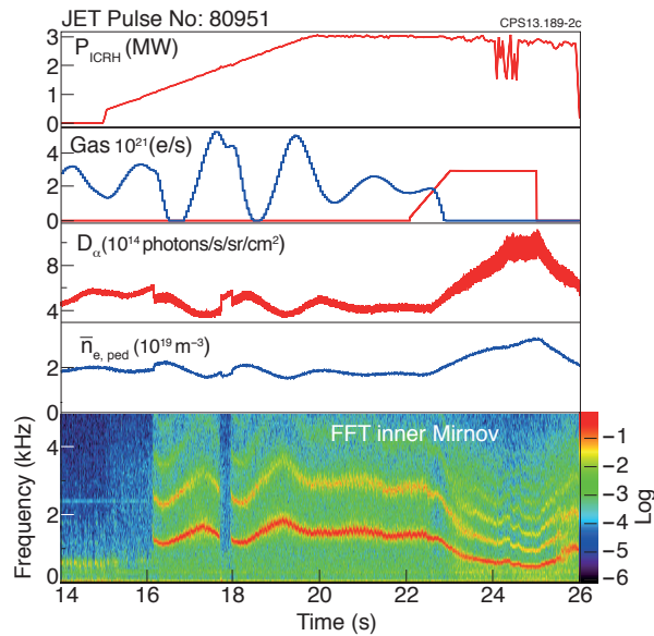
Figure 5: a) ICRH heating power; b) fuelling from divertor and from plasma top (blue and magenta); c) D_\alpha ; d) line integrated pedestal density; e) FFT of Mirnov coil.
