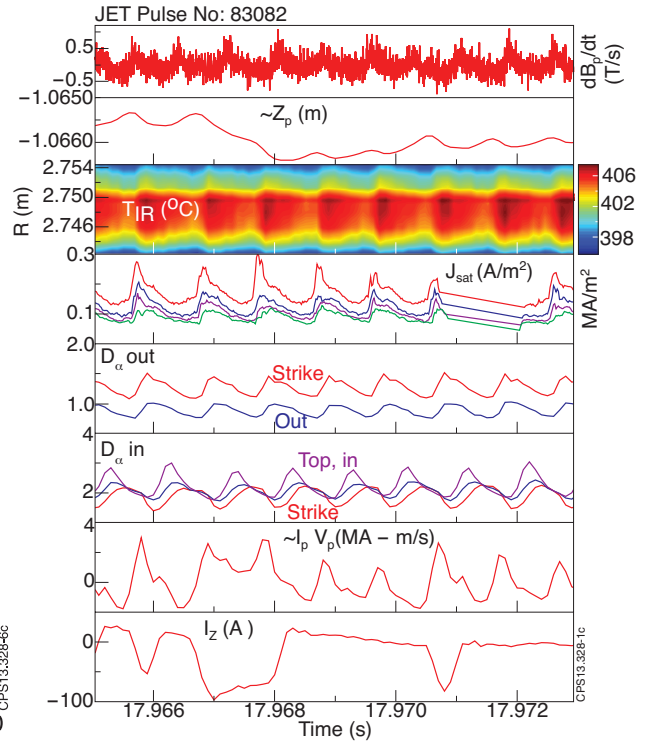
Figure 4: a) dB_\theta/dt from inner Mirnov; b) Proxy of plasma vertical position; c) Temperature profile at outer strike (IR); d) Ion saturation current at outer strike (red), and further out (by 1–2cm); e) D_\alpha at outer strike (red); f) D_\alpha inner strike (red), others further out; g) Plasma velocity proxy, used for position control; h) current in position control power supply.
