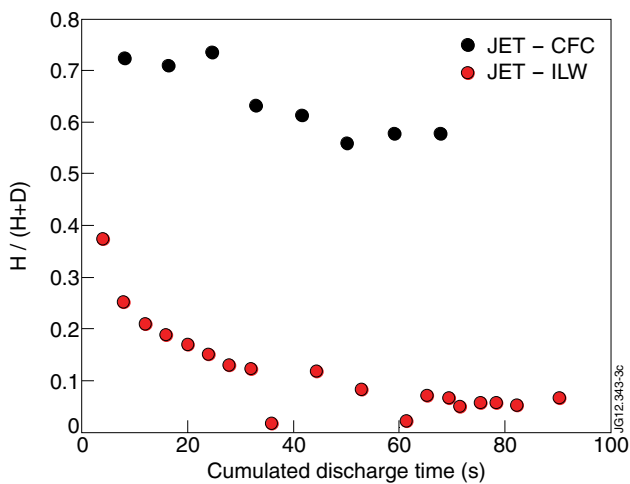
Figure 3. Isotopic ratio as measured by mean of mass spectrometry in the divertor as a function of the cumulated ICWC discharge time in JET-ILW and JET-CFC.
