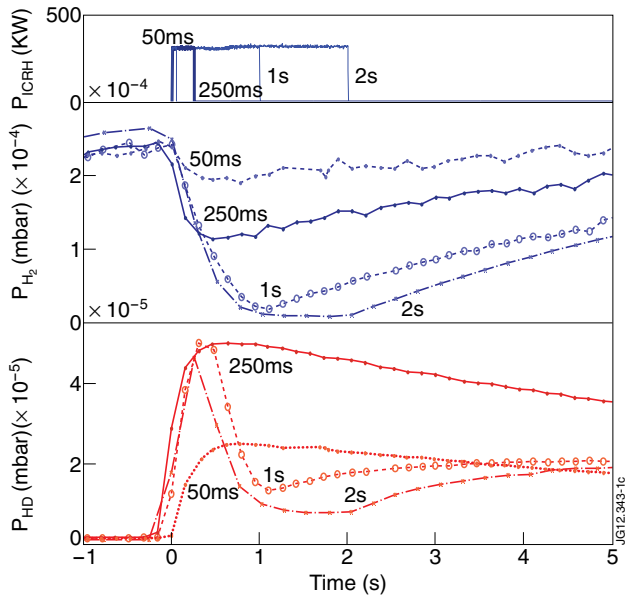
Figure 1: 1:H_2 and HD partial pressure in AUG H2-ICWC discharges with different pulse durations ( P_{RF} = 300kW )
