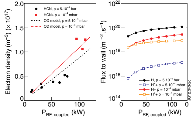
Figure 2: Calculated and measured densities (left) and wall fluxes (right) as a function of coupled power in a TEXTOR H_2 -ICWC discharge ( P(H_2) = 10^{-2} Pa and 5).
