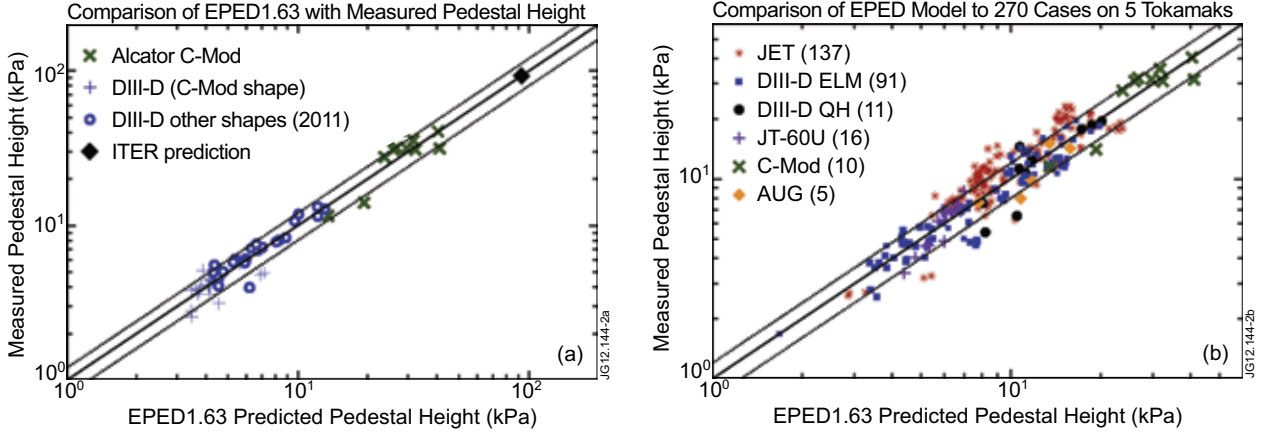
Figure 2: (a) Comparison of EPED predicted pedestal height to observations on Alcator C-Mod and DIII-D, including a similarity experiment on C-Mod and DIII-D. An EPED prediction for the ITER baseline is also shown. (b) Comparison of predicted and observed pedestal height for a set of 270 cases on five tokamaks.
