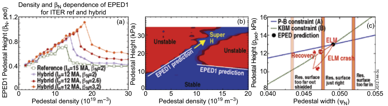
Figure 3: (a) EPED predictions for ITER pedestal height as a function of pedestal density for ITER baseline (15MA) and hybrid (12MA) cases. (b) EPED predictions for pedestal height (white lines) are shown as a function of pedestal density for a high triangularity DIII-D case. Note in particular that a “Super H-Mode” region at very high pedestal pressure is potentially accessible by starting at lower density and then dynamically increasing the density in time to move up and to the right in this parameter space. (c) A working model for RMP ELM suppression is illustrated, showing that a region of increased transport (here associated with a rational surface, e.g. an island or stochastic region) can suppress the ELM if this region is in the proper location to constrain the broadening of the pedestal.
