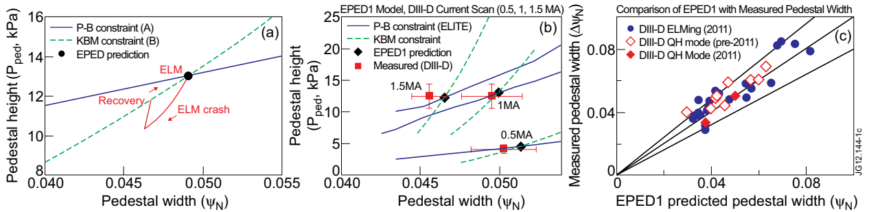
Figure 1: (a) EPED predicts the pedestal height and width (black circle) as the intersection of calculated peeling-ballooning (solid line) and KBM (dotted line) constraints. A typical ELM cycle in this space is illustrated in red. (b) EPED predicted height and width (black diamonds) is compared to observations (red squares) for a current scan across 3 discharges on DIII-D. (c) Comparison of EPED predicted and observed pedestal width for a set of DIII-D discharges with accurate width measurements from a new Thomson system (blue circles) as well as from a set of 11 QH mode discharges (diamonds).
