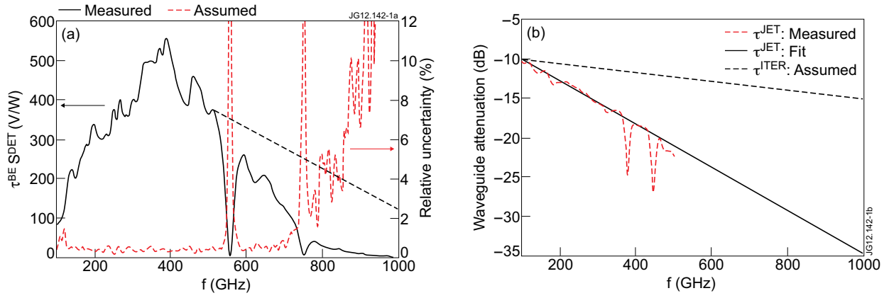
Figure 1: (a) Measured (black) and estimated (dashed) sensitivity of Michelson interferometer back end assuming an ideal antenna. (b) Measured (red) and estimated (dashed) attenuation of transmission lines.
