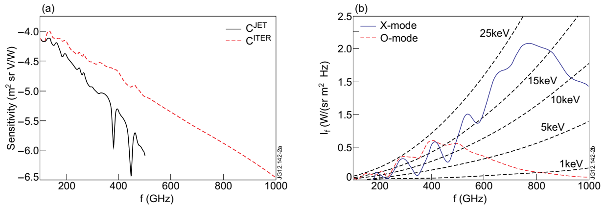
Figure 2: (a) Measured sensitivity (black) and estimated minimum sensitivity (red) required for calibration up to 1 THz. (b) Predicted ECE spectrum I_f for pure O- and X-mode polarization for central T_e = 25 \text{ keV} .
