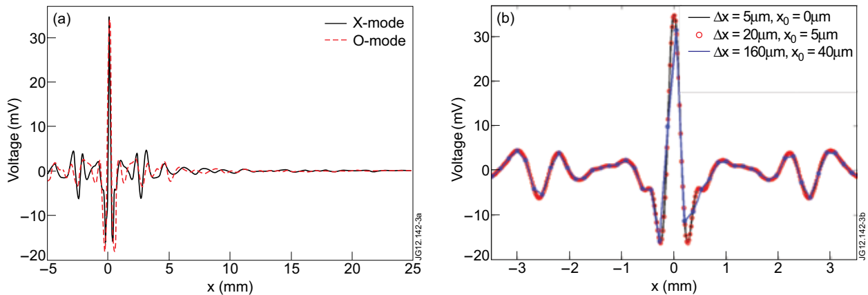
Figure 3: (a) Predicted interferogram for pure ECE spectrum in X- (black) and O-mode (red) polarization. (b) Effect of spatial sampling of interferogram around ZPD position for X-mode polarization.
