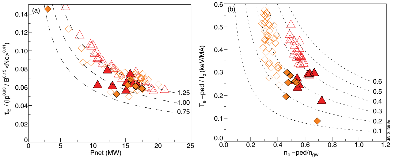
Figure 5: Hybrid plasma. Normalized energy confinement versus input power (a). Normalized pedestal temperature versus normalized pedestal density, (b). Symbol definition as in figure 1.
