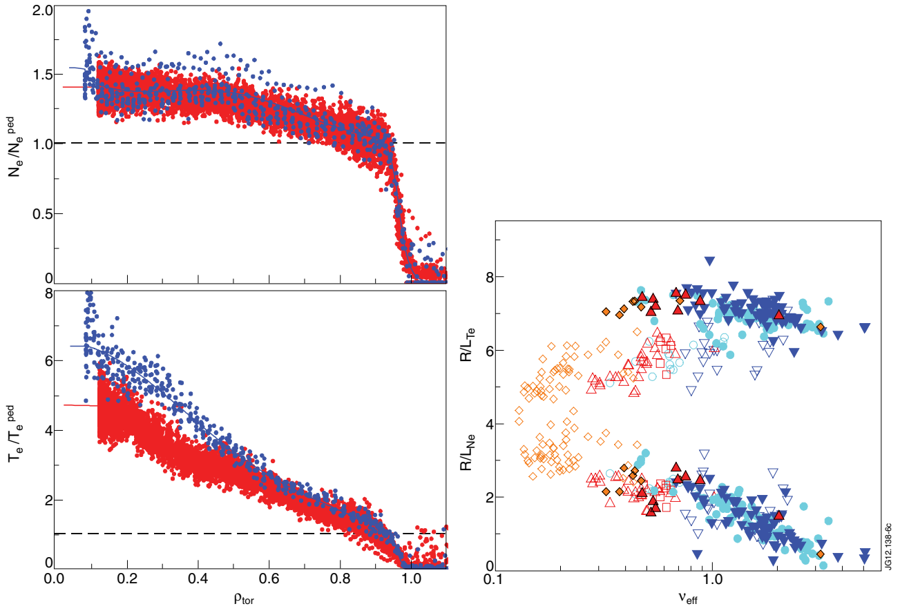
Figure 6: Gradient length at \rho_{tor} = 0.6 (a). Normalized N_e and T_e profile for a ILW (blue) and a CFC (red) shot with \nu_{eff} = 0.9 (both high \delta BL plasmas).
