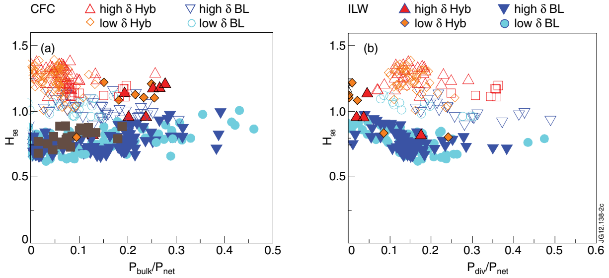
Figure 2: Confinement factor versus the power radiated by the bulk plasma normalized to the total input power (a) and versus the power radiated at the divertor normalized to the total input power
