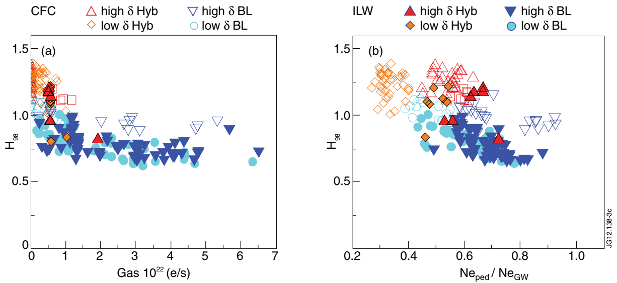
Figure 3: Confinement factor versus gas rate (a) and versus pedestal density normalized to the Greenwald density (b).
