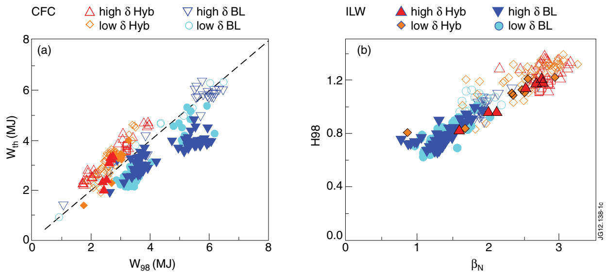
Figure 1: Frame (a): stored thermal energy obtained from the diamagnetic energy corrected for the fast particle energy versus the thermal energy expected by the IPB98(y,2) scaling. Frame (b) H_{98} versus normalized beta for CFC and ILW plasmas.
