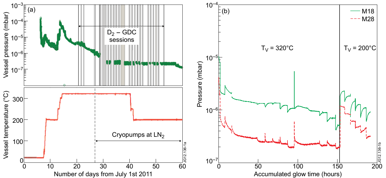
Figure 1: (a) The initial conditioning cycle of JET with ILW: penning pressure, vacuum vessel temperature and (b) partial pressures of H_2O and CO during the D_2 -GDC ( p = 3 \times 10^{-3} mbar, I = 15A , U = 500V ).
