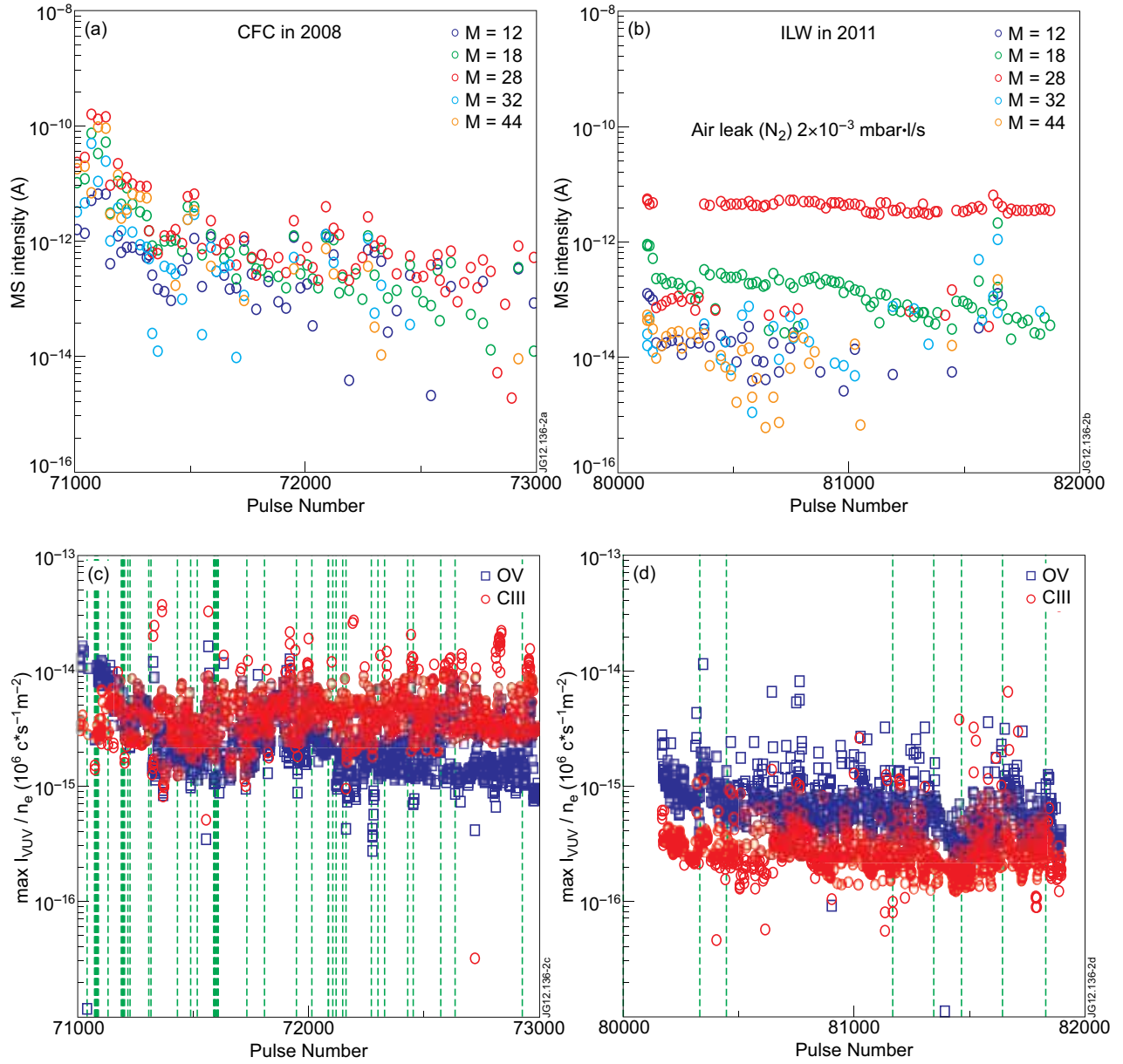
Figure 2: Residual gas impurity levels 1 hour before the first pulse of the day in 2008 (a) and for the restart with ILW (b). Normalized OV and CIII line intensities in plasmas and GDCs applied (green dashed lines) in 2008 (c) and 2011 (d).
