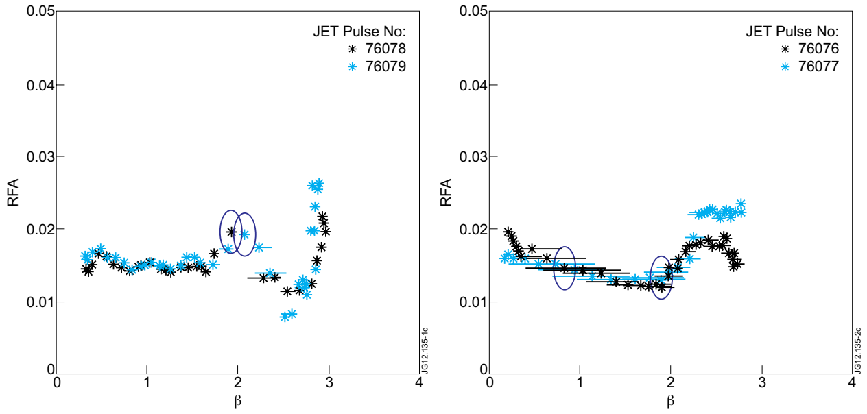
Figure 2: RFA measurements of four adjacent shots with the same plasma conditions. (left) no additional puffing (right) with additional puffing showing suppression of the early peak. The appearance of the first ELM is highlighted with a blue circle.
