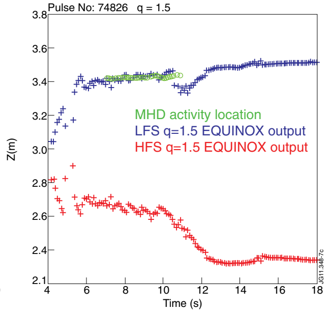
Figure 5: Comparison between MHD markers and location of q=1.5 obtained in real time from EQUINOX (constrained with polarimetry), (Pulse No: 74826, 19MW NBI, I_p = 1.6\text{MA} , B_T = 2\text{T} )
