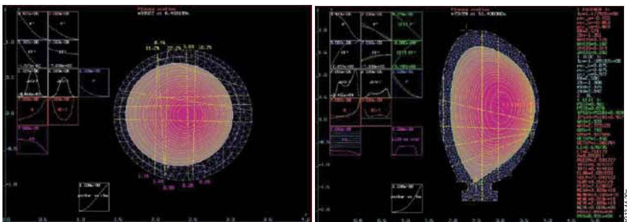
Figure 1: Examples of Equilibrium reconstruction: left Tore Supra case (Pulse No: 33922 at 6.4s) right JET case (Pulse No: 70199 at 11.4s).
