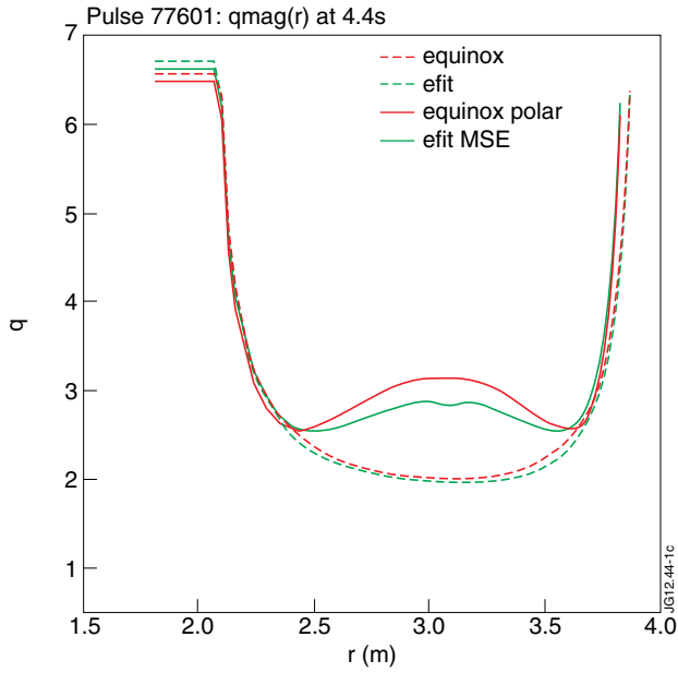
Figure 4: Comparison between EQUINOX and EFIT of q profile magnetic only (dotted lines), polarimetry and MSE (green plain lines) Pulse No: 77601, I_p = 1.7\text{MA} , B_T = 2.6\text{T} , 3MW LHCD (Lower Hybrid Current Drive), 6MW ICRH (Ion Cyclotron Resonance Heating), 20MW NBI.
