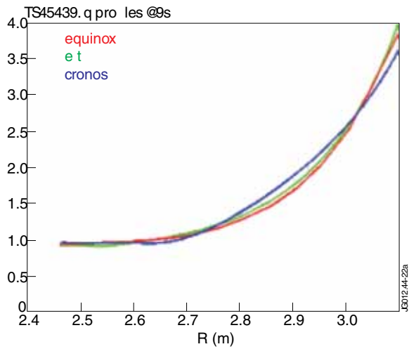
Figure 7:(a) Comparison of q profiles obtained by EQUINOX, EFIT, and the current diffusion code Cronos. 7 (b) Comparison of rational q surfaces evolution with time for EQUINOX, EFIT and CRONOS. The sawteeth inversion radius is indicated.
