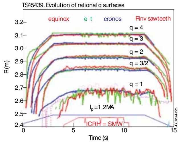
Figure 7:(a) Comparison of q profiles obtained by EQUINOX, EFIT, and the current diffusion code Cronos. 7 (b) Comparison of rational q surfaces evolution with time for EQUINOX, EFIT and CRONOS. The sawteeth inversion radius is indicated.
