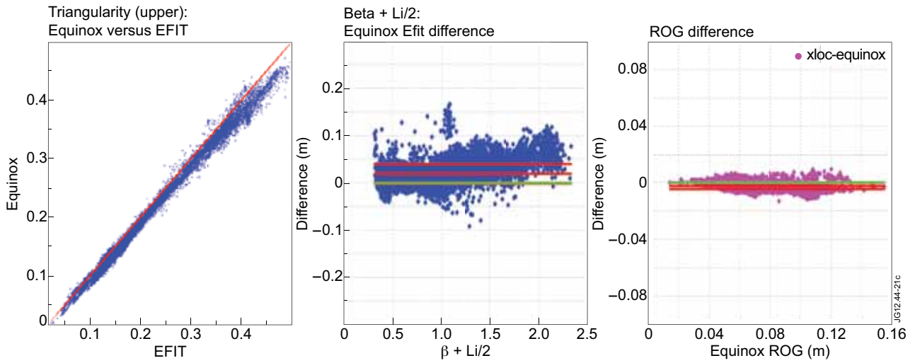
Figure 2: Statistical comparisons between EQUINOX and EFIT [5] for (a) triangularity (b) Shafranov Shift and XLOC (c) Right Outer Gap (ROG)). Horizontal green line zero reference, horizontal red lines standard deviations
