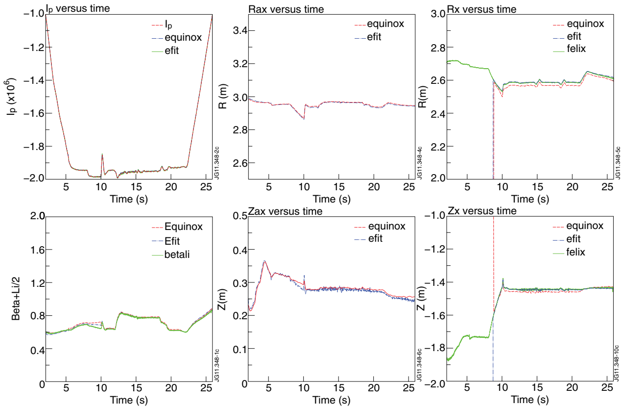
Figure 3: Example of dynamical comparison between EQUINOX and EFIT Pulse No: 81991 (6MW NBI (Neutral Beam Injection) applied at 12s to 19.3s, plasma current I_p = 2\text{MA} Magnetic toroidal field B_T = 2.9\text{T} )
