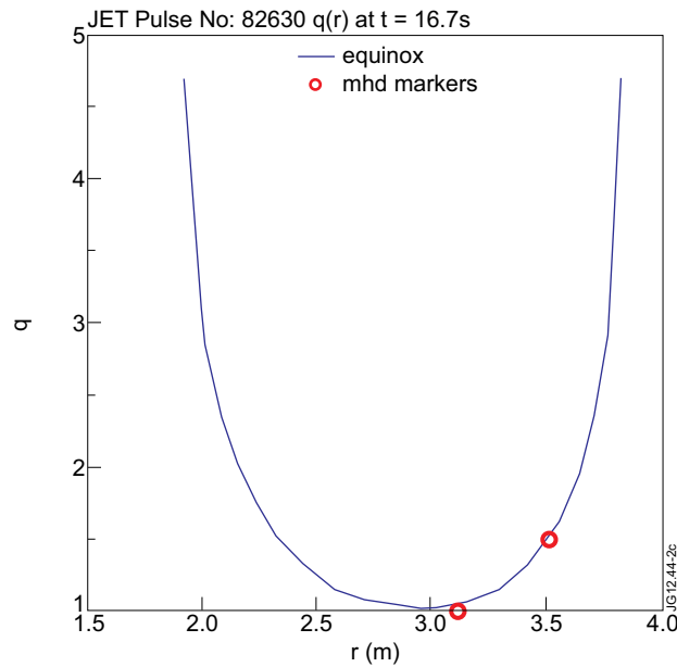
Figure 6: Comparison between MHD markers position and q profile obtained from EQUINOX real time constrained with polarimetry, ohmic Pulse No: 82630 at 16.7s
