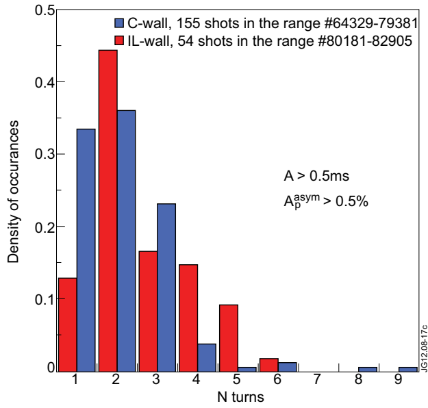
Figure 5: Distribution of the number of rotations.
