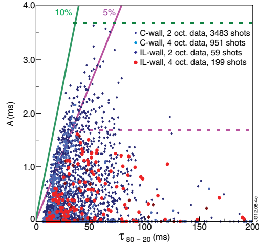
Figure 3: The severity of I_p asymmetries (Hiro currents) for C- and IL-walls.
