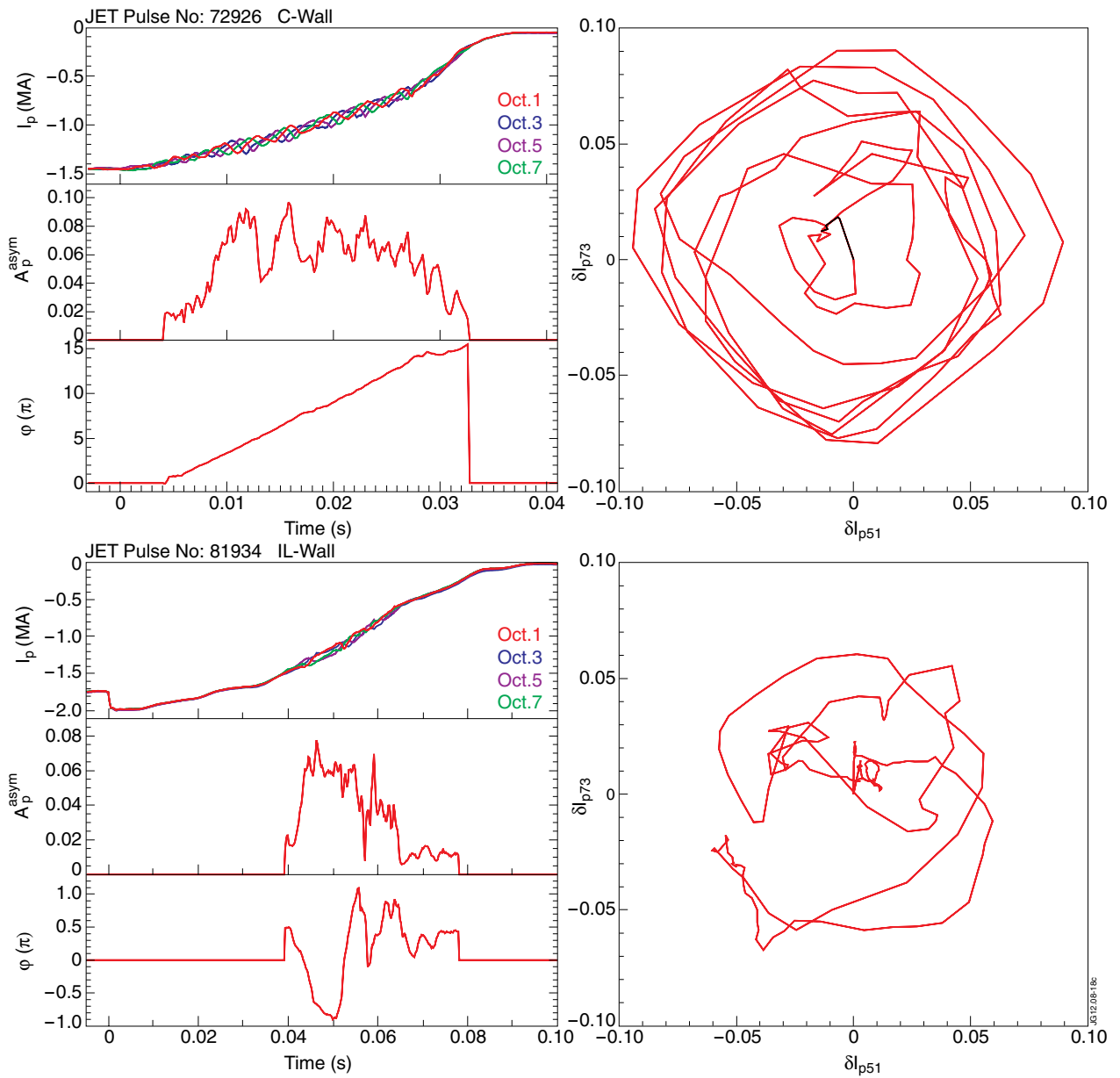
Figure 4: Waveforms of the the I_p , A_p^{asym} , mode toroidal angle ( \phi ) and JET top view on trajectories of the tip of I_p asymmetry vector: multi-turn fast rotation (top), rotation with reversal (bottom).
