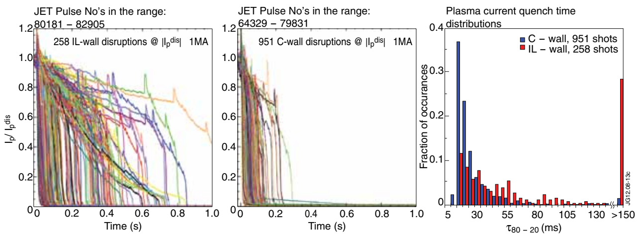
Figure 2: Normalised plasma current during IL-wall (left), C-wall (centre) disruptions and their CQ time distributions (right); where \tau_{80-20} is the CQ time extrapolated from time to quench from 80 to 20% of I_p^{dis} .
