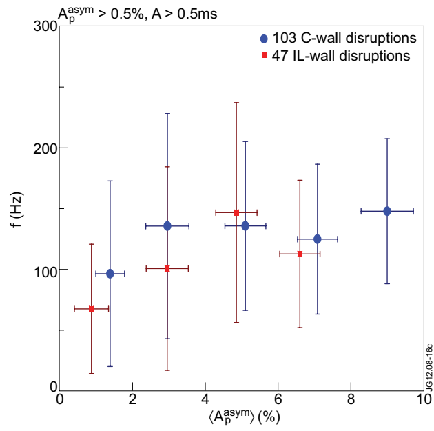
Figure 7: Variation of the “one turn” frequency versus average I_p asymmetry (Hiro current) amplitude.
