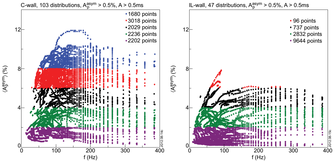
Figure 6: Normalised amplitude of plasma current asymmetry divided on the five \langle A_p^{\text{asym}} \rangle regions versus “one turn” rotation frequency.
