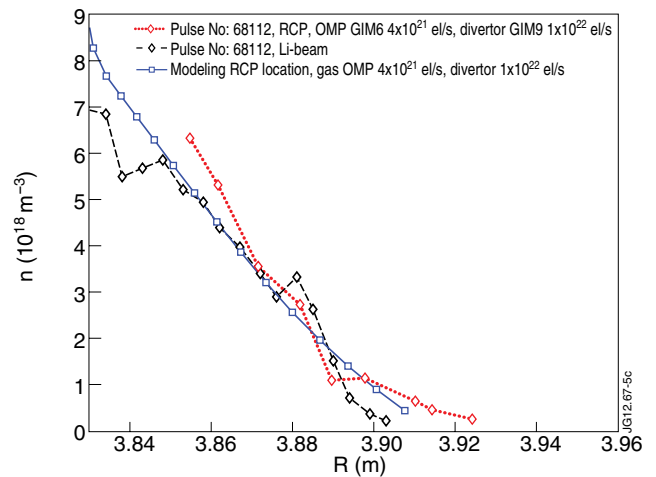
Figure 5: Comparison of n_{eSOL} profiles simulations at the RCP and Li beam locations with the experimental profiles from Pulse No: 68112 using D = 1.75 \text{ m}^2/\text{s} and using the same gas puff as in the experiment. The modeling separatrix is at the coordinate R = 3.82 \text{ m} .
