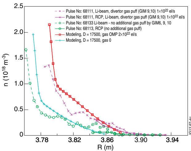
Figure 4: Comparison of n_{eSOL} profiles simulations at the RCP and Li beam locations with the JET experimental profiles using D = 1.75 \text{ m}^2/\text{s} . For the red modeling curve, the modeling separatrix is at R = 3.79 \text{ m} .
