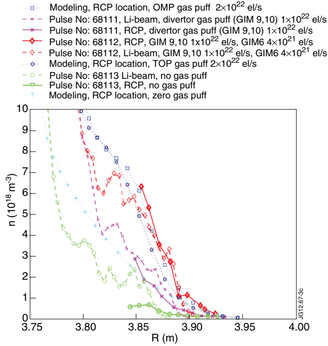
Figure 3: Comparison of n_{eSOL} profiles simulations at the RCP and Li beam locations with the JET experimental profiles using D = 1 \text{ m}^2/\text{s} . The RCP and Li beam measurements were done at 8s, at ROG 14cm.
