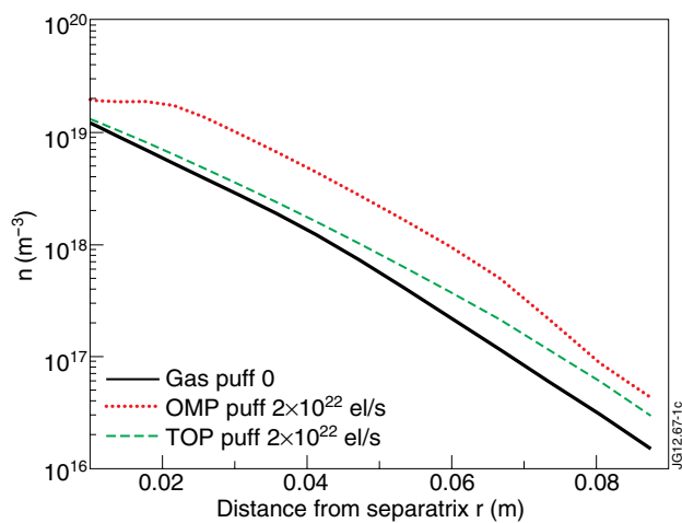
Figure 1: OMP n_{eSOL} profiles, TOP and OMP gas puff 2 \times 10^{22} el/s and ICRF power level of 2MW.
