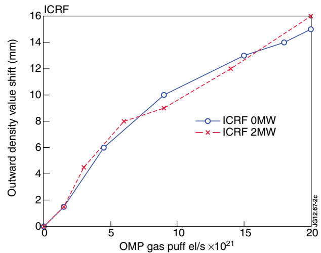
Figure 2: Outward OMP shift of the cut-off density value of 2 \times 10^{18} \text{ m}^{-3} . (JET scenarios [3]) for different OMP gas injection levels.
