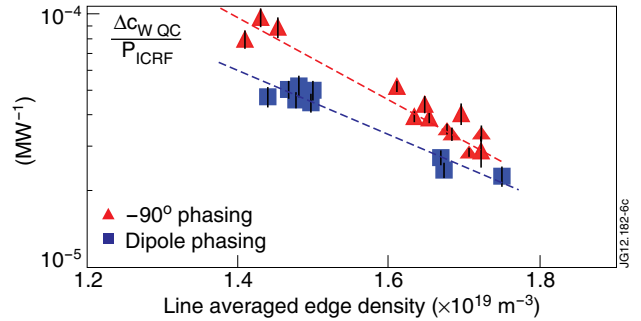
Figure 6: Comparison of c_{wQC} in the dipole and the -90^\circ ICRF (only A and B) powered L-modes.
