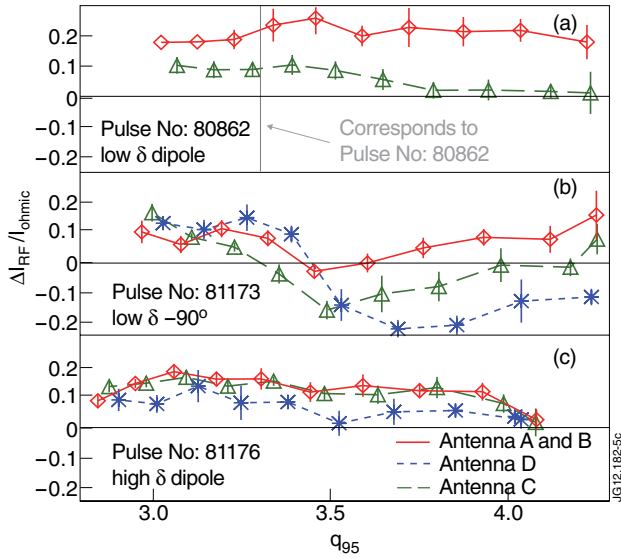
Figure 5: Relative change of WI intensity at the top of tile 8 near antenna B during 1 MW of ICRF with respect to ohmic phases, deduced from the WI imaging: a) low with dipole; b) low with -90^\circ ; c) high with dipole.
