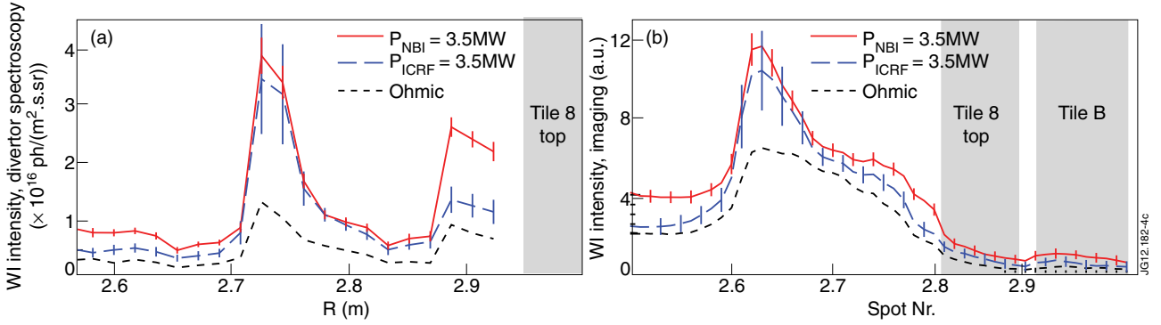
Figure 4: WI emission at 400.8 nm from the WI spectroscopy (a) and the WI imaging (b) in Pulse No 81852 for ohmic only, ICRF and NBI heated phases (3.5MW phases). Top of tile 8 is indicated, which appears larger on the WI imaging system due to viewing geometry.
