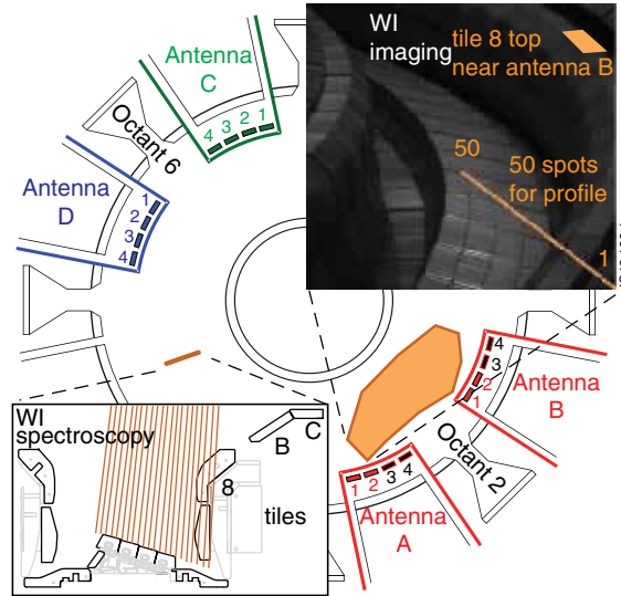
Figure 1: Arrangement of ICRF antennas and W source diagnostics in the divertor.
