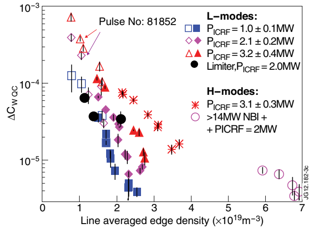
Figure 3: Dependence of change of c_{WQC} during ICRF on line averaged edge density. Open squares, diamonds and triangles: B_T = 2.55T , I_p = 2.5MA , low shape; stars, filled squares, diamonds and triangles: B_T = 2.4 T , I_p = 2MA , low shape; open circles: B_T = 2.7T , I_p = 2.5MA , high shape; closed circles: B_T = 2.5 T , I_p = 2 MA , limiter shape.
