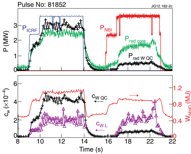
Figure 2: Comparison of ICRF and NBI heating in Pulse No: 81852 with B_T = 2.55T and f_{ICRF} = 42MHz . Upper graph: solid lines without symbols - applied ICRF and NBI power, crosses - radiated power estimated using c_{WQC} , dashed line - measured core radiation. Lower graph: solid line with crosses - c_{WQC} measured at \rho_{QC} = 0.6 \pm 0.1 during ICRF and at \rho_{QC} = 0.5 \pm 0.2 during NBI; solid line with triangles - c_{WL} measured at \rho_L = 0.25 \pm 0.1 during ICRF and at \rho_L = 0.2 \pm 0.1 during NBI.
