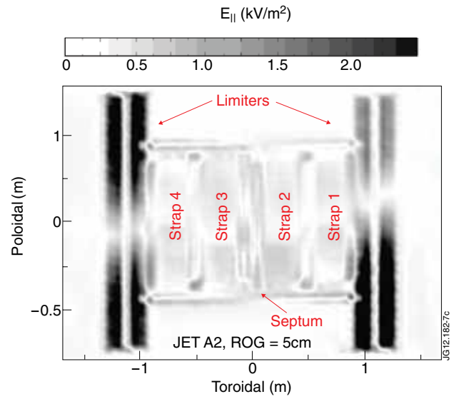
Figure 7: TOPICA calculations of E_{||} in front of (0\pi0\pi) phased JET A2 antenna in L-mode, normalized to 1MW coupled to antenna.
