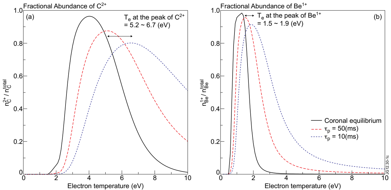
Figure 1: (a) and (b) show the fractional abundance of C^{2+} and Be^{1+} , respectively. In both figures, each line indicates the assumed equilibrium or particle confinement time: solid black (Coronal equilibrium), dashed red ( \tau_p = 50 [ms]), and dashed blue ( \tau_p = 10 [ms]).
