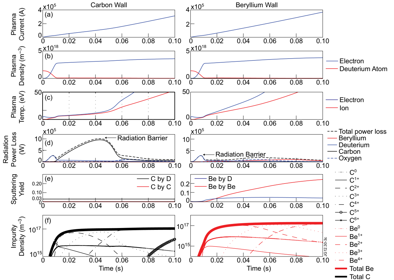
Figure 3. Simulation results in the carbon wall and the ILW under the identical conditions are presented: (a) Plasma current, (b) electron density (blue) and deuterium atom density (red), (c) electron temperature (blue) and ion temperature (red), (d) radiation power losses (dashed black: total radiation power loss, solid blue: deuterium radiation, solid red: beryllium radiation, solid black: carbon radiation, dashed blue: oxygen radiation.), (e) sputtering yield (solid black: carbon sputtering due to incident deuterium ion, solid blue: beryllium sputtering due to incident deuterium ion, solid red: self-sputtering yield), (f) impurity densities in each charge state.
