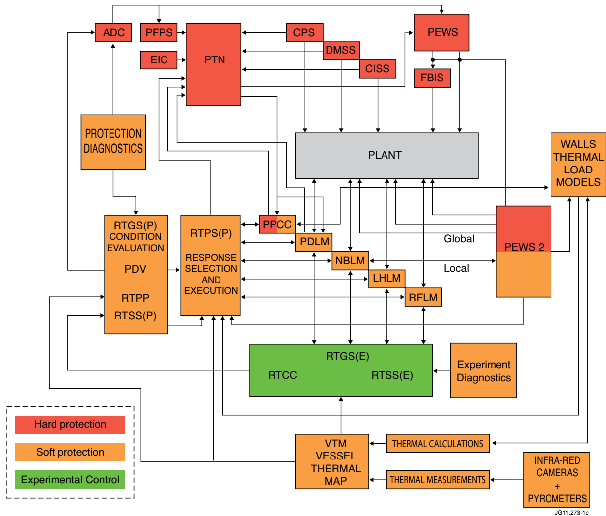
Figure 1: JET protection of the ITER-like wall system architecture. The experimental real-time control links to the density and heating local managers (PDLM, NBLM, RFLM and LHLM) is expanded to allow protection overrides from the new RTPS system which receives alarms from VTM, WALLS and also from the Real-Time Plasma Protection (RTPP) and Real-Time Central Controller (RTCC) systems. The original higher level protection systems of CISS, PTN and PEWS are retained.
