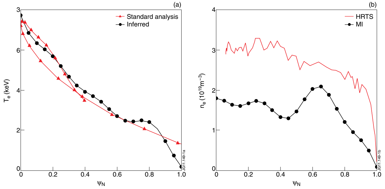
Figure 1: Derived profiles (black) for Michelson interferometer in terms of normalized flux \psi_N for JET Pulse No: 79853, t=14.72\text{s} . (a) Temperature T_e . The standard analysis (red) does not assume T_e preservation on flux surfaces. (b) Density n_e . The inferred density is smaller with respect to the one (red) measured by the High Resolution Thomson Scattering (HRTS) diagnostic and others.
