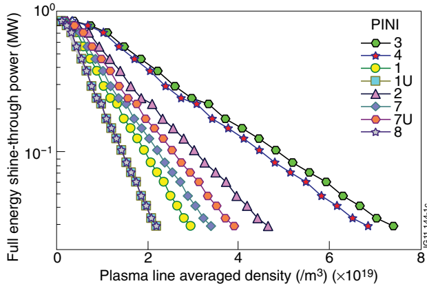
Figure 1: Shine-through power of the full energy component for each PINI as a function of the plasma line averaged density.
