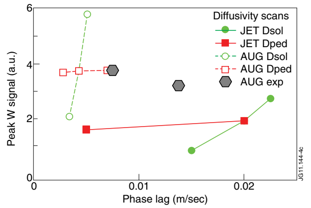
Figure 4: The magnitude of the EDGE2D calculated tungsten density (at r/a = 0.8 ) in response to an oscillating source. The AUG (hollow symbols and dashed lines) source was at the outer mid-plane (location of ICRF antenna). The JET (solid symbols and lines) source was at the inner mid-plane (location of W shine-through protection tiles). Each calculation had low/medium/high ( 0.5, 1, 2 \text{ m}^2/\text{s} ) values of SOL W diffusivity (green) and pedestal diffusivity (red). The AUG data is shown for illustration and is not a fit to the EDGE2D calculations.
