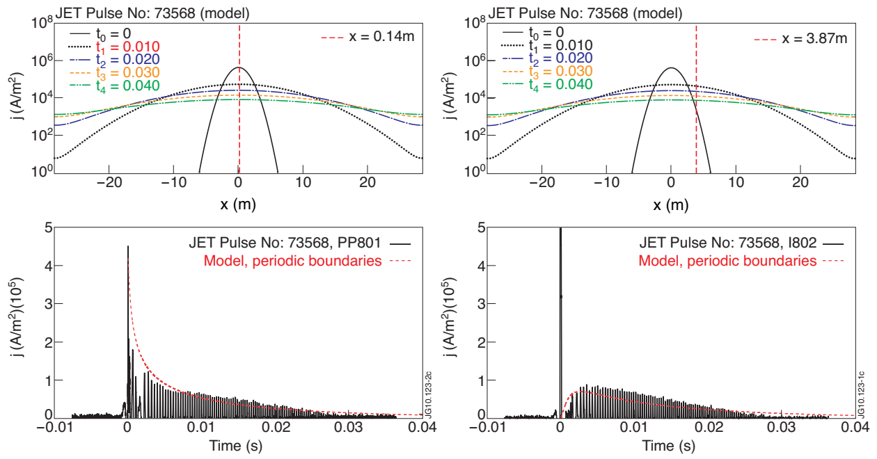
Figure 3: Comparison of measured and simulated current densities for the outboard a) and inboard side b) of JET (JET Pulse No: 73568, t_0 = 12:9936 s).
