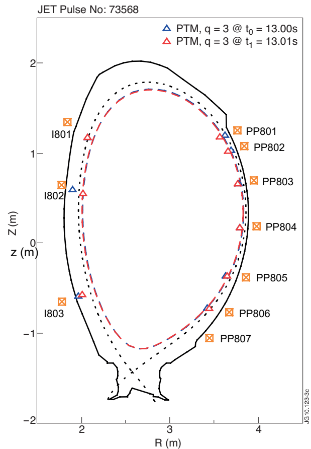
Figure 2: Computed location of a PTM filament and the q = 3 surface for two different time steps with respect to coil PP804. JET Pulse No: 73568, t_0 = 13.00s (blue), t_1 = 13.01s (red).
