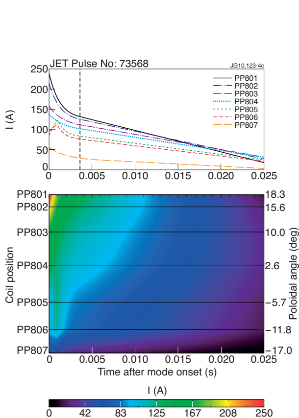
Figure 1: Evolution of a PTM (JET Pulse No:73568, t_0 = 12.996s ) as seen by the poloidal limiter coil array in quadrant eight.
