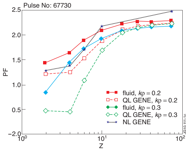
Figure 1: Impurity peaking factor PF = -R \nabla n_Z / n_Z versus Z for Z \geq 2 as obtained by Weiland fluid model and quasi-linear and nonlinear GENE simulations in the collisionless, electrostatic limit. The parameters are taken from JET Pulse No: 67730 at r/a \approx 0.5 .
