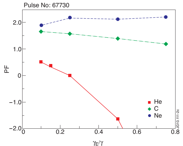
Figure 2: Impurity peaking factor -R \nabla n_Z / n_Z versus shearing parameter \gamma_E / \gamma_i . The parameters are taken from JET Pulse No: 67730 at r/a \approx 0.5 . The results are obtained with the fluid model.
