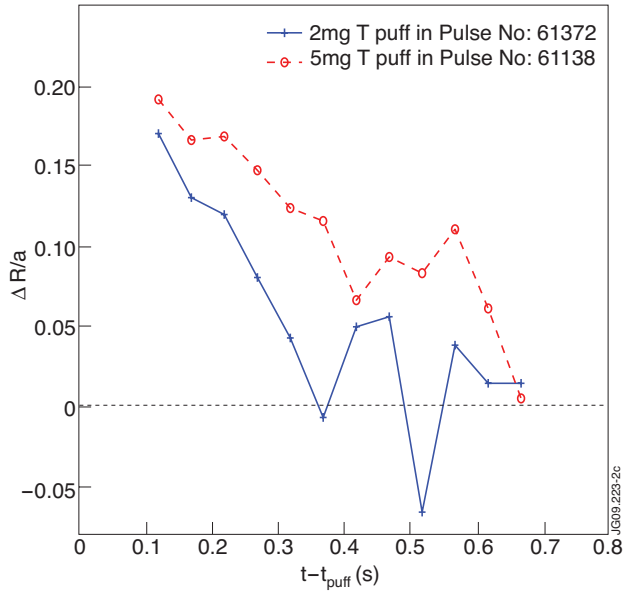
Figure 2: Evolution of radial asymmetry of the DT/DD emissivity ratio in two almost identical JET discharges after different level of tritium puff.
