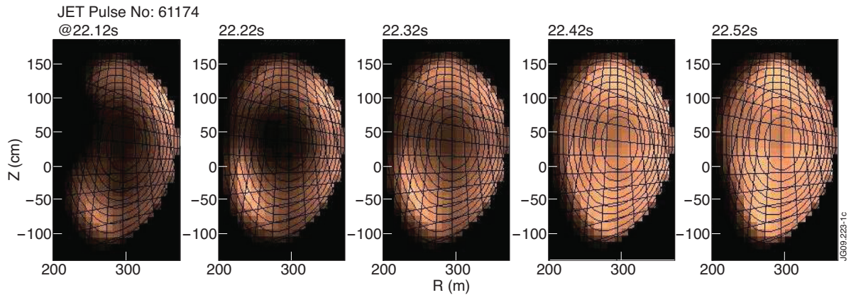
Figure 1: Typical evolution of the DT/DD neutron emissivity ratio after T puff (JET Pulse No: 61174)
