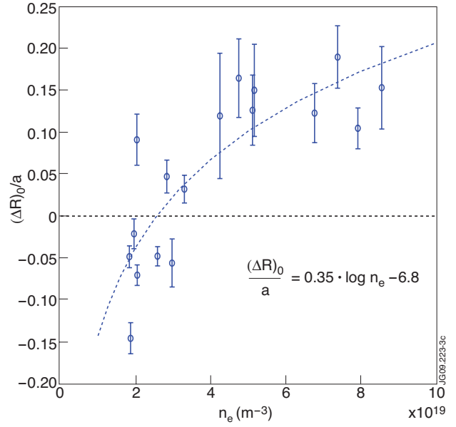
Figure 3: Initial radial offset of the DT/DD emissivity as a function of plasma density. A tentative logarithmic fit to the experimental data is shown (dashed line).
