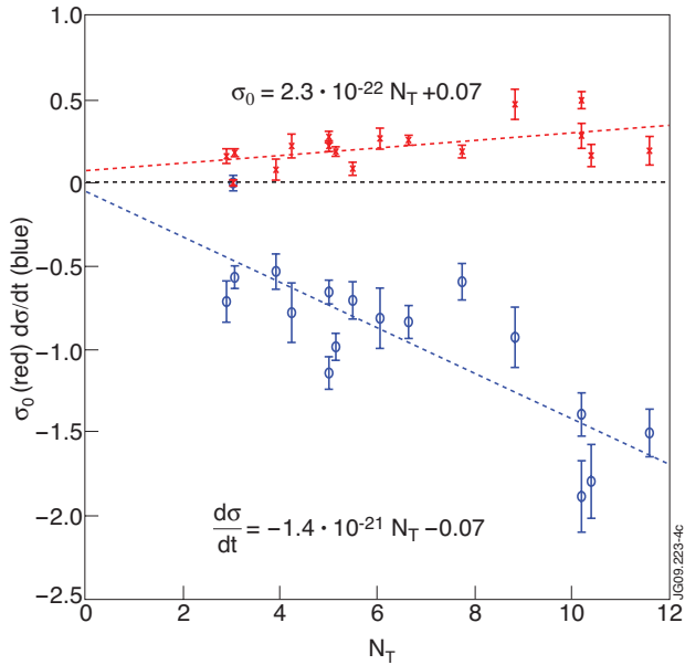
Figure 4: Initial offset (in red) and time derivative (in blue) of the standard deviation of the poloidal component of the emissivity ratio as a function of the amount of puffed tritium. Notice that linear fits (dashed lines) extrapolate to zero at zero puff.
