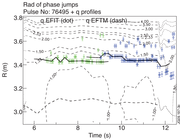
Figure 3: Mode locations for the 4/3 and 3/2 modes. Error bars represent half the distance between channels that enclose the p -phase jump.
