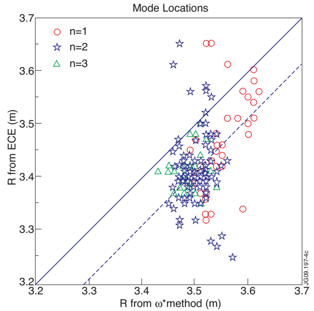
Figure 4: Comparison between locations from mode frequency and from T_e oscillations for m/n=2/1, 3/2 and 4/3 modes. Identity corresponds to the blue solid line. The dashed line is shifted by 9cm
