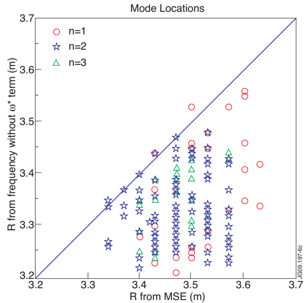
Figure 6: Rational q locations from mode frequency without ion diamagnetic drift and from MSE diagnostic. Identity corresponds to the blue line.
