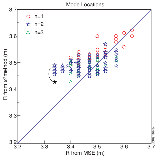
Figure 5: Comparison between rational q locations from mode frequency including ion diamagnetic drift and from MSE diagnostic for m/n= 2/1, 3/2 and 4/3 . Identity corresponds to the blue solid line.
