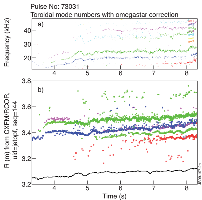
Figure 2: (a) Spectrogram of magnetic signals, with toroidal number shown in color code. (b) Mode locations in major radius for m/n=1/1 (red), 4/3 (inner green points), 3/2 (blue), 5/3 (outer green points).
