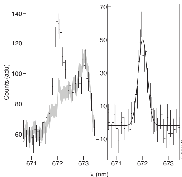
Figure 1: Measured beam emission spectrum of the 5th spatial channel of the observation system. The measured spectrum (left, black points with error bars) is shown together with the estimate for the background radiation obtained from the adjacent beam-off time frames (gray, shaded area shows uncertainty.). In the right part of the figure, the signal is shown after subtracting the background. The black line depicts a Gaussian fit to the signal.
