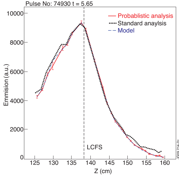
Figure 2: Emission profile as obtained by the fitting procedure. The red curve shows the measured emission with its uncertainty. The blue curve shows a simulated emission profile, which was obtained from the forward calculation, using parameters fitted to the shown data. The black curve shows the emission profile obtained from the standard lithium beam analysis. The dashed line shows the position of the Last Closed Flux Surface (LCFS), as obtained by the plasma equilibrium reconstruction EFIT.
