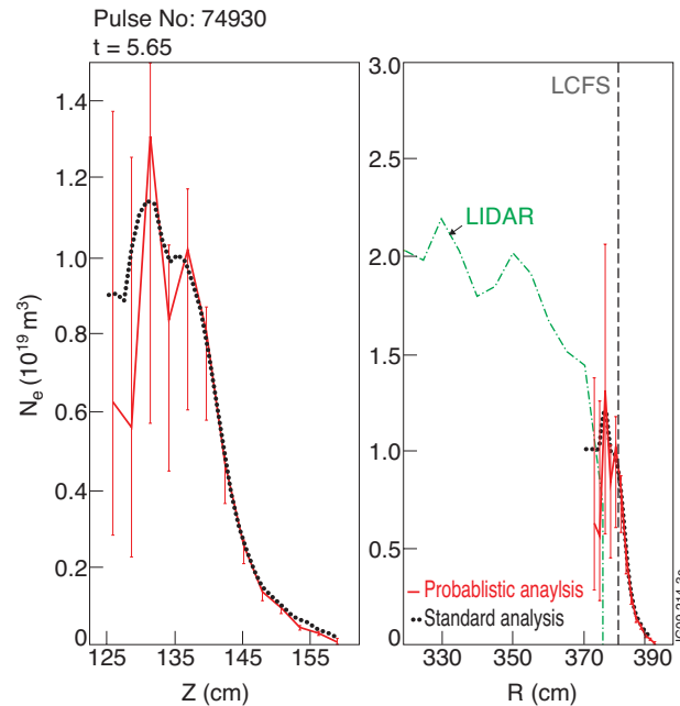
Figure 3: Reconstructed electron density profiles in the early phase of Pulse No: 74930 ( t=5.65 ). The result of the standard lithium beam analysis is shown in black, while the red curve with error bars shows the result of the probabilistic analysis. The right part of the plot shows the profiles mapped onto the midplane together with the result of the LIDAR measurement (green curve).
