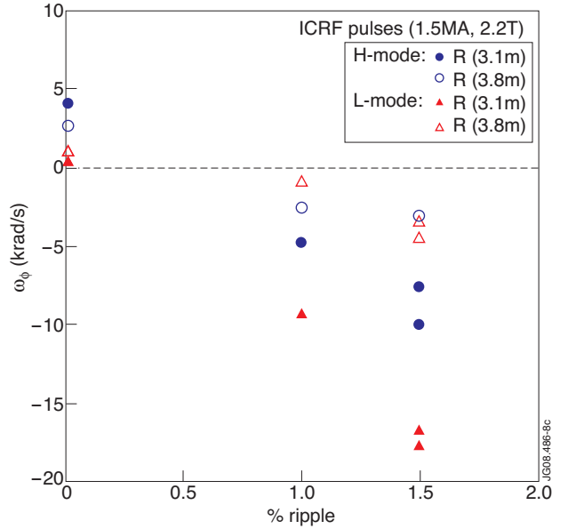
Figure 4: Toroidal rotation as a function of ripple for ICRF pulses with 1.5MA, off-axis R_{res}=2.71\text{m} , for the centre ( 3.1\text{m} , solid symbols) and the edge ( R=3.8\text{m} , open symbols). Blue circles are measurements in H-mode and red triangles are Lmode.
