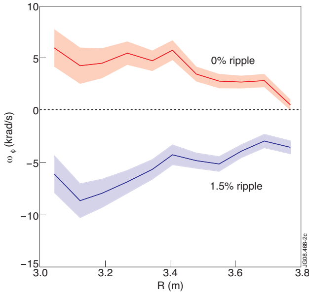
Figure 3: Toroidal rotation profiles from charge exchange measurements for ICRF heated pulses with I_p=1.5\text{MA} and \langle B_T \rangle=2.2\text{ T} , P_{ICRF} \sim 3\text{ MW} for two ripple levels. Top: Pulse No: 74688 with 0% ripple and P_{ICRF}=3.1\text{MW} ; bottom: Pulse No: 74686 with P_{ICRF}=2.9\text{MW} bottom). R_0=3.02\text{m} , the ICRF resonance is off-axis on the high-field side at R_{res}=2.71\text{m} .
