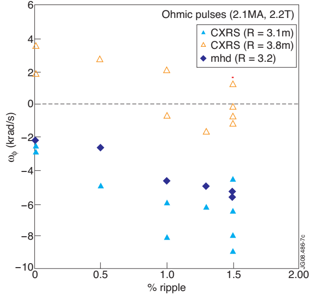
Figure 2: Toroidal rotation frequencies as a function of ripple for Ohmic pulses with 2.1MA. Plot shows: the charge exchange toroidal rotation frequency at the centre ( R=3.1\text{m} , blue triangles) and the edge ( R=3.8\text{m} , red triangles) and the frequency of sawtooth postcursors (solid blue kites). The sawtooth inversion radius and period remained unchanged with ripple.
