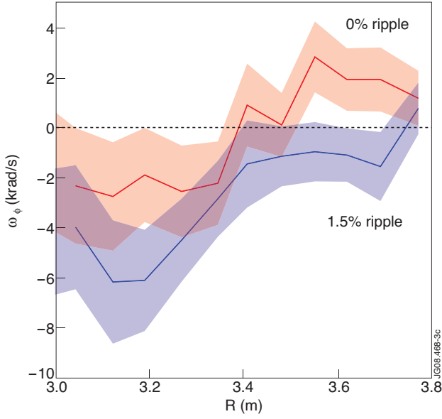
Figure 1: Toroidal rotation profiles from charge exchange measurements for Ohmic Pulse No's: 74758 with 0% ripple and 74599 with 1.5% ripple, I_p=2.1\text{MA} and \langle B_T \rangle=2.2\text{ T} . Here and in the following figures, the profiles shown are the average over the first 20ms. Error-bars are indicated by the shaded areas.
