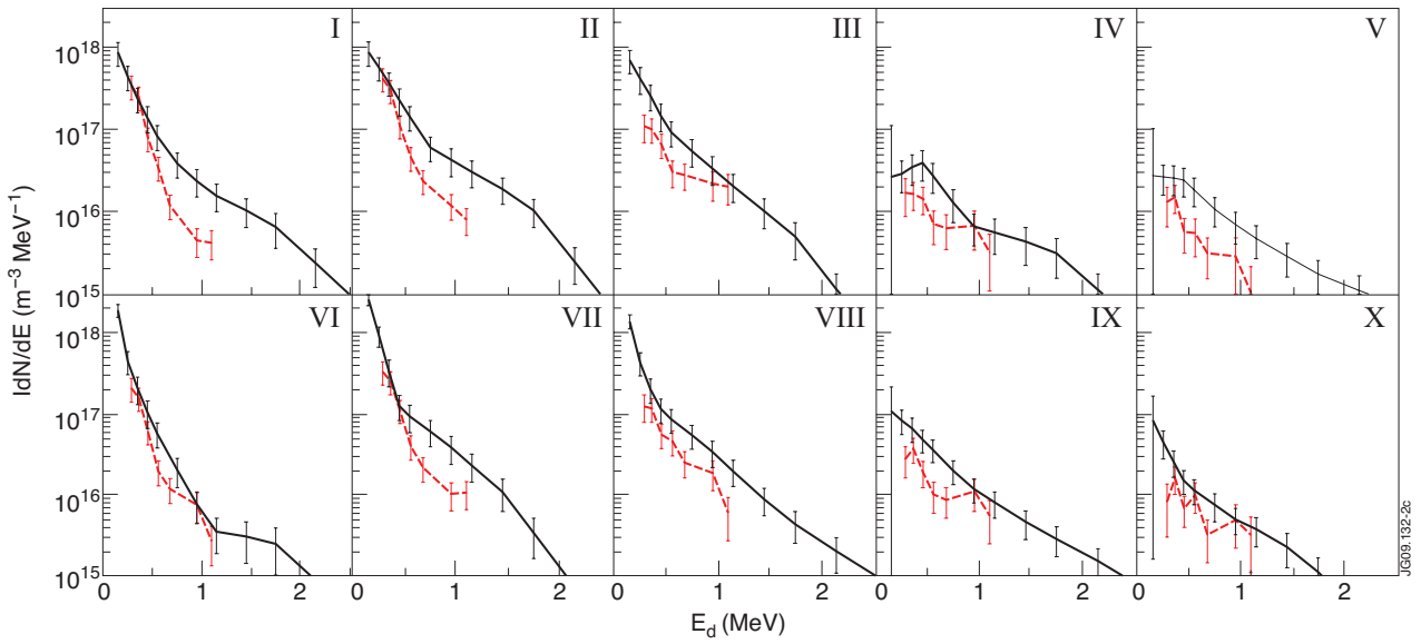
Figure 2: Deuteron energy distributions derived from measured TOFOR (black) and KF1 (red) data using the modeling described in the text, for time period I-X of JET Pulse No: 69247 indicated in figure 1.
